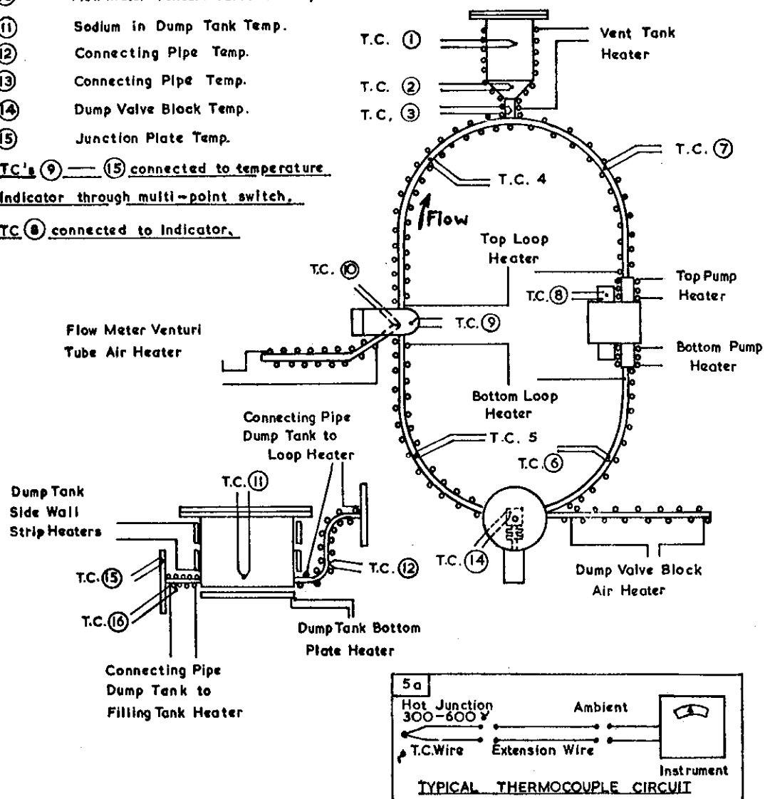
FIG.5 HEATERS AND THERMOCOUPLE LOCATION DETAILS.
