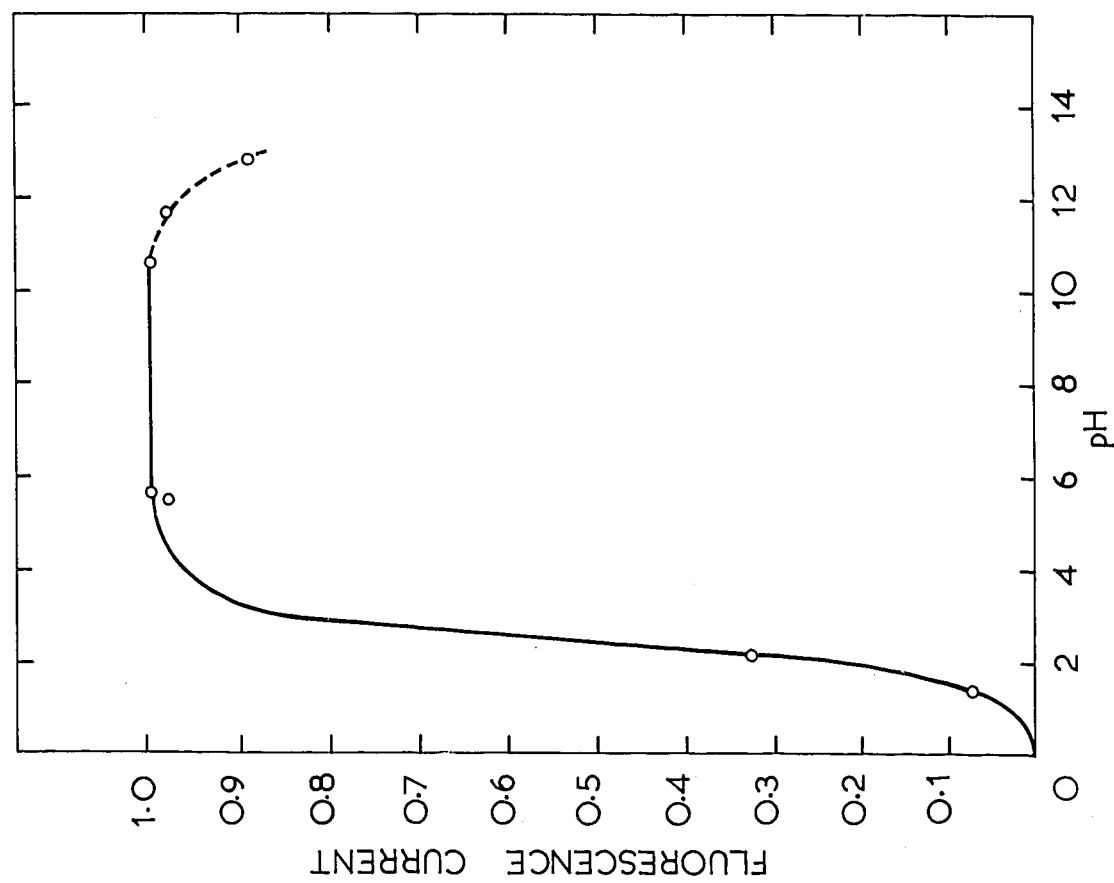
FIGURE 1. FLUORESCENCE-INDUCED PHOTOCURRENT OF IRRADIATED SODIUM TEREPHTHALATE SOLUTION vs. pH
