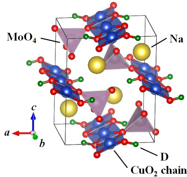
Figure 1. Crystal structure of NaCuMoO 4 (OD). The positions of the D ions are determined by this study. VESTA software [9] is used for drawing crystal structure.
