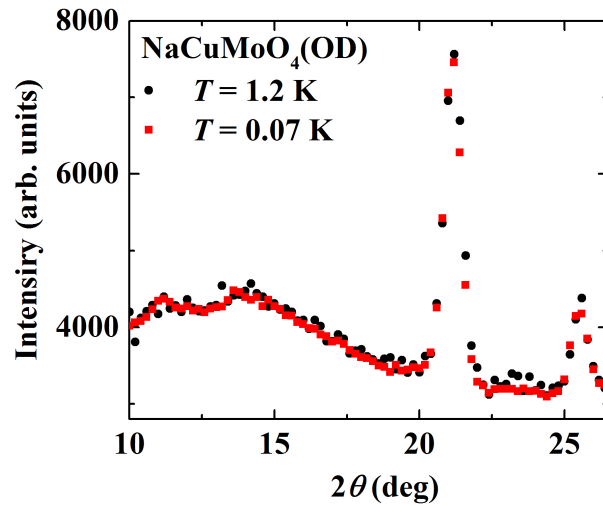
Figure 2. Powder neutron diffraction patterns at T = 0.07 and 1.2 K. Data are vertically scaled.
