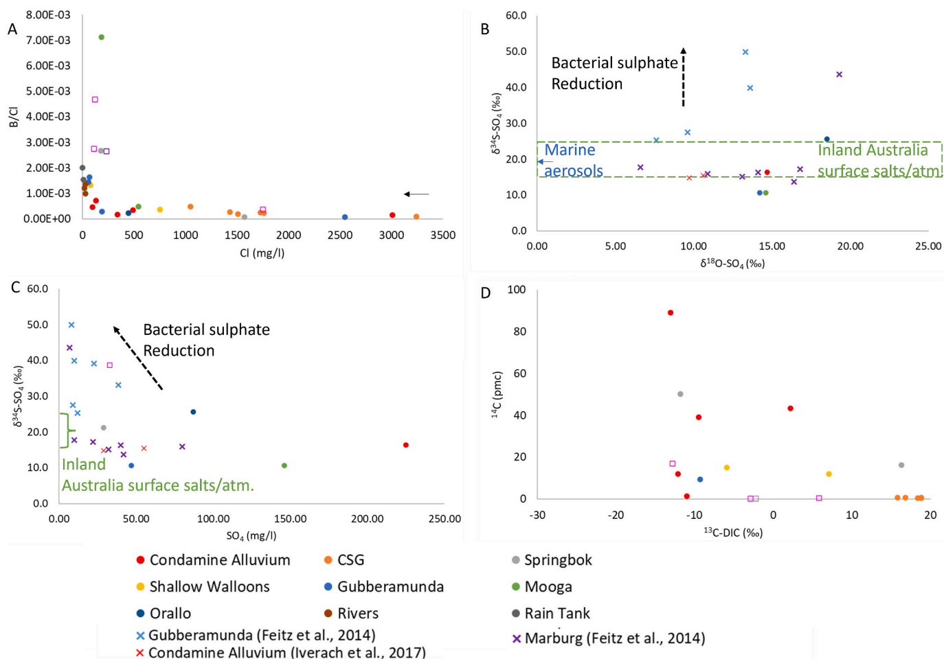
Fig. 7. A) B/Cl vs Cl concentration. The arrow indicates the equivalent seawater value. B) The \delta^{34}\text{S-SO}_4 vs \delta^{18}\text{O-SO}_4 with general region associated with surface salts in Inland Australia in recharge waters. C) The \delta^{34}\text{S-SO}_4 vs \text{SO}_4 concentration. The reported value for surface salts in inland Australia is shown. Existing data for groundwaters from deeper Gubberamunda bores are also shown (crosses), along with those for Marburg Sandstone bores that are the equivalent of the Hutton Sandstone in the Clarence-Moreton Basin from (Feitz et al., 2014), and the Condamine Alluvium from (Iverach et al., 2017). Sulphide was below detection in the existing data. D) The ^{14}\text{C} of sampled waters vs \delta^{13}\text{C-DIC} .
