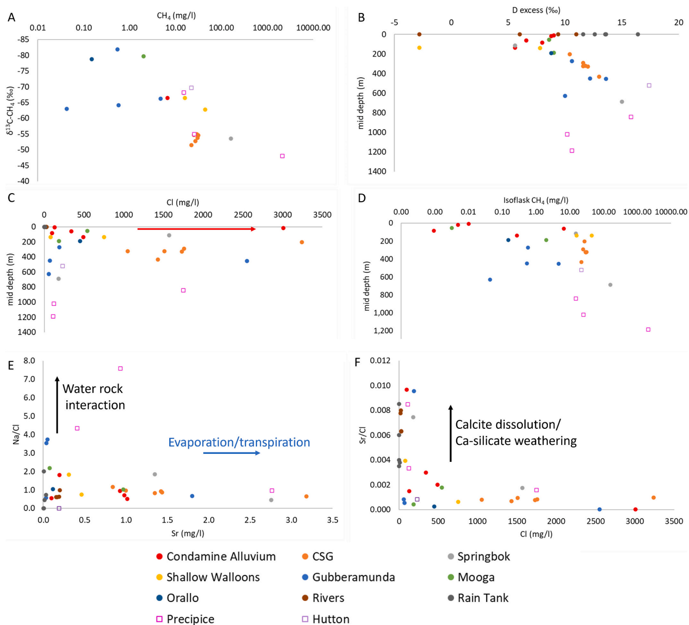
Fig. 3. A) Dissolved methane vs ^{13}\text{C}\text{-CH}_4 . B) The \delta^2\text{H}\text{-H}_2\text{O} or “D” excess vs depth. C) Concentration of Cl with bore screen sample depth below surface. The red arrow indicates the effect of (evapo)transpiration that has likely increased Cl in one Condamine Alluvium sample. D) Dissolved methane concentration (log scale, measured from Isoflask containers) with depth. E) Na/Cl vs Sr concentration. F) Sr/Cl vs Cl concentration. (For interpretation of the references to colour in this figure legend, the reader is referred to the web version of this article.)
