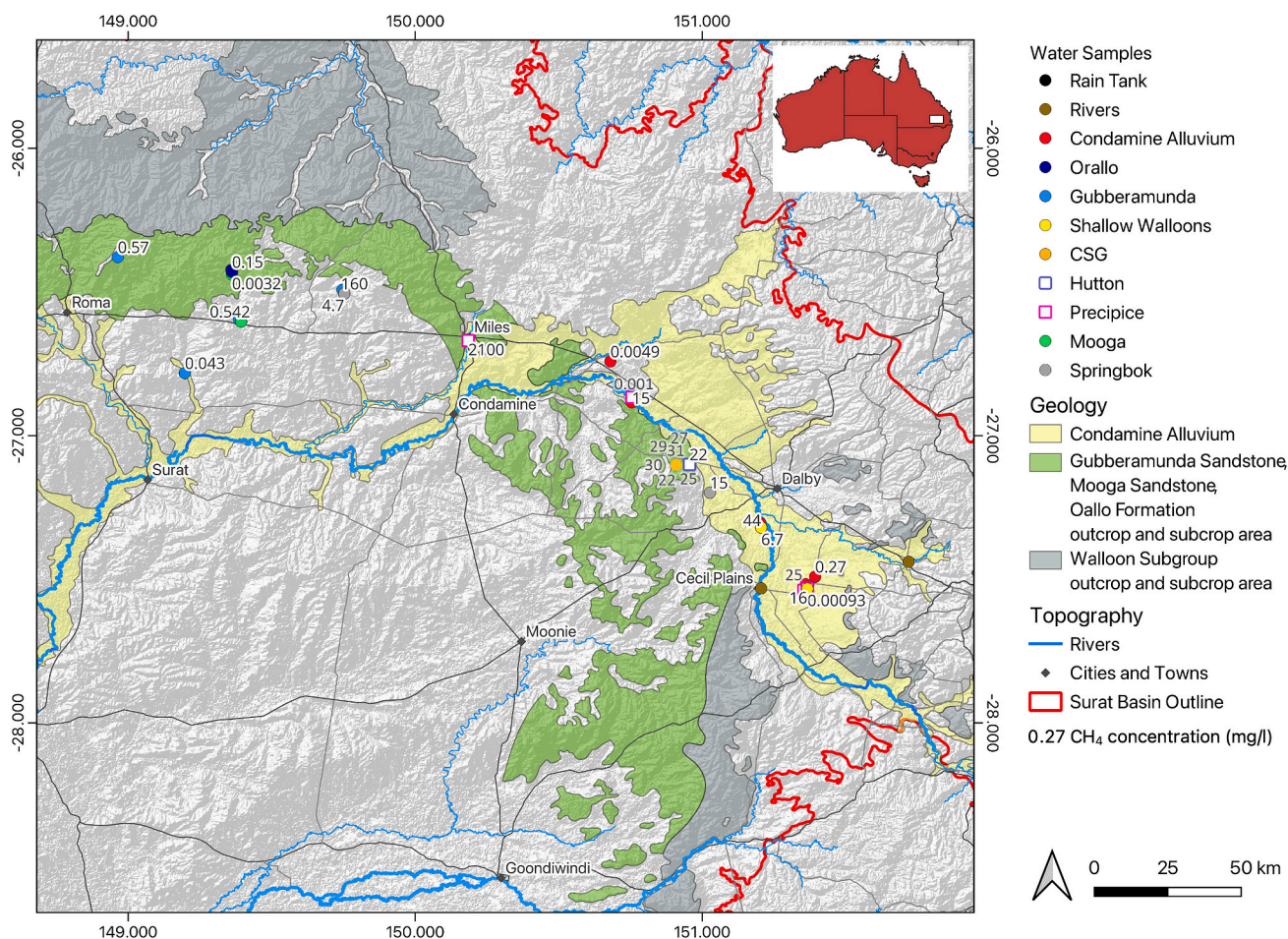
Fig. 2. Dissolved methane concentrations (mg/L) on an overview map of bores, CSG wells, and river sample positions. Note that several water bores were in close proximity to each other or nested. Full data are given in supplementary material. Inset is the study site position relative to Australia.
