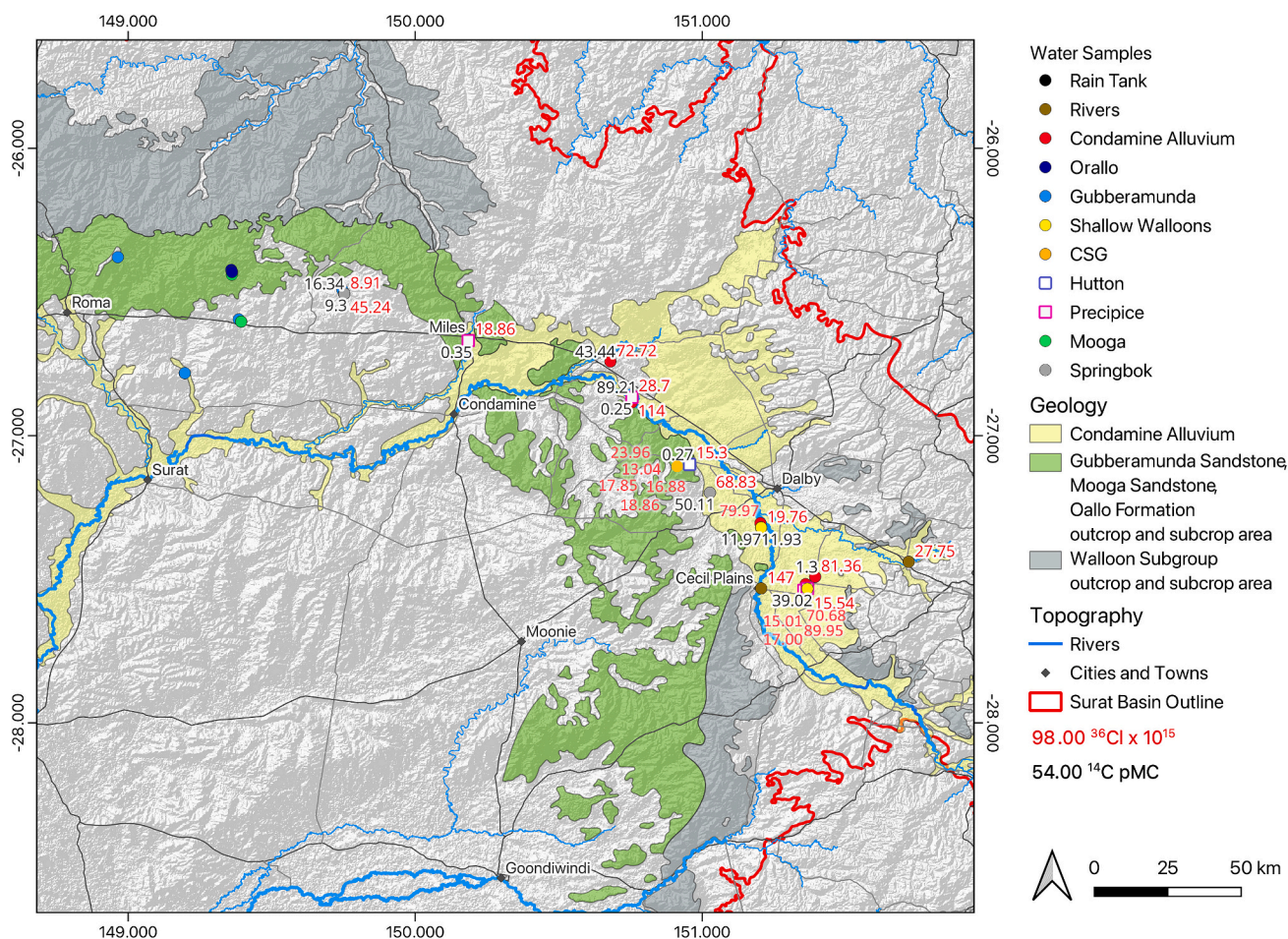
Fig. 8. Map showing the groundwater, CSG production water and river water ^{36}\text{Cl}/\text{Cl} ( \times 10^{15} ) (labelled in red), and ^{14}\text{C} (pMC) labelled in black. Many bores were nested or in close proximity. Full data, including rainwater, are given in the supplementary material. (For interpretation of the references to colour in this figure legend, the reader is referred to the web version of this article.)
