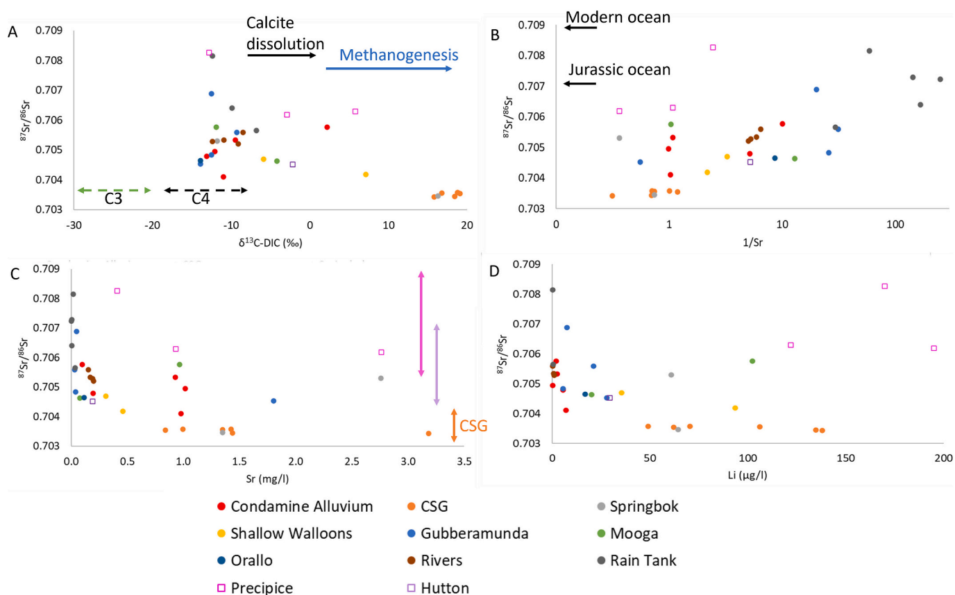
Fig. 5. A) The ^{87}\text{Sr}/^{86}\text{Sr} signatures of bore groundwaters, CSG production waters, rivers and rain waters vs \delta^{13}\text{C-DIC} . The dashed arrows indicate general input \delta^{13}\text{C-DIC} ranges to soil carbon from C3 and C4 plants. Calcite dissolution and methanogenesis elevate \delta^{13}\text{C-DIC} . B) The ^{87}\text{Sr}/^{86}\text{Sr} signatures vs 1/\text{Sr} concentration (on a log scale to view the rainwaters), the isotope signatures of the Jurassic and modern ocean are also indicated. C) ^{87}\text{Sr}/^{86}\text{Sr} vs Sr concentration, the orange arrow indicates the ^{87}\text{Sr}/^{86}\text{Sr} isotope range of Walloon Coal Measures CSG production water previously published (Baublys et al., 2019). The pink and purple arrows indicate ^{87}\text{Sr}/^{86}\text{Sr} isotope ranges of Precipice and Hutton aquifer samples respectively across the southern Surat Basin from (Hofmann et al., 2021) and also from (Hofmann et al., 2024) note these arrows do not indicate the Sr concentration ranges. D) ^{87}\text{Sr}/^{86}\text{Sr} vs Li concentration. (For interpretation of the references to colour in this figure legend, the reader is referred to the web version of this article.)
