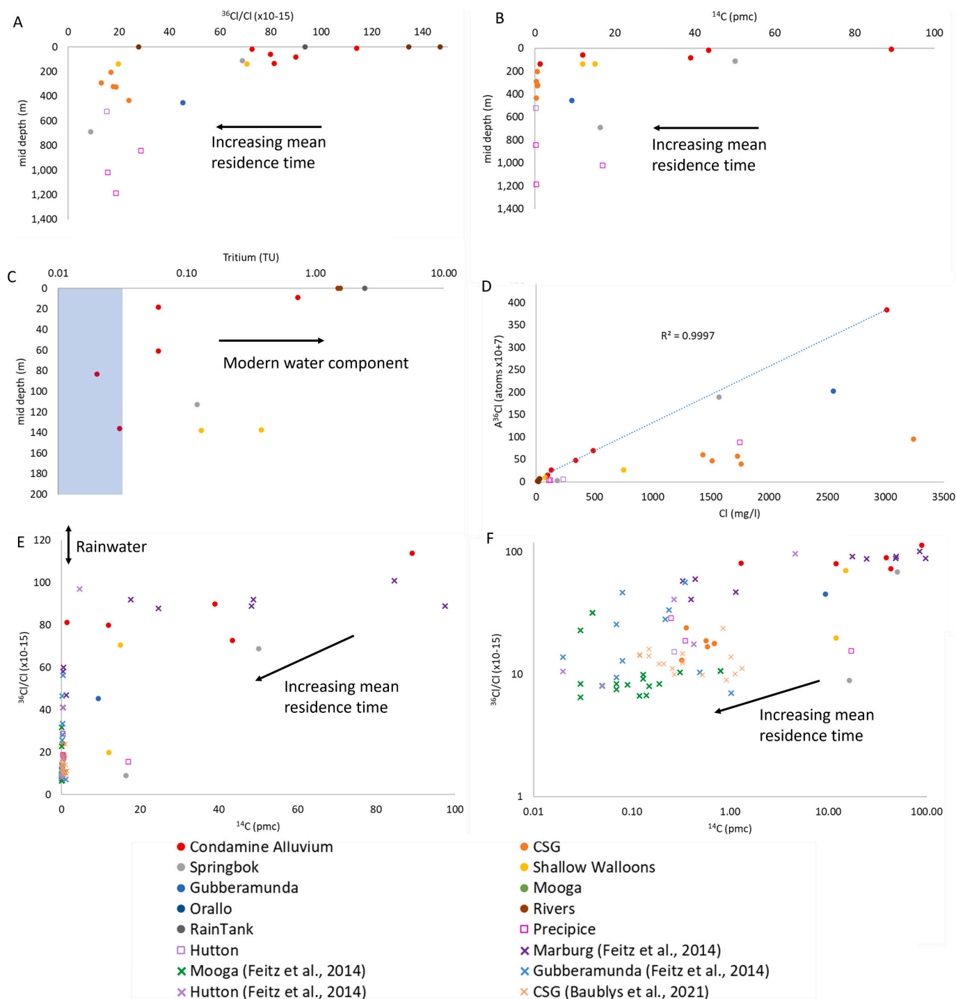
Fig. 10. A) The groundwater, produced water, rain and river water ^{36}\text{Cl}/\text{Cl} with mid screen sample depth. The more depleted river sample is Oakey Creek, the two more enriched river samples are Condamine River. B) The ^{14}\text{C} of groundwater and produced waters vs sample depth. C) Tritium of groundwaters, Condamine River samples and rain water vs sample depth (note the smaller depth scale compared to A) and B) for these shallow samples). The blue box indicates the limit of meaningful detection of tritium D) The A^{36}\text{Cl} vs Cl concentrations of waters. The correlation of Condamine Alluvium groundwaters is shown. E) The groundwater and produced water ^{36}\text{Cl}/\text{Cl} vs ^{14}\text{C} with existing data shown as crosses from (Baublys et al., 2021; Feitz et al., 2014). The rainwater range is from two reported Roma and Chinchilla rain samples (Baublys et al., 2021). F) The groundwater and produced water ^{36}\text{Cl}/\text{Cl} vs ^{14}\text{C} values shown on a log scale. (For interpretation of the references to colour in this figure legend, the reader is referred to the web version of this article.)
