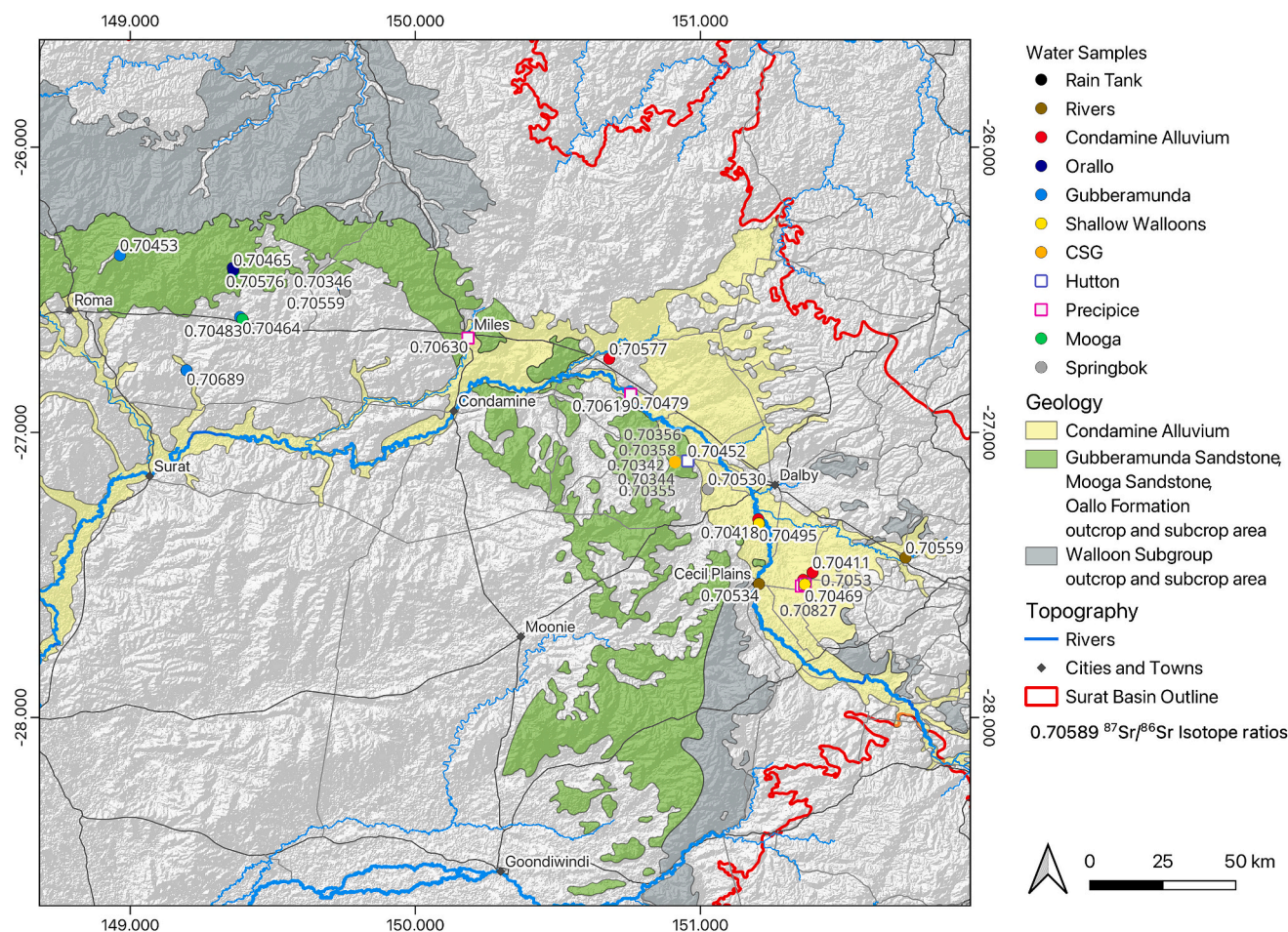
Fig. 4. Map showing the ^{87}\text{Sr}/^{86}\text{Sr} isotope ratios of bore groundwaters, CSG production waters, and river waters. Note many bores are nested, and one Condamine River sample is off the range of this map, see supplementary material. All data including rainwaters and positions are in the supplementary material.
