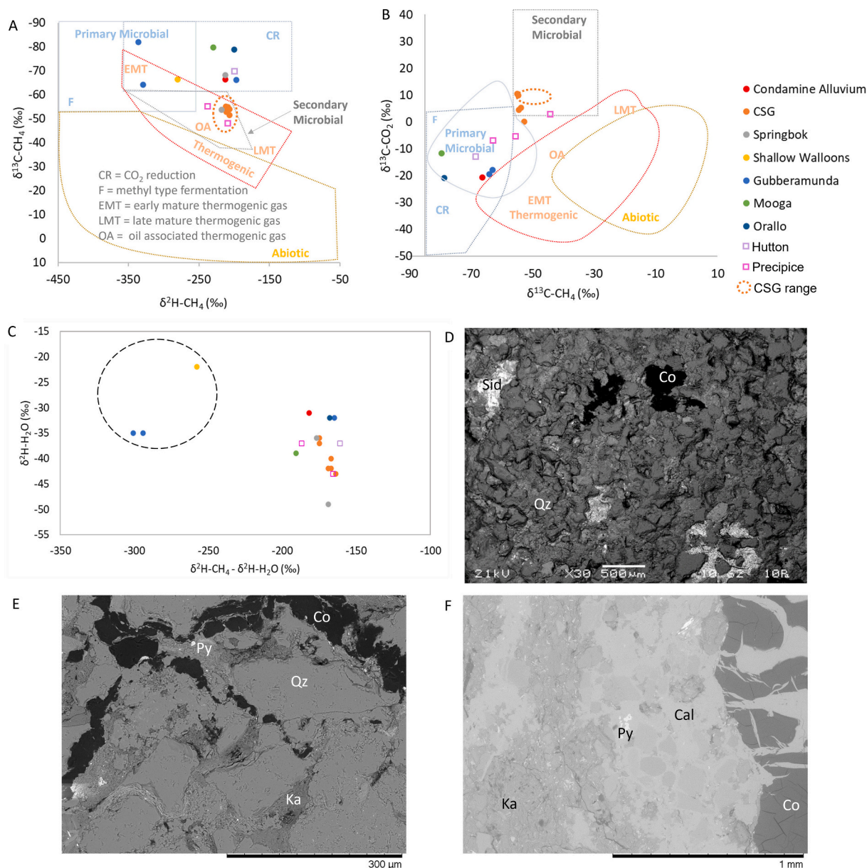
Fig. A1. A) The \delta^{13}\text{C-CH}_4 vs \delta^2\text{H-CH}_4 for the groundwater and CSG production waters. B) The \delta^{13}\text{C-CO}_2 vs \delta^{13}\text{C-CH}_4 modified after (Pearce et al., 2022a). The regions are shown from (Milkov and Etiope, 2018). The CSG range orange dashed circle is existing data across the Surat Basin from (Baublys et al., 2015). C) The \delta^2\text{H-H}_2\text{O} vs \delta^2\text{H-CH}_4 - \delta^2\text{H-H}_2\text{O} where two Gubberamunda samples and a Shallow Walloons bore sample with lower \delta^2\text{H-CH}_4 - \delta^2\text{H-H}_2\text{O} , circled, are consistent with acetate fermentation, and the others with \text{CO}_2 reduction pathways producing methane. D) Example of coal in the Hutton Sandstone, scanning electron microscope (SEM) image. E) SEM of coal in the upper Precipice Sandstone. F) SEM of coal and calcite cements in the Springbok Sandstone. Co = coal, Qz = quartz, Sid = siderite, Py = pyrite, Ka = kaolinite, Cal = calcite.
