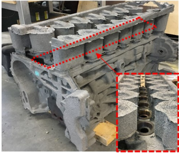
As-Cast with Fe Chills (TSR + Chills)
