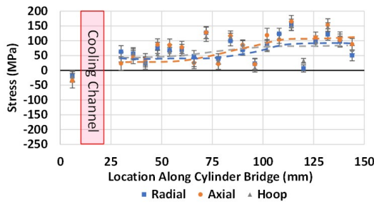
Stress - T4 (Edge Bridge)
