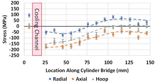
Stress - TSR (Edge Bridge)
