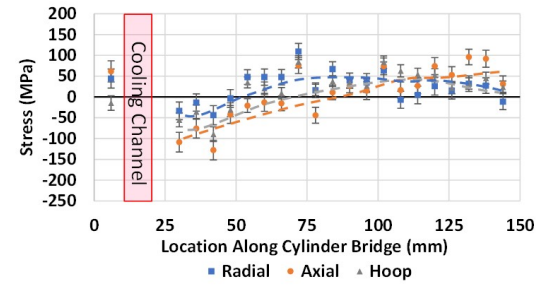
Stress - T7 (Edge Bridge)
