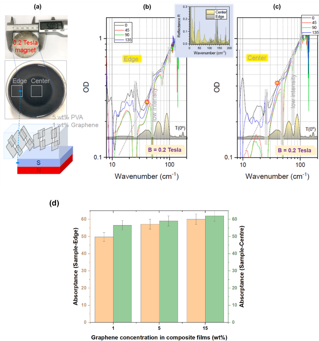
Fig. 12. (a) PVA-Graphene composite (5 wt%-1wt%) made on B = 0.2 T magnet. Absorbance spectra OD ( \nu ) from the sample edge (b) and sample center (c) regions at different polarisations \theta . The inset shows reflectivity spectra at \theta = 0^\circ . The star-markers are at \tilde{\nu} = 40 \text{ cm}^{-1} .
