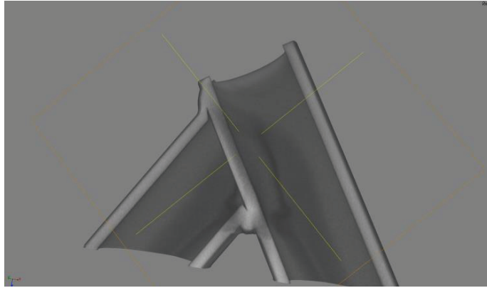
Figure 2 cut through 3D model from reconstructed neutron tomography of welded tubes
