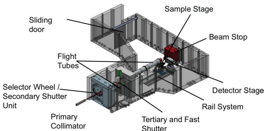
Figure 1 DINGO instrument assembly
