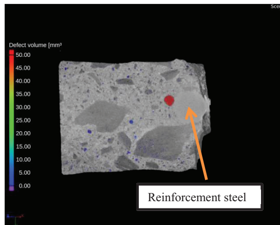
Figure 3 porosity analysis of a concrete sample with reinforcement steel
