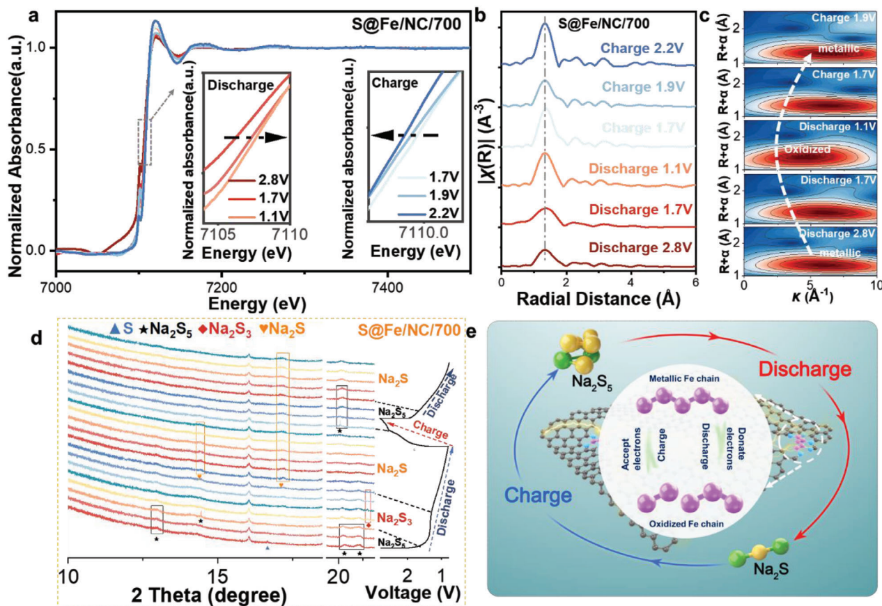
Figure 5. a) Ex situ Fe K-edge XANES spectra of the S@Fe/NC/700 sample during the first discharge and charge processes, with the insets enlargements of the white-line shifts. b) The corresponding ex situ Fe K-edge EXAFS spectra and c) WT plots of the S@Fe/NC/700 sample by using k^3 space. d) In situ high-energy X-ray diffraction (XRD) patterns of S@Fe/NC/700. e) Mechanism diagram for S@Fe/NC/700 during charging and discharging processes.
