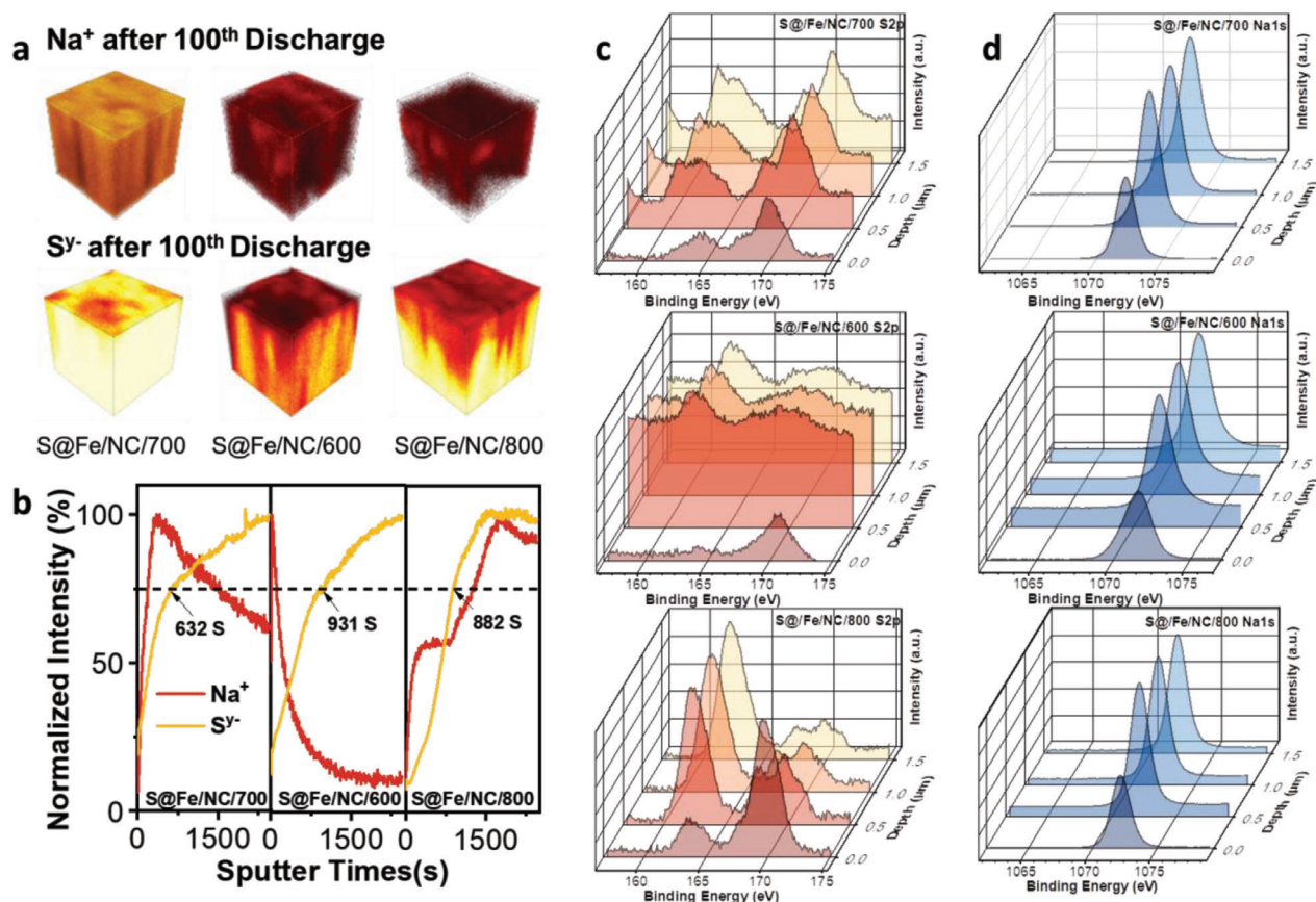
Figure 6. a) 3D reconstructed images of TOF-SIMS depth profiles of \text{Na}^+ and \text{S}^{2-} after the 100th cycle. b) Normalized depth profiles of secondary ion fragments obtained from the S@Fe/NC/600, S@Fe/NC/700, and S@Fe/NC/800 cathodes after the 100th cycle, respectively. Depth profile spectra of S 2p (c) and Na 1s (d) for S@Fe/NC/600, S@Fe/NC/700, and S@Fe/NC/800, respectively.
