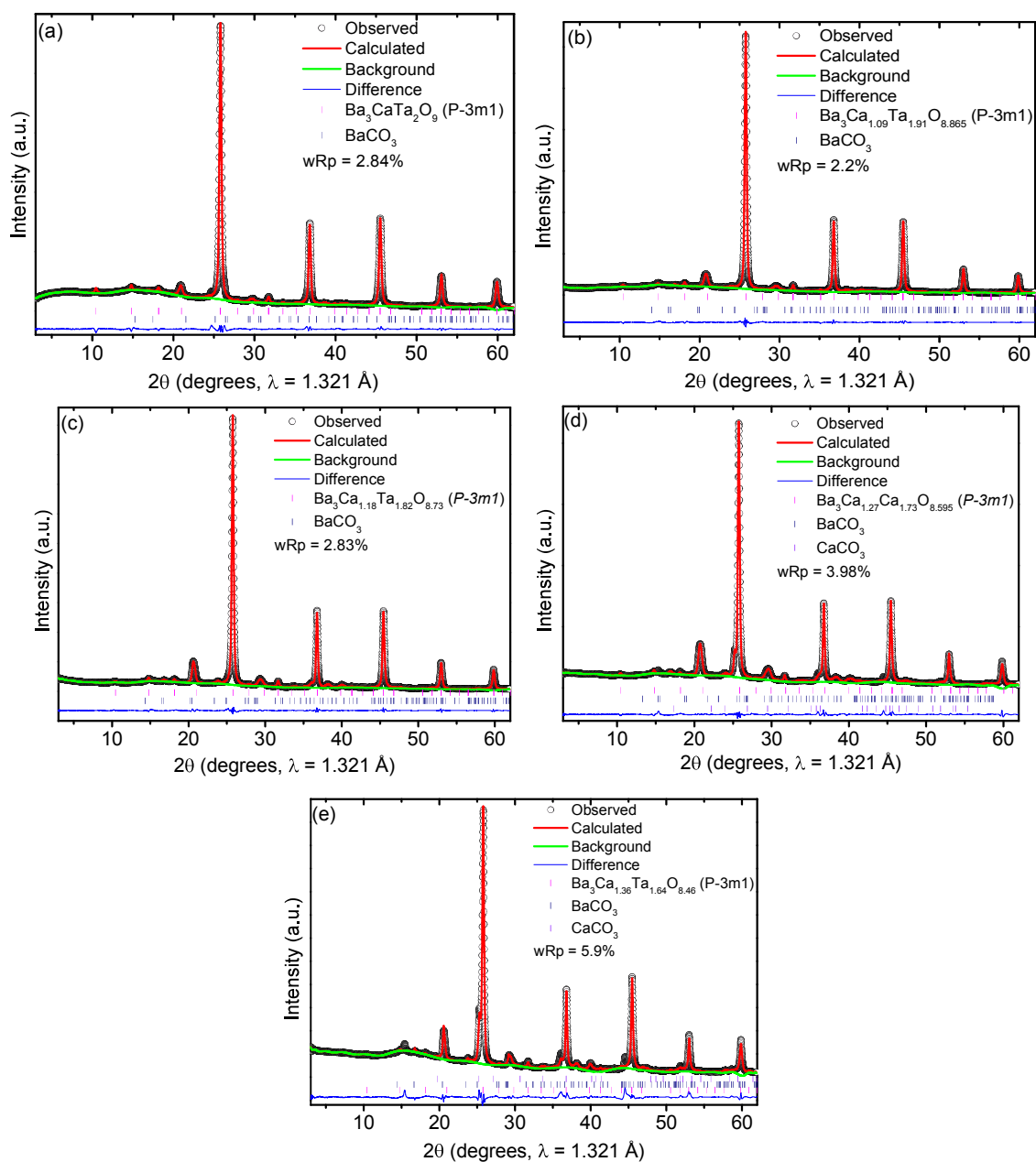
Figure 3. Rietveld refinement of monochromatic synchrotron X-ray diffraction data for \text{Ba}_3\text{Ca}_{1+x}\text{Ta}_{2-x}\text{O}_{9-3x/2} ( 0 \leq x \leq 0.36 ). The samples were prepared at 1000^\circ\text{C} , (a-e).
