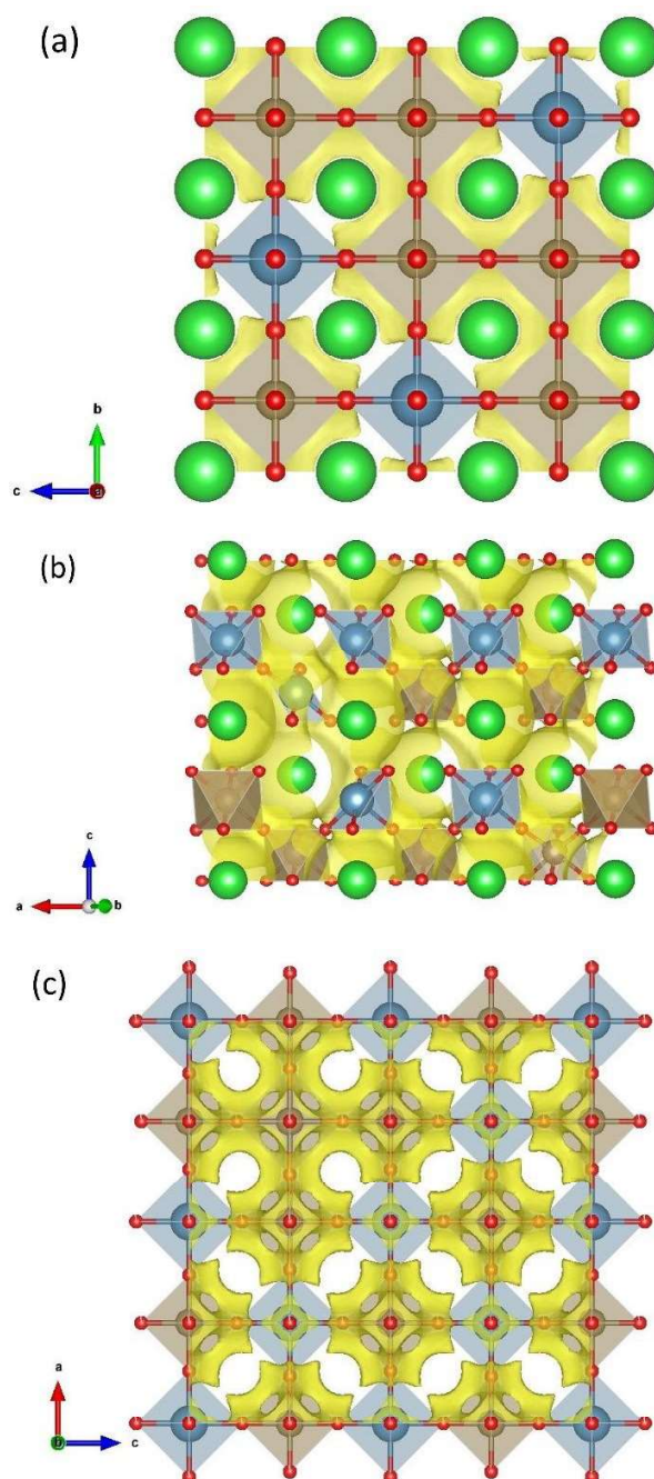
Figure 7. The bond valence energy landscape (BVEL) calculations for O^{2-} ions in the supercells generated from a) Pm-3m , b) P-3m1 and c) Fm-3m as the input files. In (a), the projection of (100) plane was selected at x values between 0.25 and 0.5. In (b), the projection of (010) was selected at y values between 0.25 and 0.5. In (c), the projection of (010) was selected at y values between 0.2 and 0.35. Ba, Ca, Ta and O are represented by green, blue, brown and red spheres.
