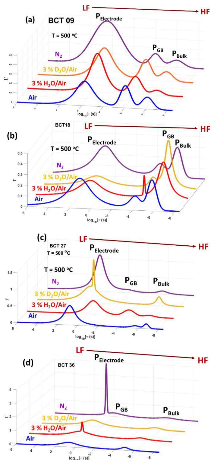
Figure 9. DFRT plots of (a) \text{Ba}_3\text{Ca}_{1.91}\text{Ta}_{0.09}\text{O}_{9-3x/2} (BCT09), (b) \text{Ba}_3\text{Ca}_{1.18}\text{Ta}_{1.82}\text{O}_{9-3x/2} (BCT18), (c) \text{Ba}_3\text{Ca}_{1.27}\text{Ta}_{1.73}\text{O}_{9-3x/2} (BCT27), and (d) \text{Ba}_3\text{Ca}_{1.36}\text{Ta}_{1.64}\text{O}_{9-3x/2} (BCT36) at 500 °C showing presence of three peaks due to bulk, grain-boundary (GB), and electrode transport processes.
