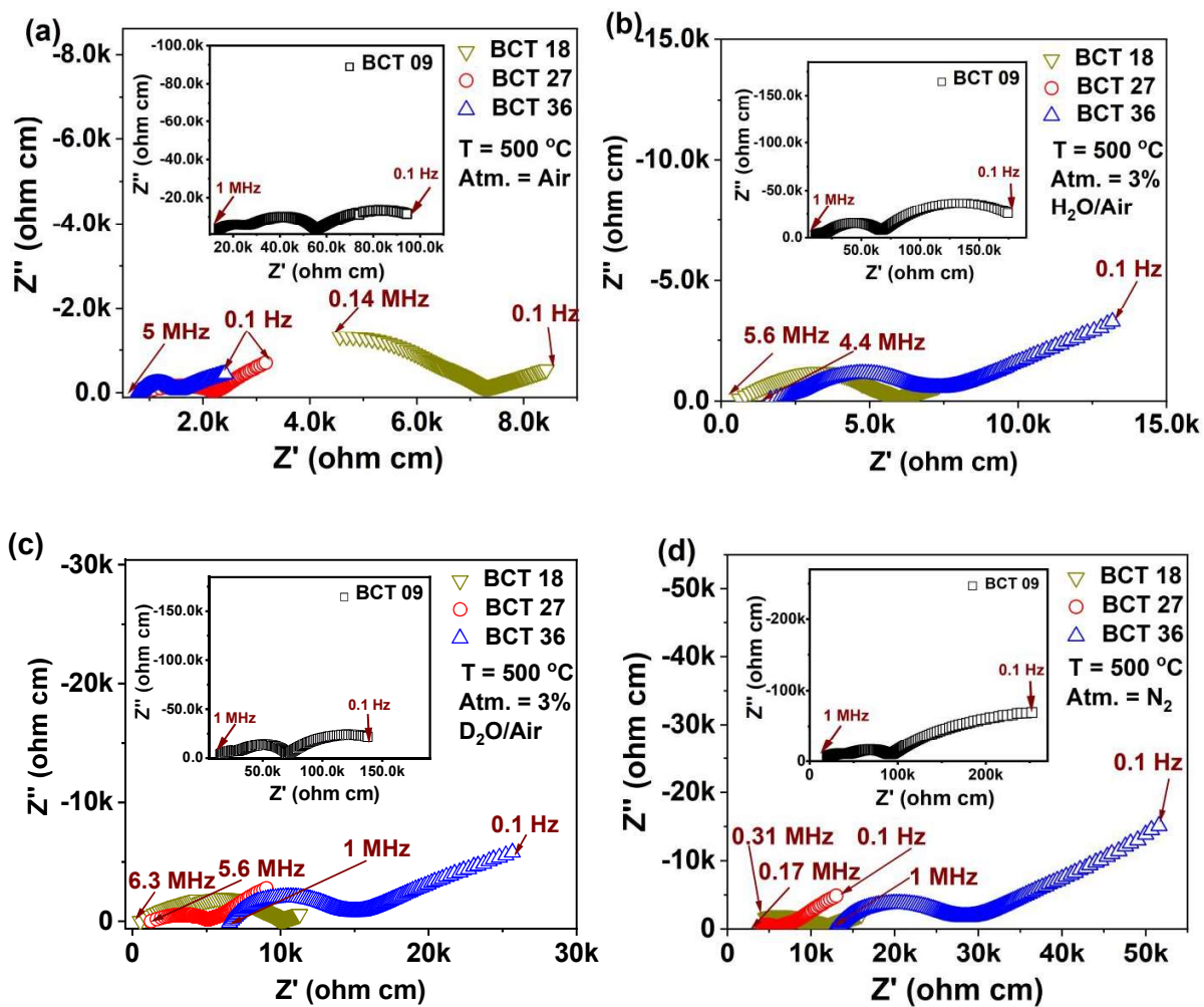
Figure 8. Nyquist plots at temperature 500 °C for Ba 3 Ca 1.09 Ta 1.91 O 8.865 (BCT09), Ba 3 Ca 1.18 Ta 1.82 O 8.73 (BCT18), Ba 3 Ca 1.27 Ta 1.73 O 8.595 (BCT27), and Ba 3 Ca 1.36 Ta 1.64 O 8.46 (BCT36) in (a) air, (b) 3%H 2 O/air, (c) 3% D 2 O/air, and (d) N 2 .
