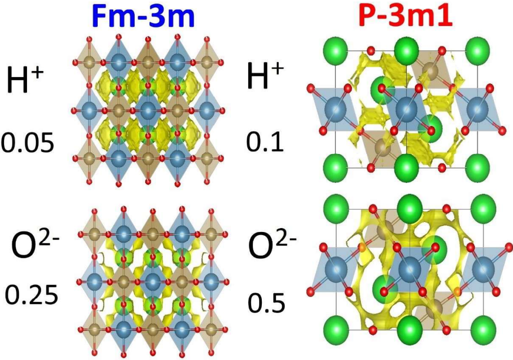
Figure 6. The bond valence sum (BVS) mismatch map calculation on Fm-3m and P-3m1 space groups for H^+ , and O^{2-} mobile ions on the projection of (110) plane.
