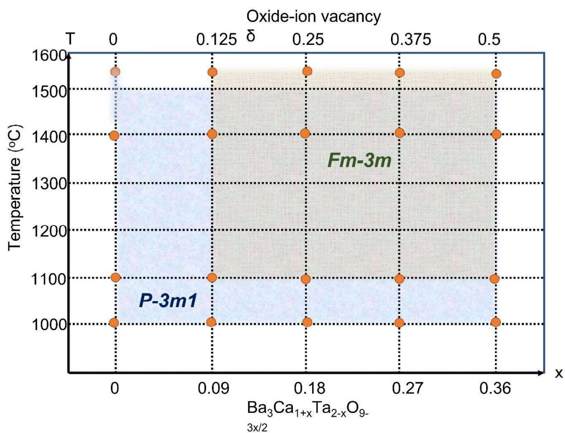
Figure 1. Functional phase diagram of \text{Ba}_3\text{Ca}_{1+x}\text{Ta}_{2-x}\text{O}_{9-3x/2} ( 0 \leq x \leq 0.36 ) as a function of temperature and off-stoichiometry. The orange spots represent the exact experimental conditions being investigated in the current study.
