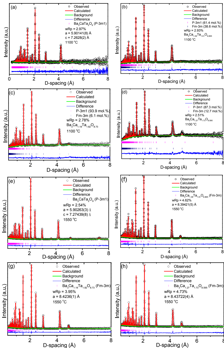
Figure 2. Rietveld refinement of TOF-Neutron diffraction data for \text{Ba}_3\text{Ca}_{1+x}\text{Ta}_{2-x}\text{O}_{9-3x/2} ( 0 \leq x \leq 0.27 ). The samples were prepared at 1100 °C, (a-d) and 1550 °C (e-f).
