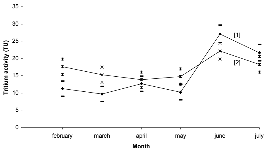
Fig. 1 Tritium concentration variation in precipitation over 2001 year measured by [1] ISO method and [2] APHA-AWA-WEF method (monthly sampling and reported uncertainty \pm 1 \square ).
