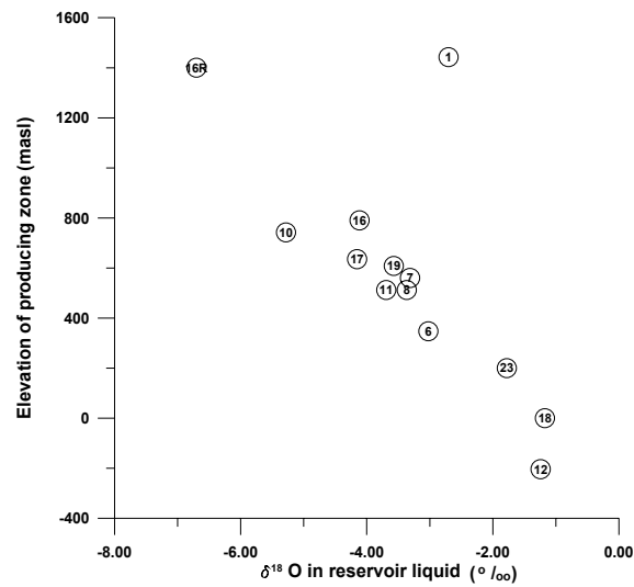
FIG. 1 Elevation of production zones of wells vs \delta^{18}O in reservoir liquid.
