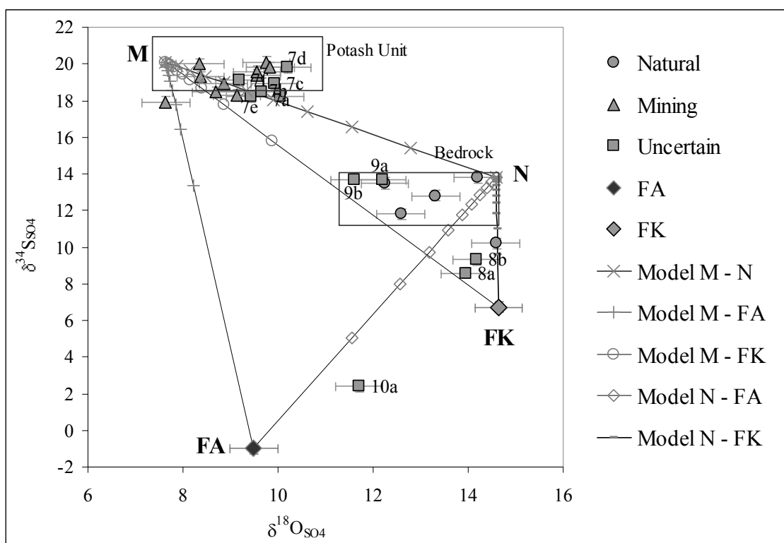
FIG. 1 Plot of \delta^{18}\text{O}_{\text{SO}_4} vs \delta^{34}\text{S}_{\text{SO}_4} . Symbols represent sample values; boxes show bedrock evaporites and Potash Unit ranges. Lines are mix models between the end members considered: M =mine effluents ( \delta^{34}\text{S} = +20\text{‰} , \delta^{18}\text{O} = +7.6\text{‰} ), N = natural springs ( \delta^{34}\text{S} = +13.8\text{‰} , \delta^{18}\text{O} = +14.6\text{‰} ), FK = NPK fertiliser ( \delta^{34}\text{S} = +8\text{‰} , \delta^{18}\text{O} = +15\text{‰} ) and FA =ammonium fertiliser ( \delta^{34}\text{S} = -1\text{‰} , \delta^{18}\text{O} = +9.5\text{‰} ).
