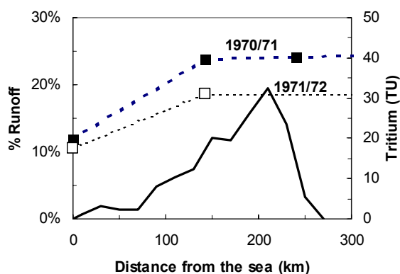
FIG. 3. Distribution of runoff generating areas (solid line) and of rainfall tritium content as function of distance from the sea. The dashed lines indicate the tritium rainfall models utilised for the two seasons.
