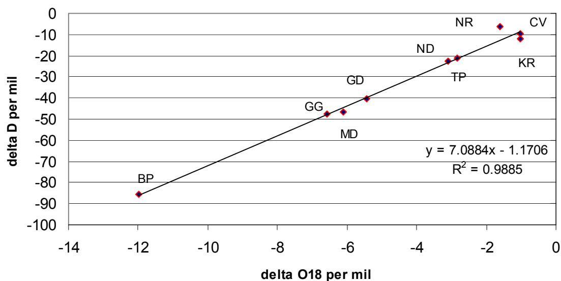
FIG. 1. Relation between \delta^{18}\text{O} and \delta^2\text{H} for the June 2002 sampling of the Indian rivers. (Brahmaputra: BP, Ganga: GG, Mahanadi: MD, Godavari: GD, Krishna: KR, Kaveri: C, Nethvarti: NR, Tapi: TP and Narmada: ND).
