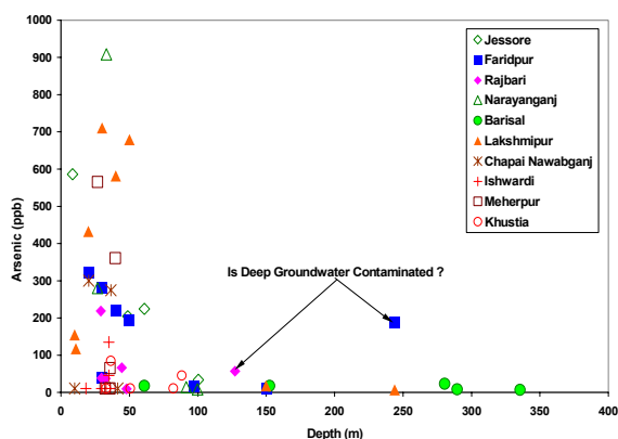
Fig. 1. Arsenic concentrations in groundwater
