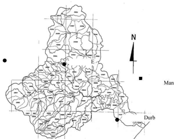
FIG. 2. The Tugela catchment showing the runoff sampling site (Mandini) and three rainwater sampling sites (Durban, Estcourt and Oxbow).
