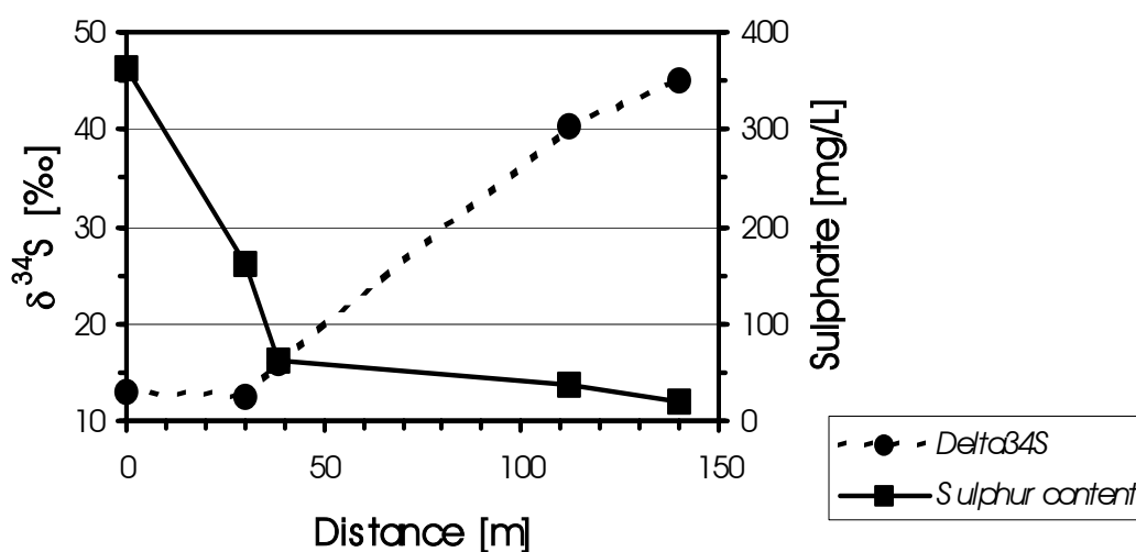
FIG. 3. Sulphate content and its \delta^{34}\text{S} along a flow path in BTEX contaminated aquifer I.
