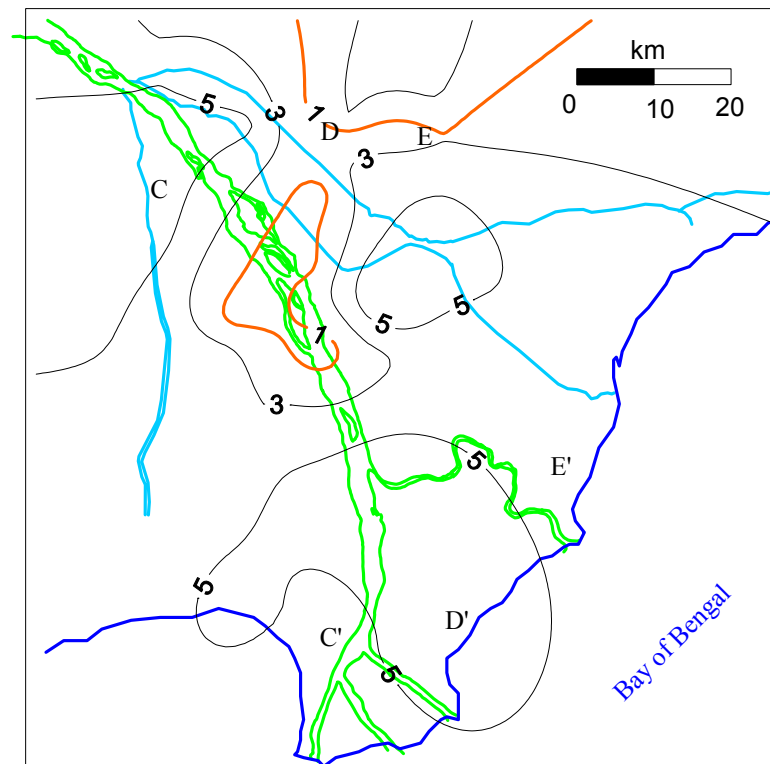
Fig. 2. Distribution of Environmental tritium concentration in the shallow groundwater (<30m bgl) in the Krishna delta region (India)
