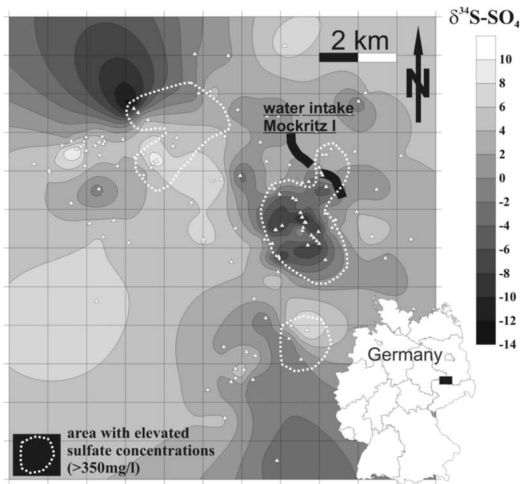
FIG. 4. Regional distribution of \delta^{34}\text{S} at the groundwater surface in the catchment area of Torgau-Mockritz
