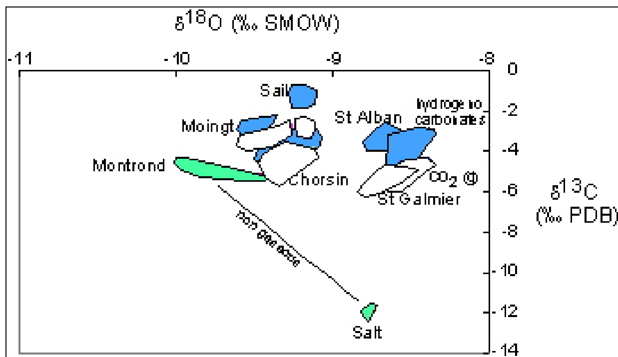
Fig. 1: C and O isotope ratios of \text{CO}_2 -rich waters (white domain: water with gas ; blue domain: degassed water) showing two groups: one ( \delta^{18}\text{O} > -9\text{‰} ) including waters in granite domain, the other ( \delta^{18}\text{O} < -9\text{‰} ) comprising waters flowing at the limits of the Forez sedimentary basin. Thermal waters are in green.
