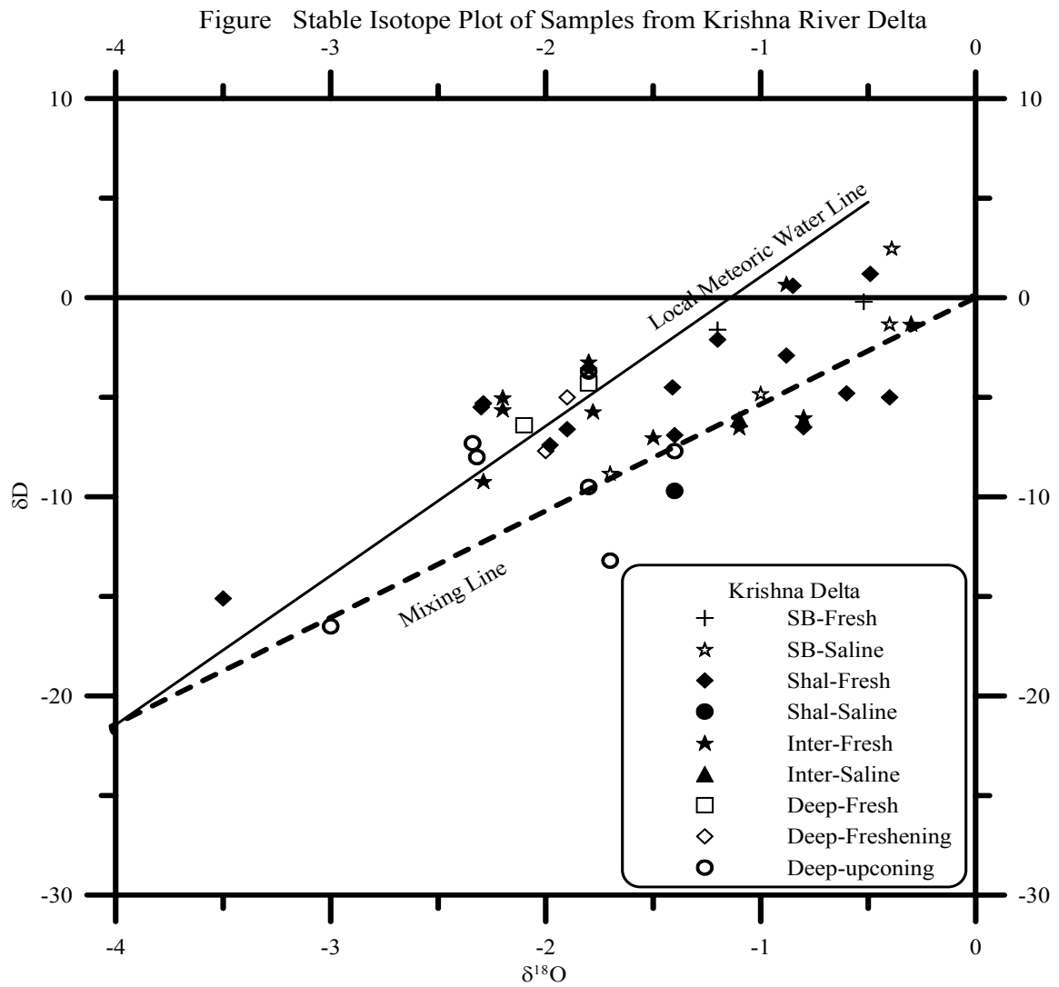
Figure 1. \delta\text{D} - \delta^{18}\text{O} plot of the data pertaining to the groundwater samples from the Krishna river delta region. The mixing trend as depicted by the mixing line is distinct from the local meteoric water line
