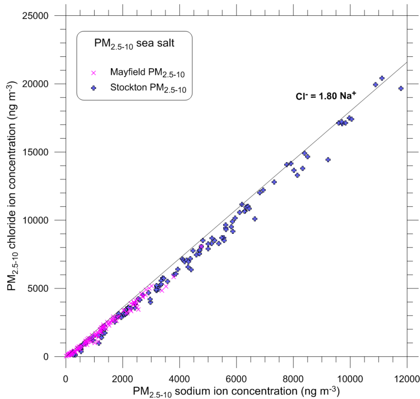
Figure 47: Scatter plot for PM 2.5-10 showing that, unlike for PM 2.5 , there is a strong correlation between chloride and sodium concentration with the ratio ( \text{Cl}^-/\text{Na}^+ = 1.80 ) matching that for fresh sea salt
