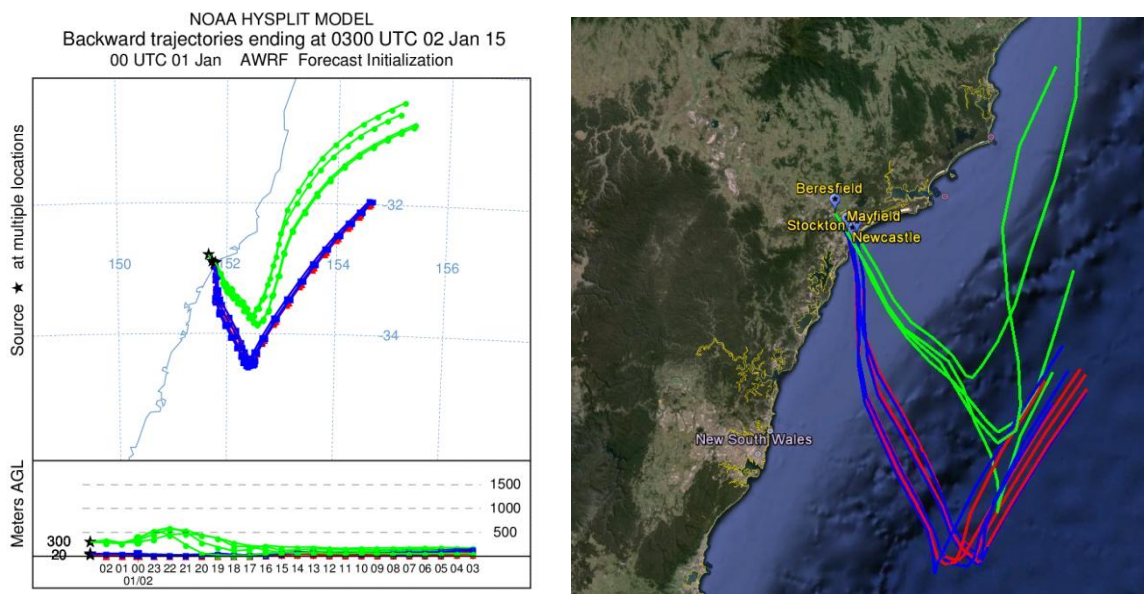
Figure 107: HYSPLIT computed backward trajectories for the 24-hour period ending at 1400 EST (0300 UTC) on 2 January 2015 from Mayfield, Newcastle, Beresfield and Stockton. HYSPLIT initialized with WRF 9km simulations
