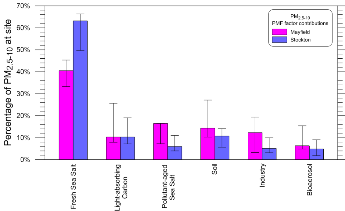
Figure 92: As for Figure 91, but showing values as percentage of annual average PM_{2.5-10} mass at each site
