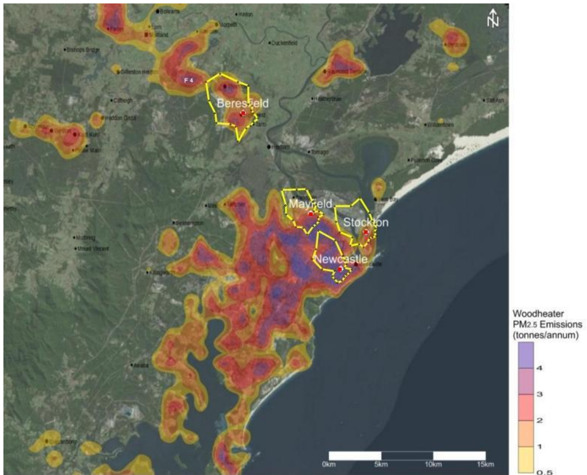
Figure 62: CPF of PM 2.5 Factor 4 (wood smoke) at the four study sites overlaid on the annual domestic wood heater PM 2.5 emissions from the Greater Metropolitan Region air emissions inventory for the 2008 calendar year (EPA 2012)
