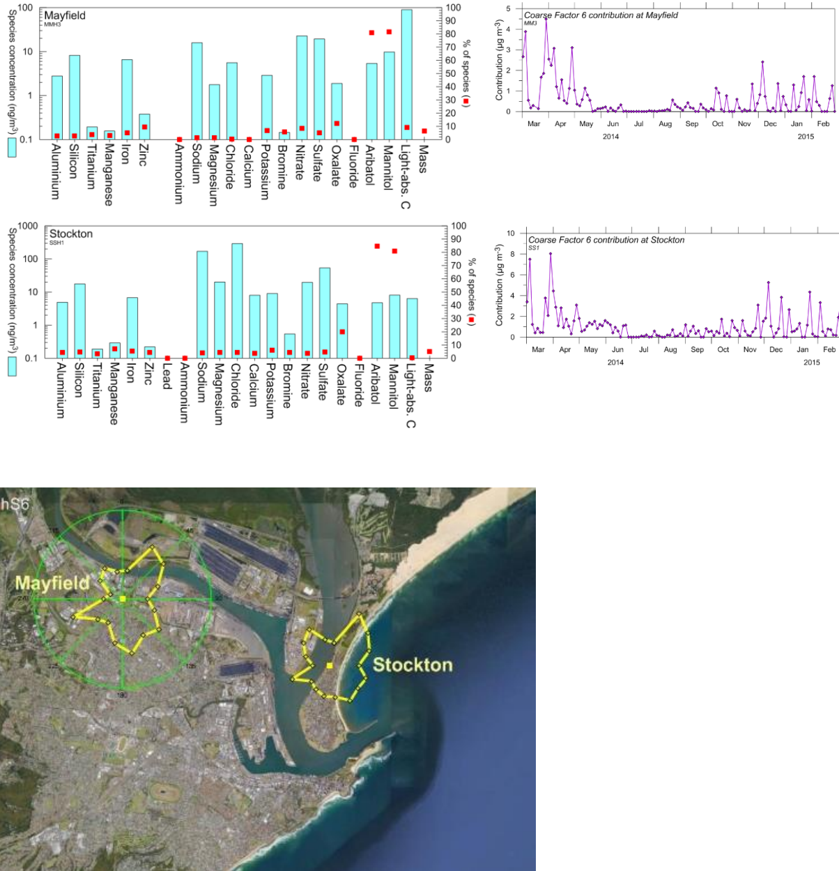
Figure 90: Fingerprints, CPF and time series plots of PM 2.5-10 Factor 6 (bioaerosol)
