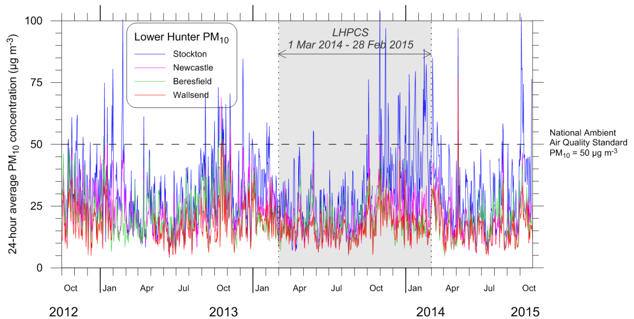
Figure 20: Long-term (Oct 2012 – Oct 2015) time series of 24-hour average PM 10 (TEOM) concentrations recorded at the OEH lower Hunter monitoring stations
