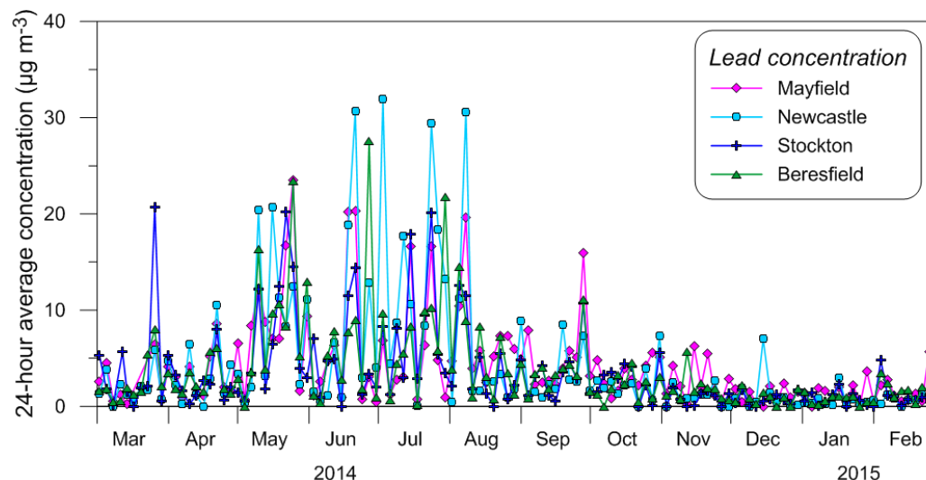
Figure 63: Time series of total lead concentrations in samples (not just in this factor)
