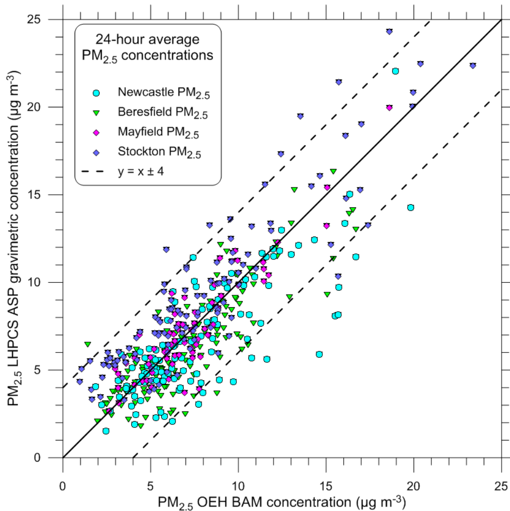
Figure 37: Comparison of PM 2.5 concentrations measured on the LHPCS filters with the regular results from the OEH Air Quality Monitoring Network using BAM instruments
