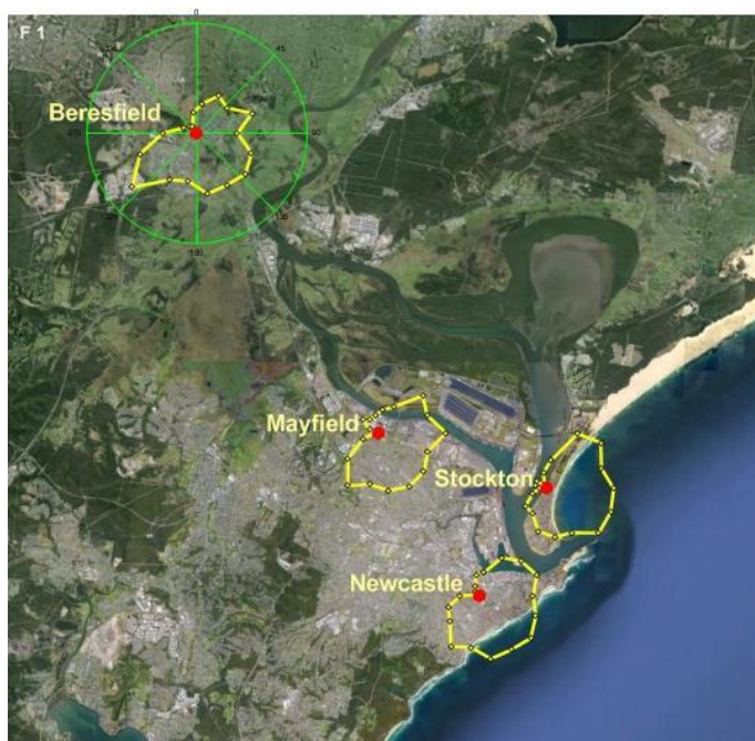
Figure 54: CPF of PM 2.5 Factor 1 (fresh sea salt) at the four study sites
