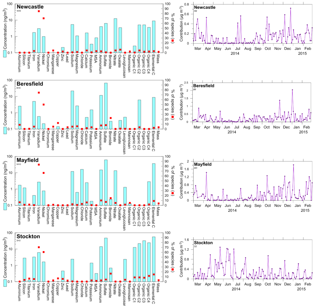
Figure 72: Fingerprints and time series plots of PM 2.5 Factor 8 (mixed shipping/industry) at the four study sites
