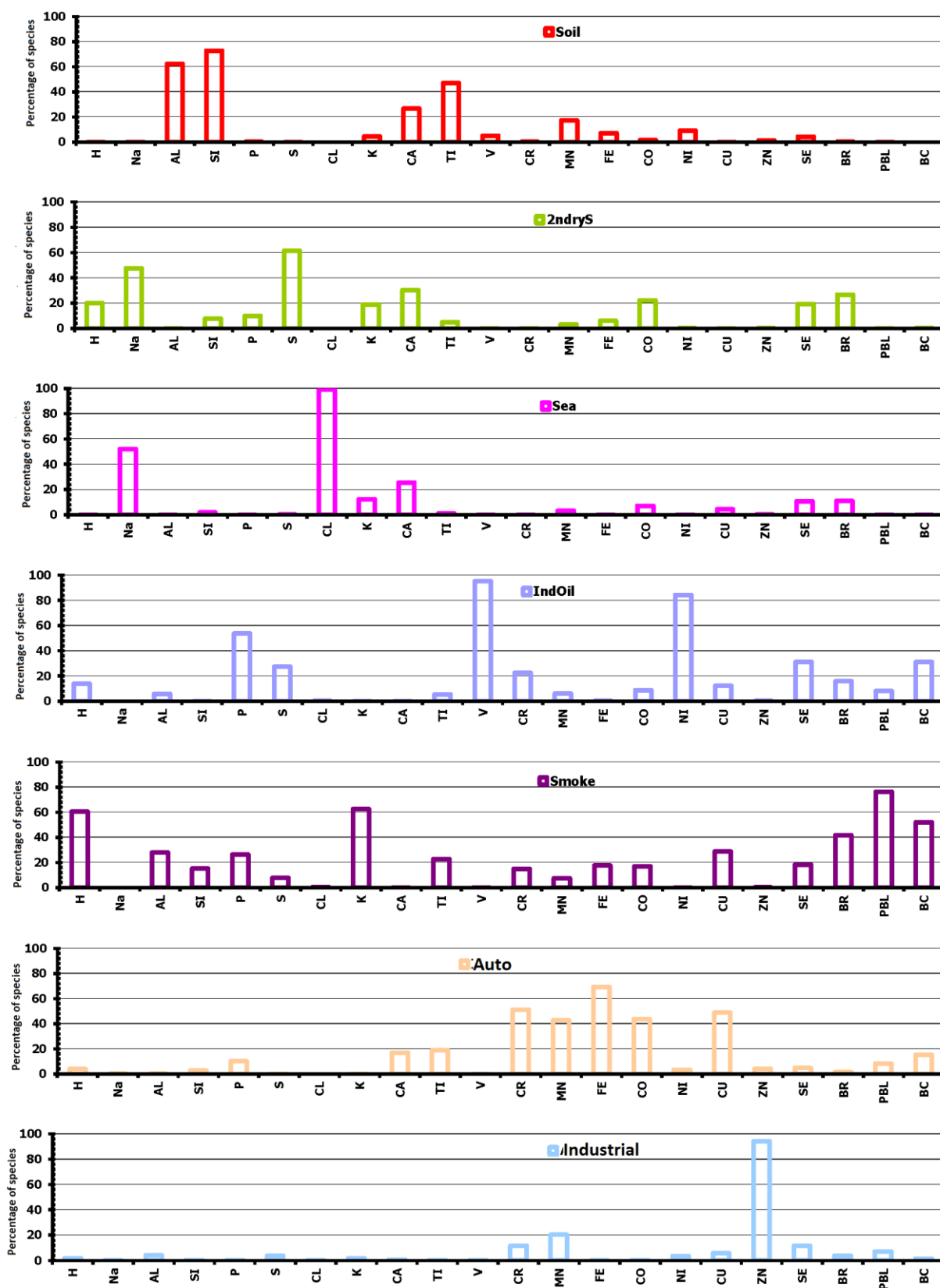
Figure 118: Percentage of each species in the factors in ANSTO's seven-factor PMF for 2010–15 IBA and BC data
