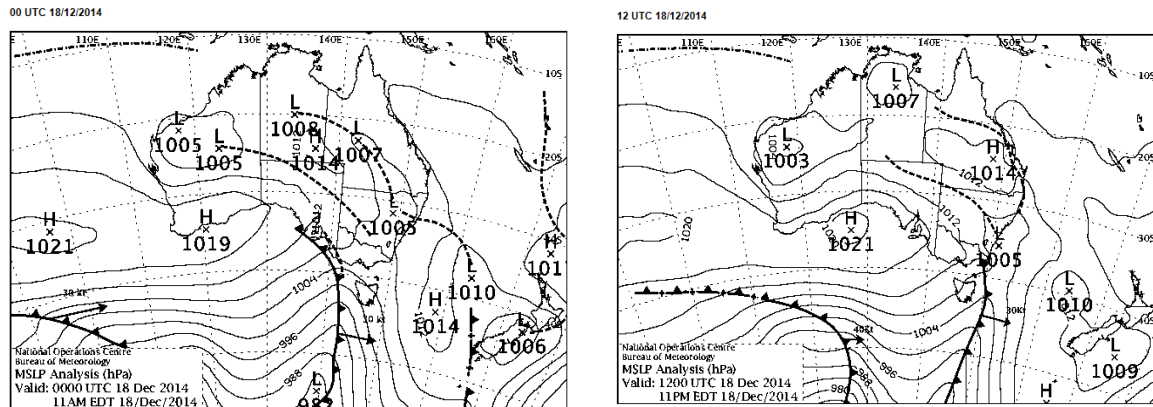
Figure 100: Surface analyses at (a) 1100 EDT and (b) 2300 EDT on 18 December 2014
