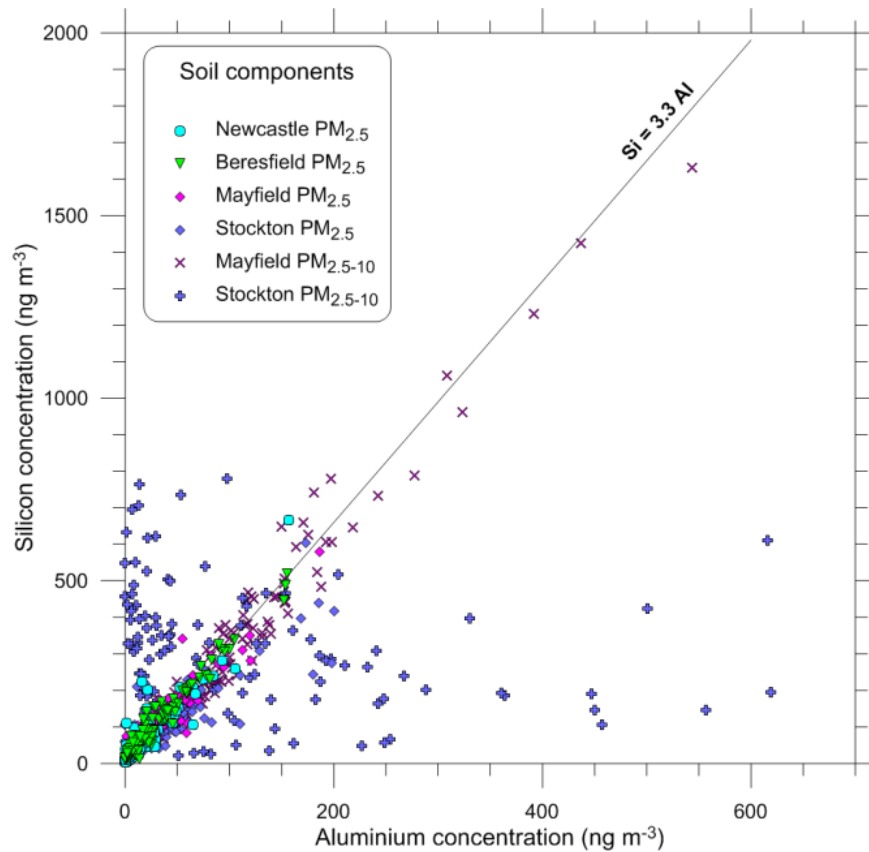
Figure 51: Scatter plot of silicon versus aluminium in PM 2.5 and PM 2.5-10
