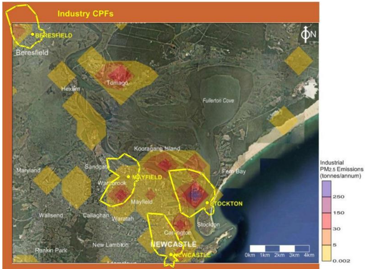
Figure 78: CPF contours overlaid on contour of PM 2.5 industrial emissions from the Greater Metropolitan Region air emissions inventory
