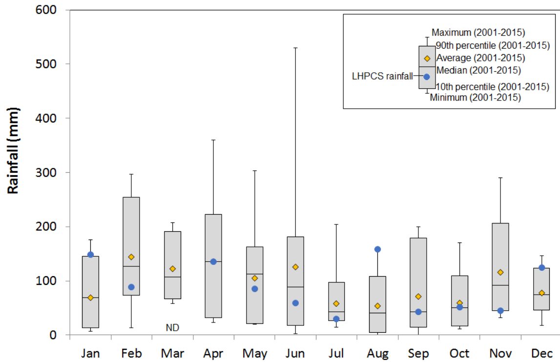
Figure 30: Comparison of rainfall recorded during the study period (March 2014 to February 2015) with rainfall statistics for the January 2001 to December 2015 period, as recorded at the Bureau of Meteorology's Newcastle University station
