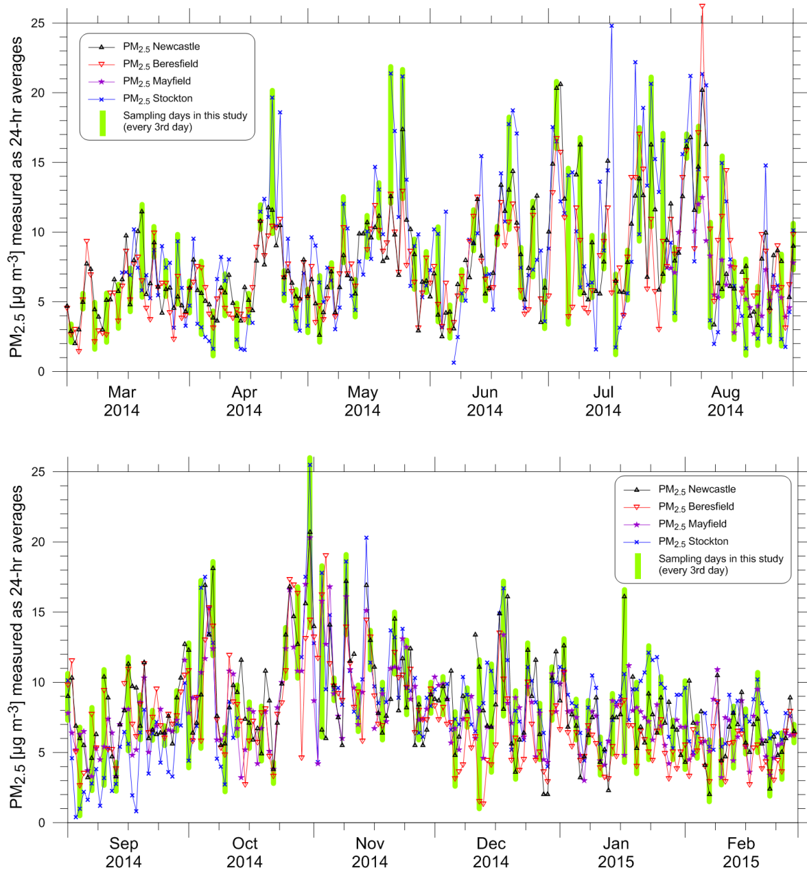
Figure 23: Time series of 24-hour average PM 2.5 concentrations measured at the Newcastle, Beresfield, Mayfield and Stockton sites using the standard BAM equipment
