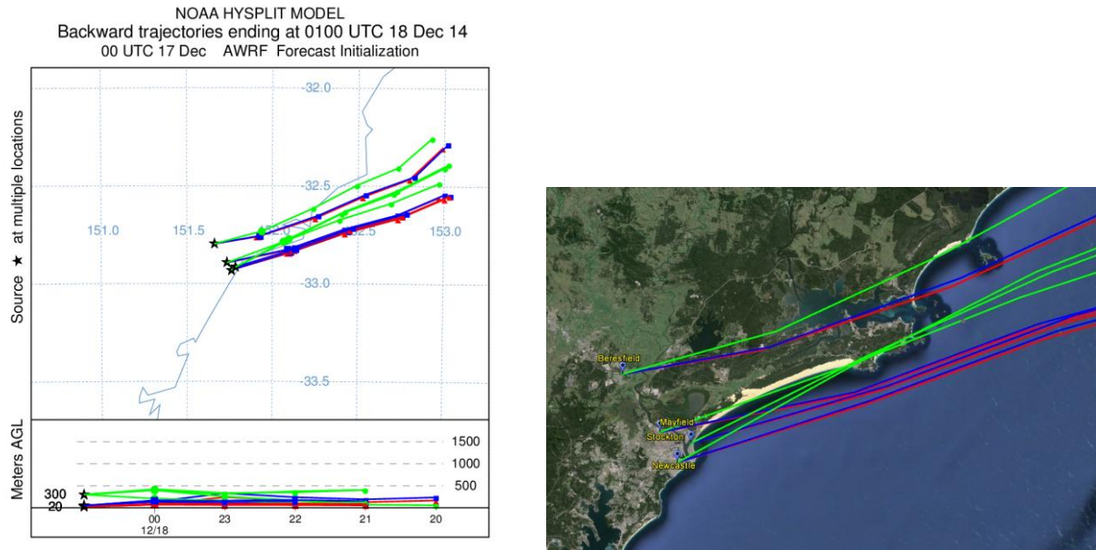
Figure 99: Same as for figure above, except HYSPLIT initialised with WRF 3km simulations
