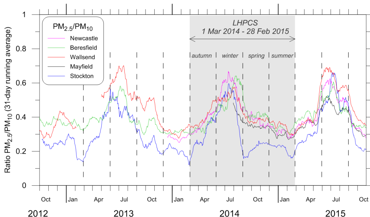
Figure 22: Long-term time series of PM 2.5 /PM 10 ratio (31-day running average) recorded at OEH and Newcastle local air quality monitoring stations (Oct 2012 – Oct 2015)
