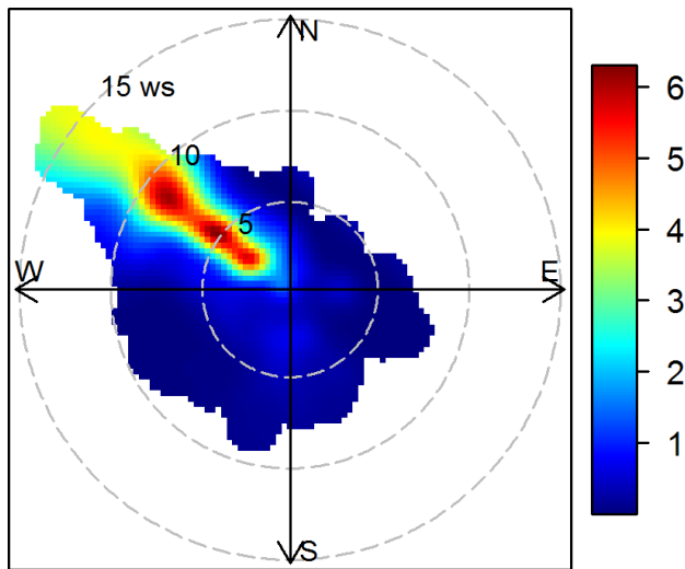
Figure 71: Bivariate pollution rose of Factor 7 (ammonium nitrate) contributions (colour scale units \mu\text{g m}^{-3} ) versus wind direction and speed ( \text{m s}^{-1} ) for the LHPCS study period
