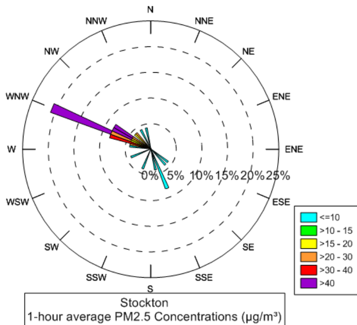
Figure 103: PM 2.5 rose for Stockton for 27 July 2014
