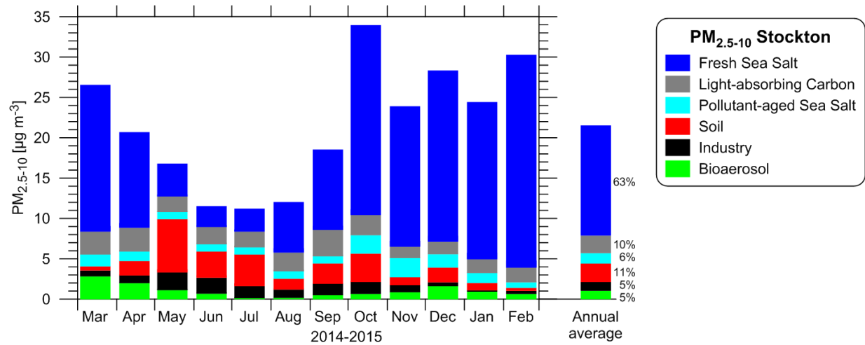
Figure 94: Monthly and annual factor contributions to PM 2.5-10 at Stockton
