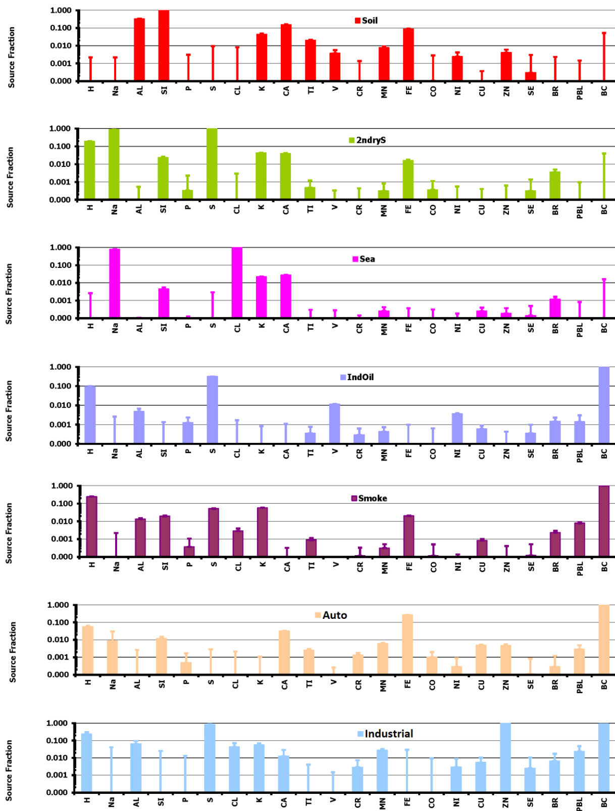
Figure 117: Fingerprints of ANSTO's seven-factor PMF for 2010–15 IBA and BC data showing the contribution of each species to the factor scaled to the largest factor contributing 1.00
