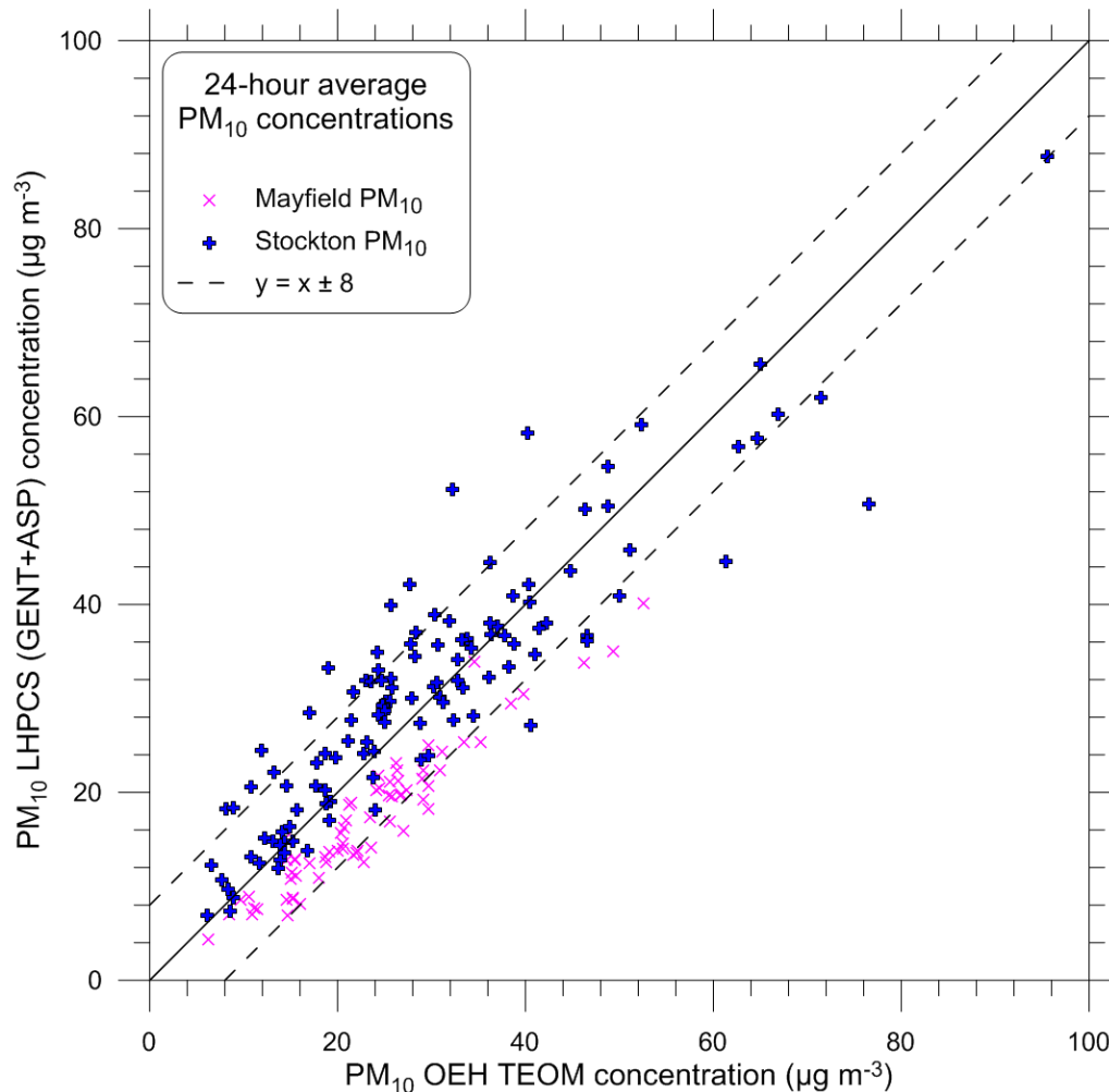
Figure 38: Comparison of PM 10 concentrations measured on the LHPCS filters with the regular results from the OEH Air Quality Monitoring Network using TEOM instruments
