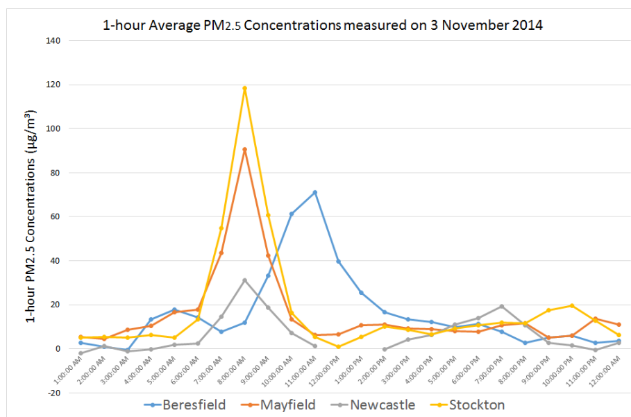
Figure 104: Hourly average \text{PM}_{2.5} concentrations measured on 3 November 2014
