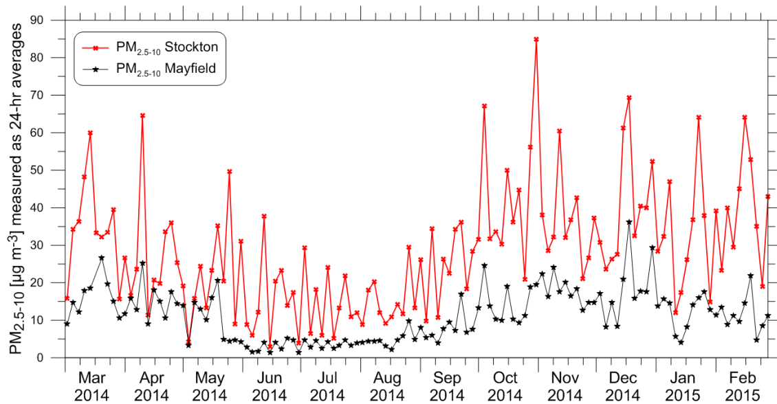
Figure 36: Time series of 24-hour average PM_{2.5-10} levels from gravimetric analysis of LHPCS samples at Stockton and Mayfield
