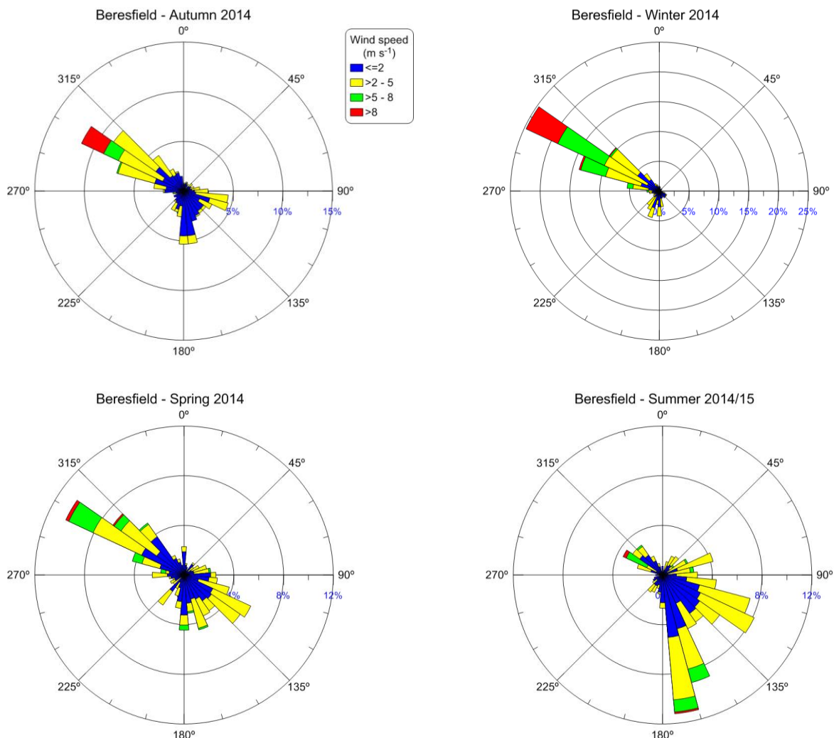
Figure 26: Seasonal wind roses from the Beresfield site (including wind data from the study sample days only)
