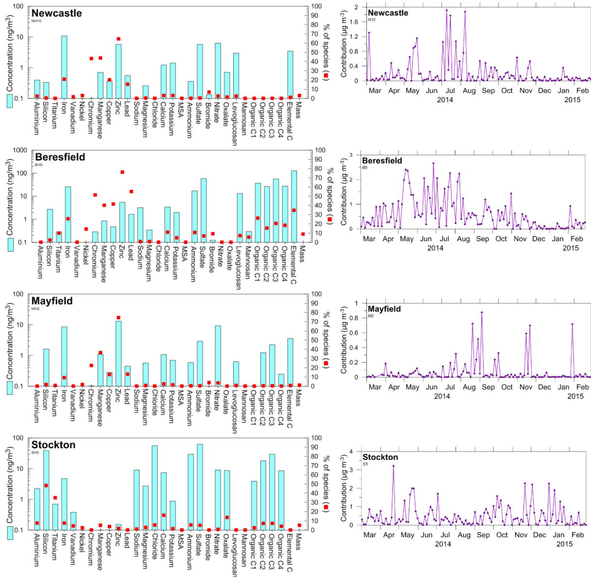
Figure 76: Fingerprints and time series plots of PM 2.5 Factor 9 (mixed industry/vehicle) at the four study sites
