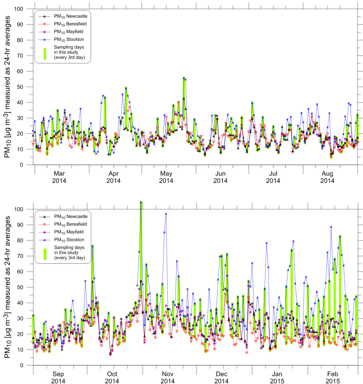
Figure 24: Time series of 24-hour average PM 10 concentrations measured at the Newcastle, Beresfield, Mayfield, and Stockton sites using the standard TEOM equipment
