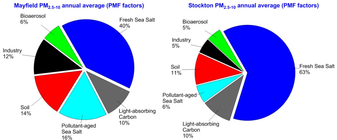
Figure 121: Pie charts of the percentage annual average factor contributions to PM 2.5-10 at the two study sites
