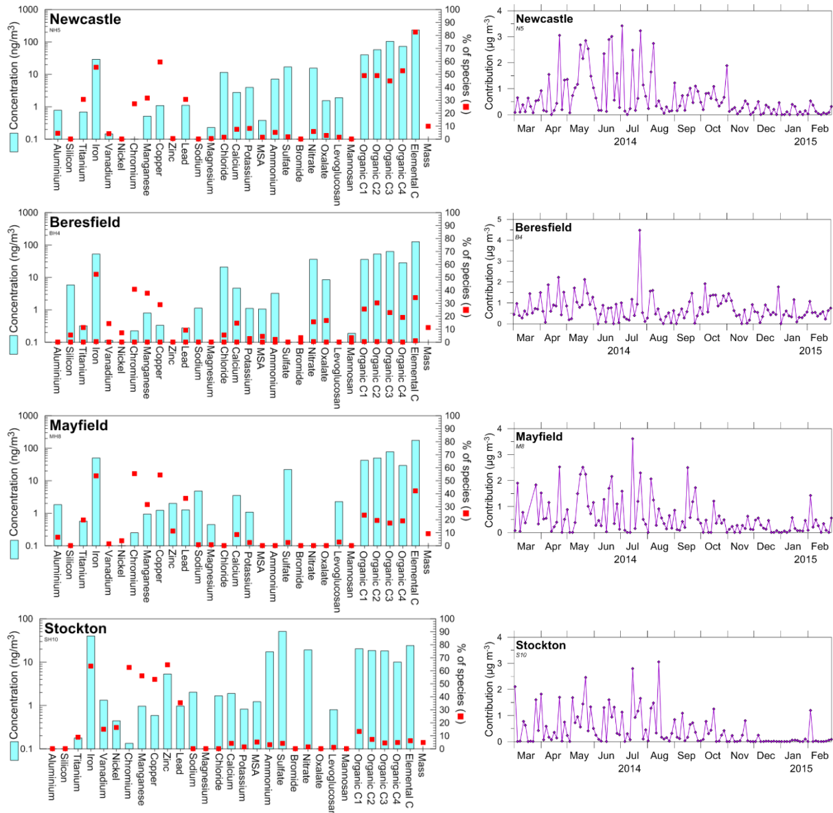
Figure 66: Fingerprints and time series plots of PM 2.5 Factor 6 (vehicle) at the four study sites
