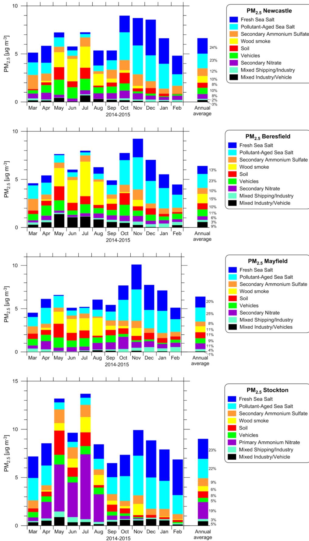
Figure S4: Monthly and annual factor contributions to PM 2.5 at the four study sites (Note: the concentration range differs for the Stockton graph.)
