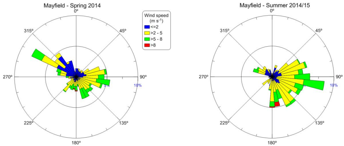
Figure 28: Seasonal wind roses from the Mayfield site (including wind data from the sample days only; data available for the second half of the study period only)
