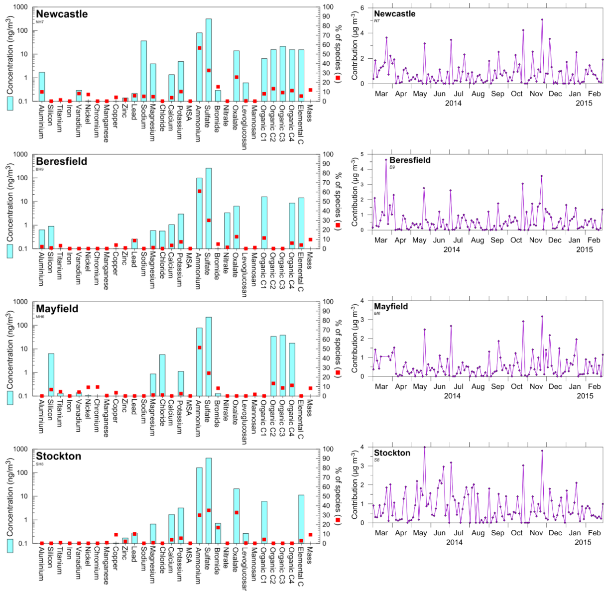
Figure 58: Fingerprints and time series plots of PM 2.5 Factor 3 (secondary ammonium sulfate) at the four study sites
