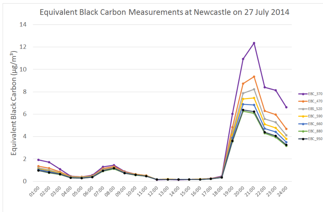
Figure 101: Diurnal variation in equivalent black carbon measured at Newcastle Air Quality Monitoring Station on 27 July 2014 using a seven wavelength aethalometer
