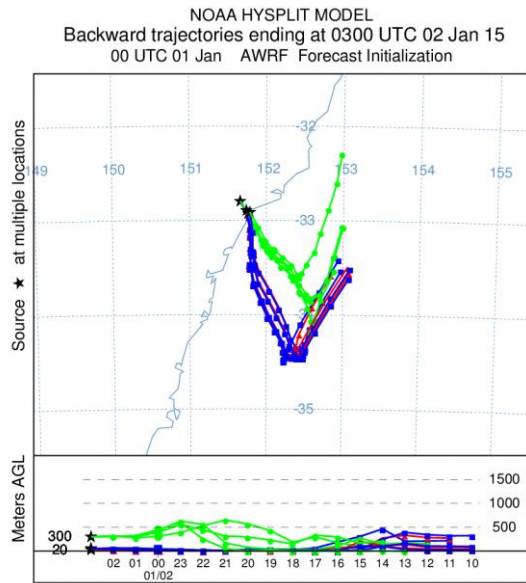
Figure 108: Same as for Figure 107, except HYSPLIT initialised with WRF 3km simulations
