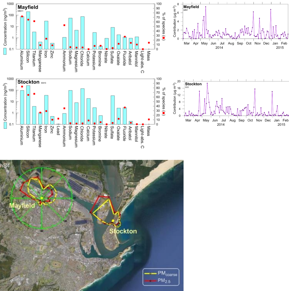
Figure 88: Fingerprints, CPF and time series plots of PM 2.5-10 Factor 4 (soil)
