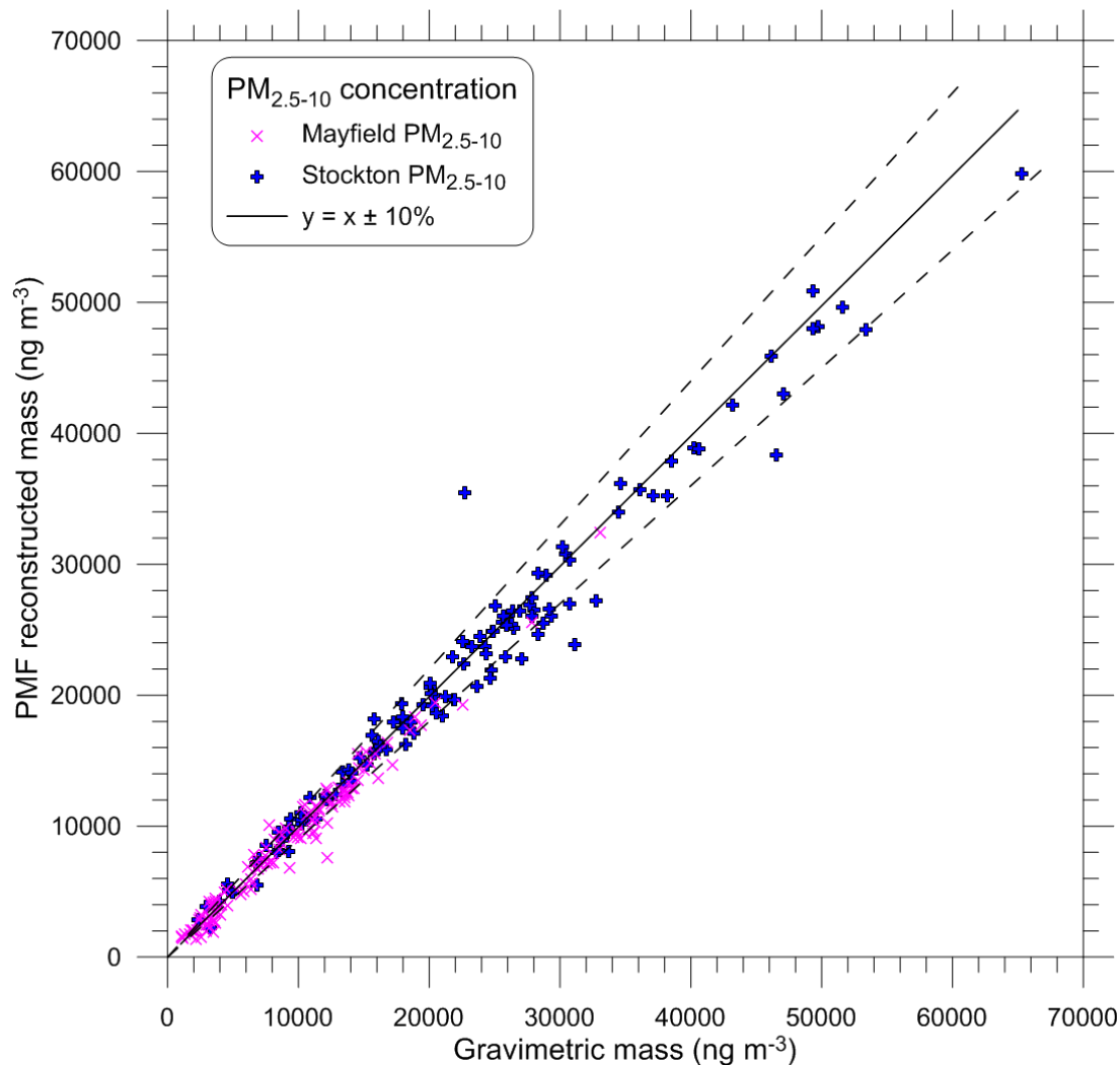
Figure 44: Scatter plot of daily PM 2.5-10 concentrations from the gravimetric mass determination and the reconstructed mass from the PMF solution
