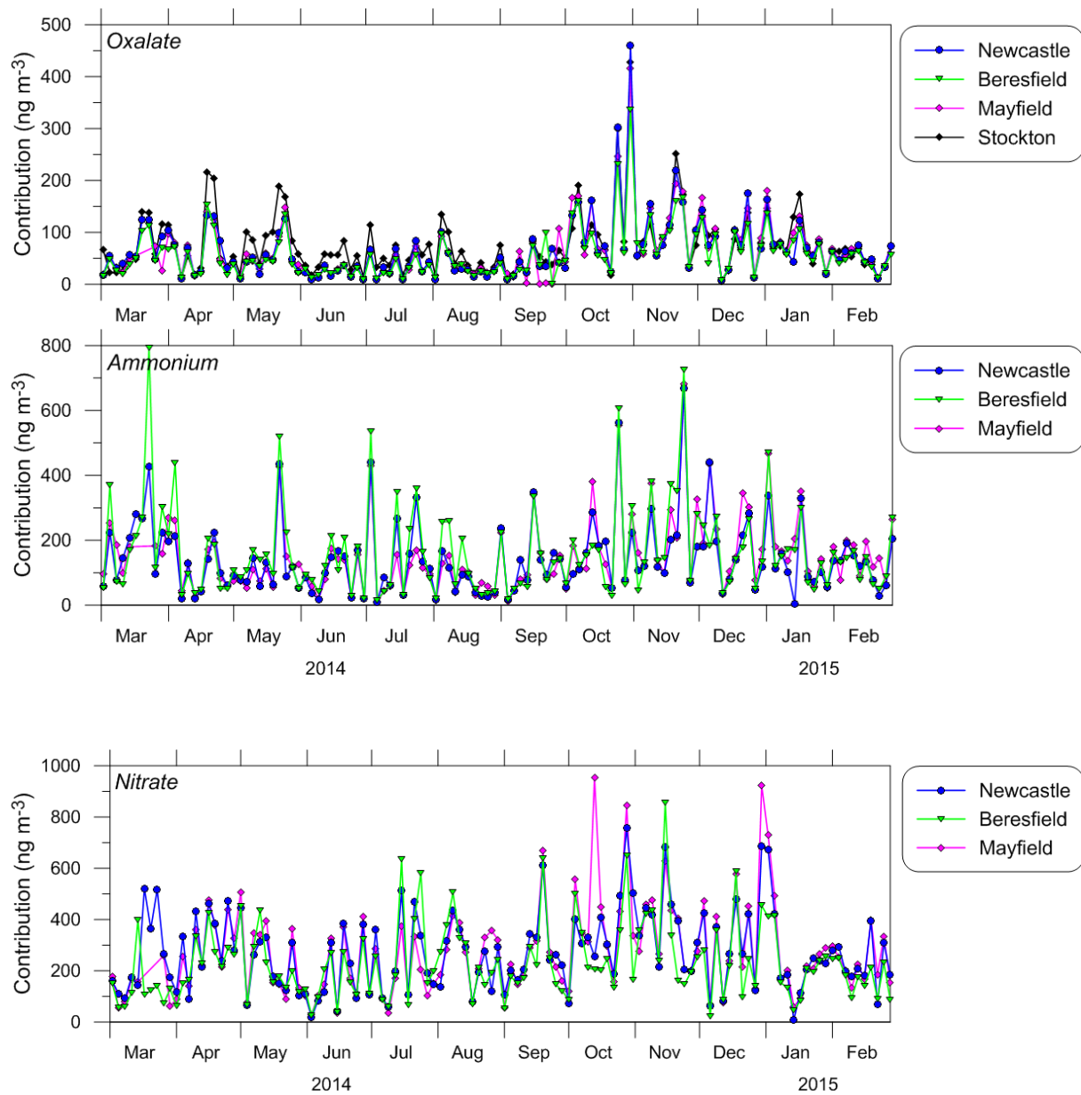
Figure 112: Time series during the study of the abundance of key species involved in secondary particle formation
