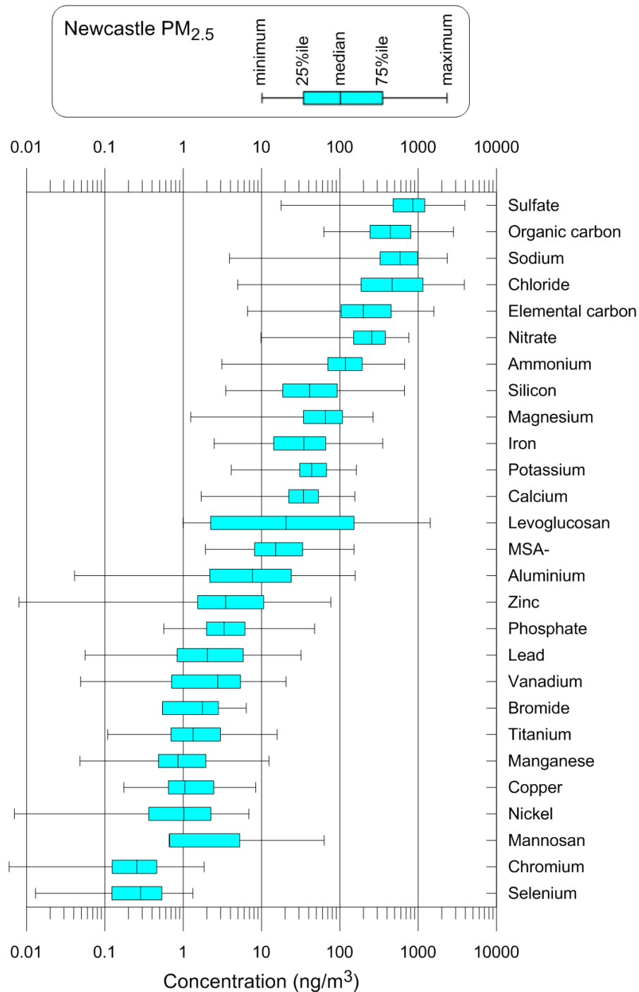
Figure 39: Box and whisker plot of the PM 2.5 species concentrations measured in the year of filter samples from Newcastle
