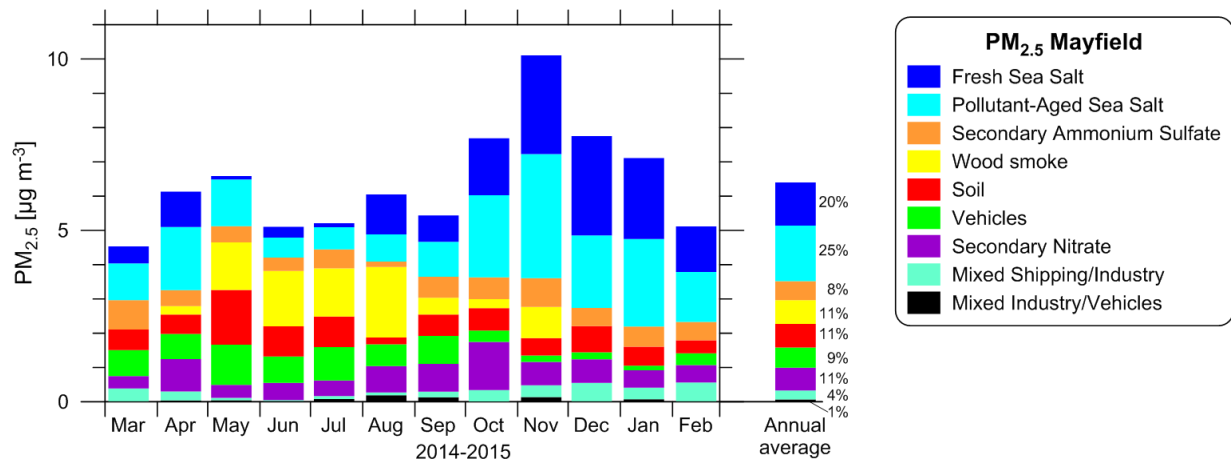
Figure 83: Monthly and annual factor contributions to PM 2.5 at Mayfield
