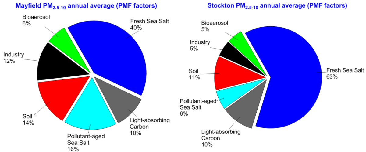
Figure S3: Percentage annual average contributions to total PM 2.5-10 mass at Mayfield and Stockton during the study
