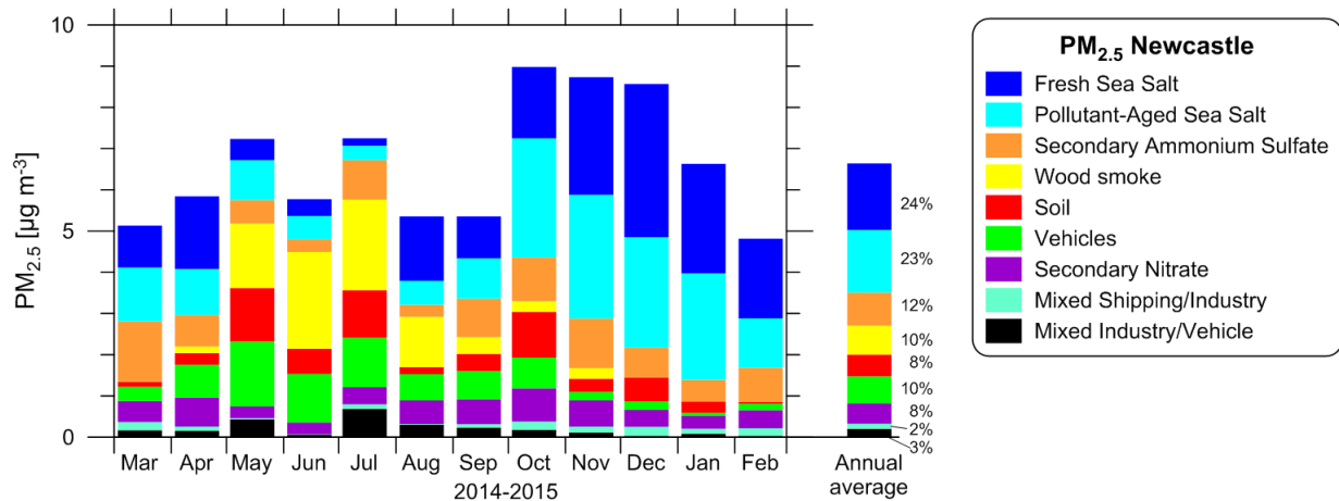
Figure 81: Monthly and annual factor contributions to PM 2.5 at Newcastle
