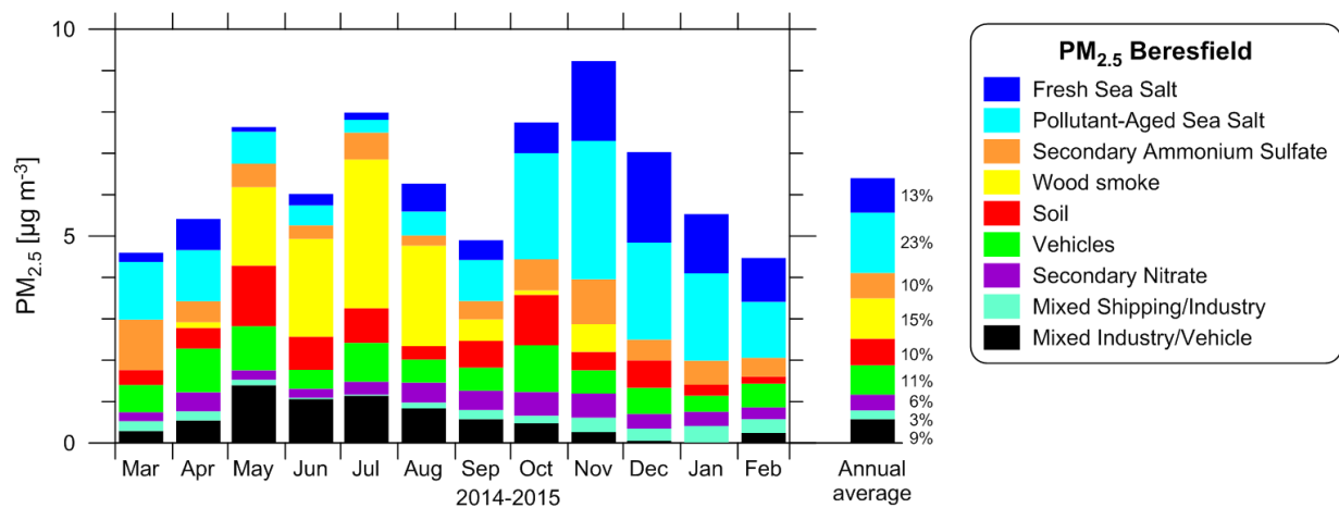
Figure 82: Monthly and annual factor contributions to PM 2.5 at Beresfield
