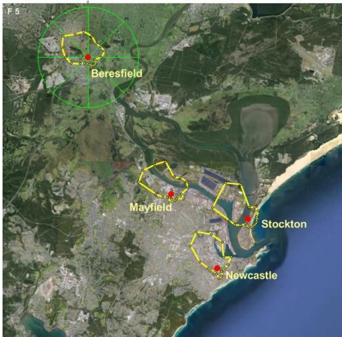
Figure 65: CPF of PM 2.5 Factor 5 (soil) at the four study sites
