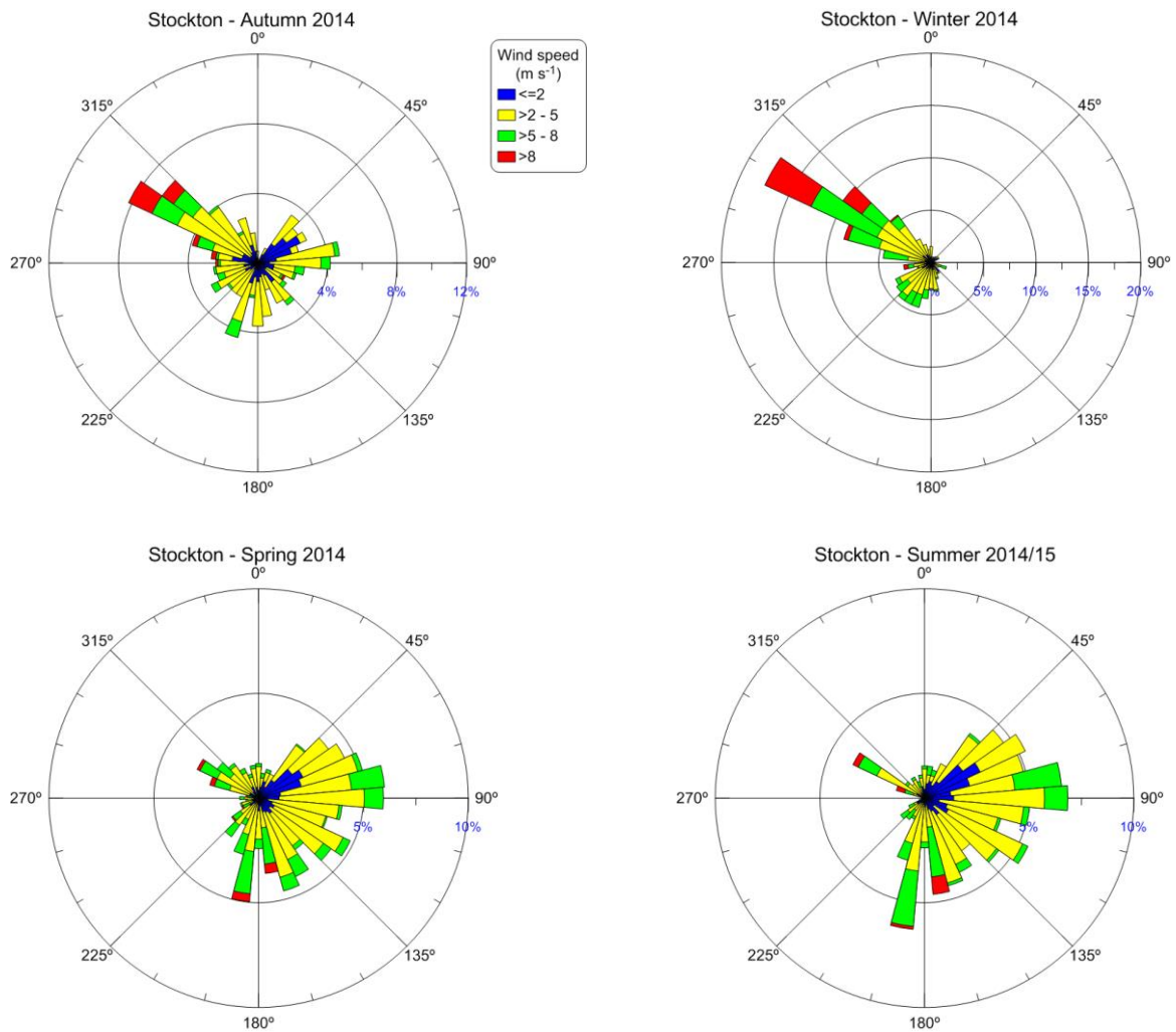
Figure 29: Seasonal wind roses from the Stockton site (including wind data from the sample days only).
