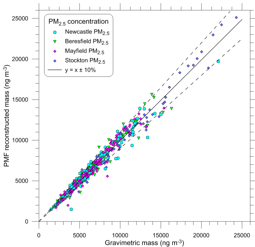
Figure 43: Scatter plot of daily PM 2.5 concentrations from the gravimetric mass determination and the reconstructed mass from the PMF solution
