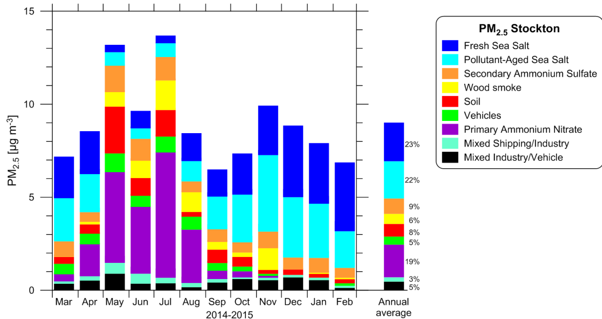
Figure 84: Monthly and annual factor contributions to PM 2.5 at Stockton
