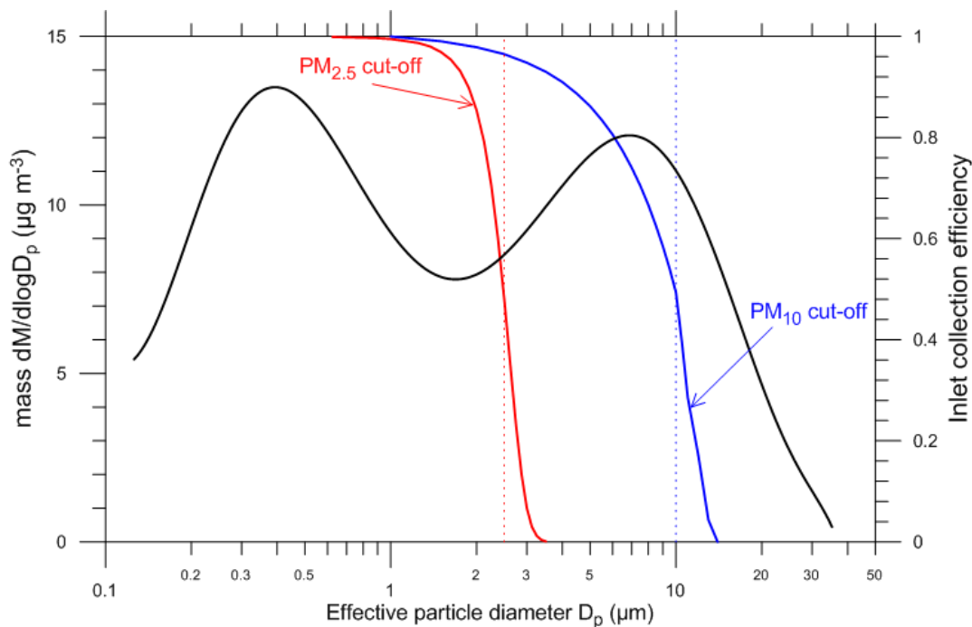
Figure 33: Size distribution measured at Liverpool in Sydney during the Australian Fine Particle Study (Keyword, pers. comm.) with size-selective inlet cut-offs for PM_{2.5} and PM_{10}
