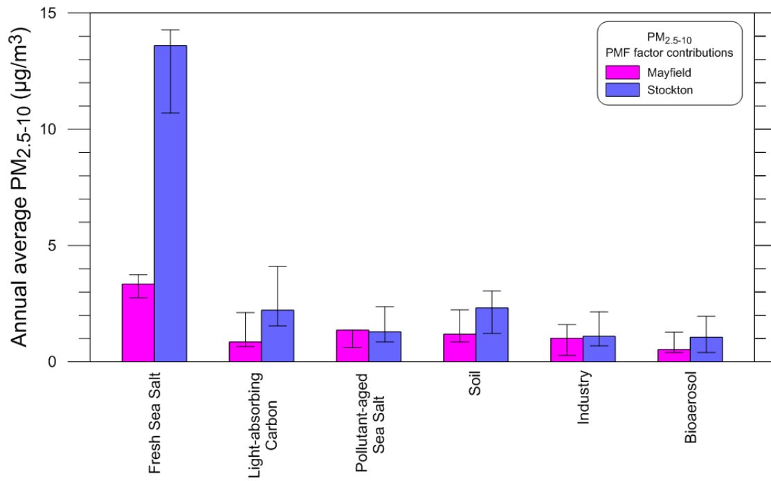
Figure 91: Comparison of the factor contributions at each site to annual average PM_{2.5-10} mass
