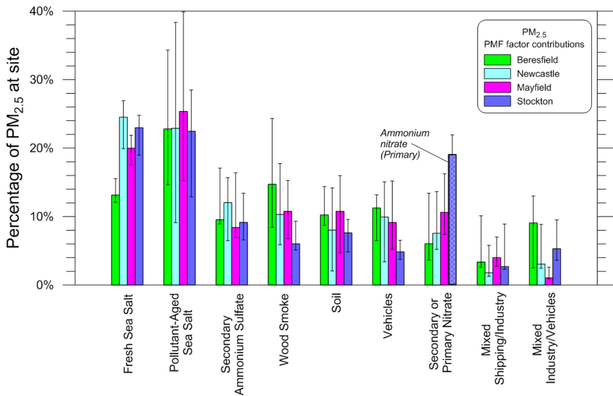
Figure 80: As for Figure 79, but showing values as percentage of annual average PM 2.5 mass at each site
