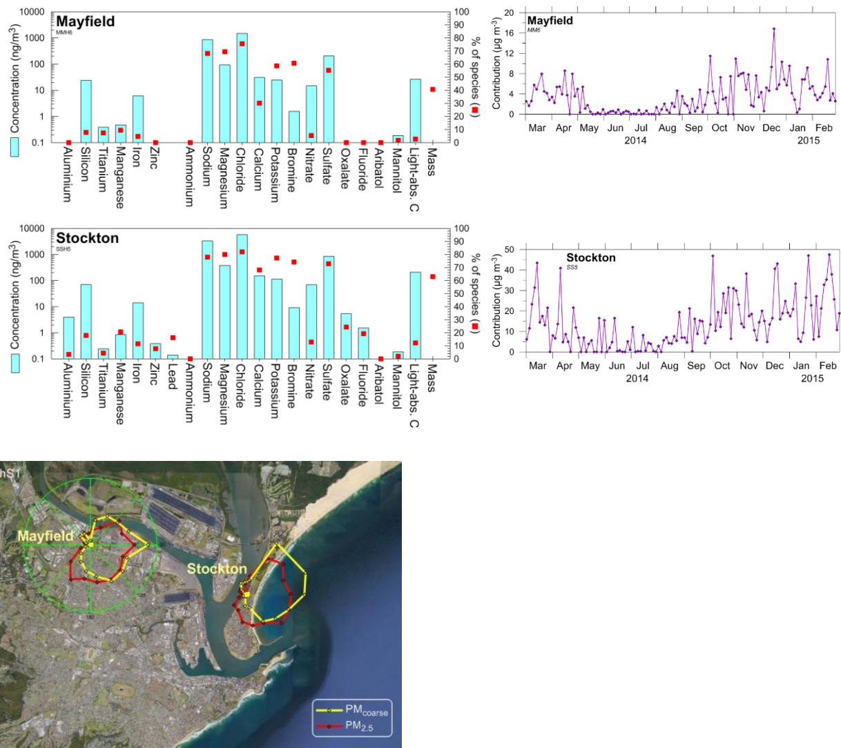
Figure 85: Fingerprints, CPF and time series plots of PM 2.5-10 Factor 1 (fresh sea salt)
