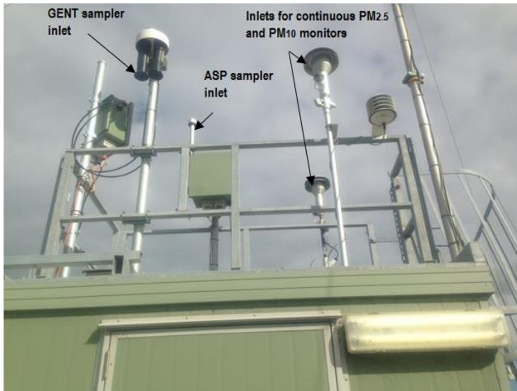
Figure 18: Identification of ASP and GENT samplers and inlets of OEHL's continuous particle monitoring instruments on the roof of the Stockton Air Quality Monitoring Station
