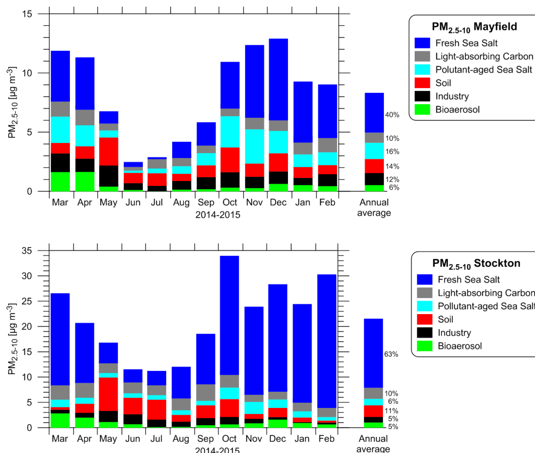
Figure S5: Monthly and annual factor contributions to PM_{2.5-10} at Mayfield and Stockton
