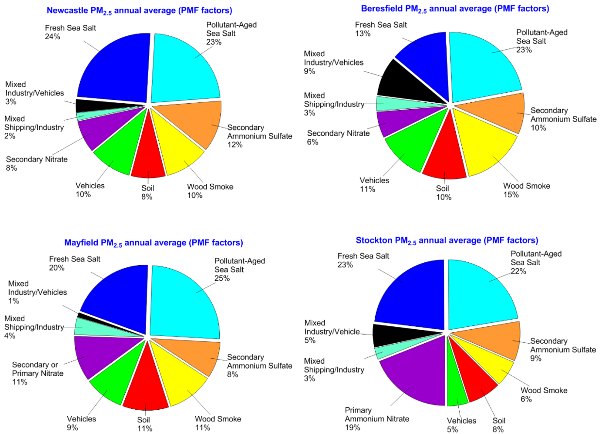
Figure 120: Pie charts of the percentage annual average factor contributions to PM_{2.5} at the study sites.
