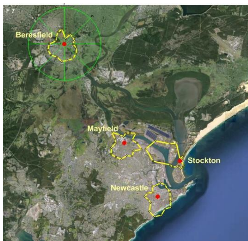
Figure 70: CPF of PM 2.5 Factor 7 (secondary sodium nitrate at three sites, primary ammonium nitrate at Stockton)
