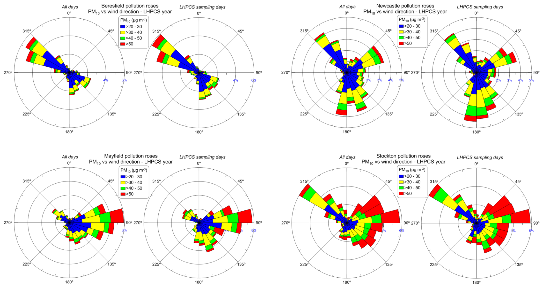
Figure 31: PM 10 pollution roses for PM 10 > 20 \mu\text{g m}^{-3} for the study period at Newcastle, Beresfield and Stockton showing close agreement between all days (left-hand side) and the 1-day-in-3 sampling days (right-hand side)
