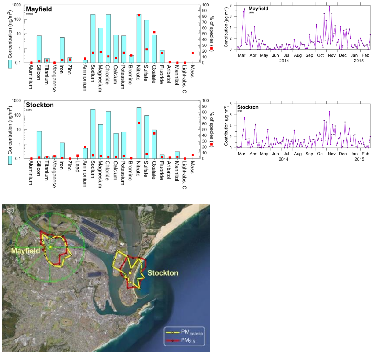
Figure 87: Fingerprints, CPF and time series plots of PM 2.5-10 Factor 3 (pollutant-aged sea salt)
