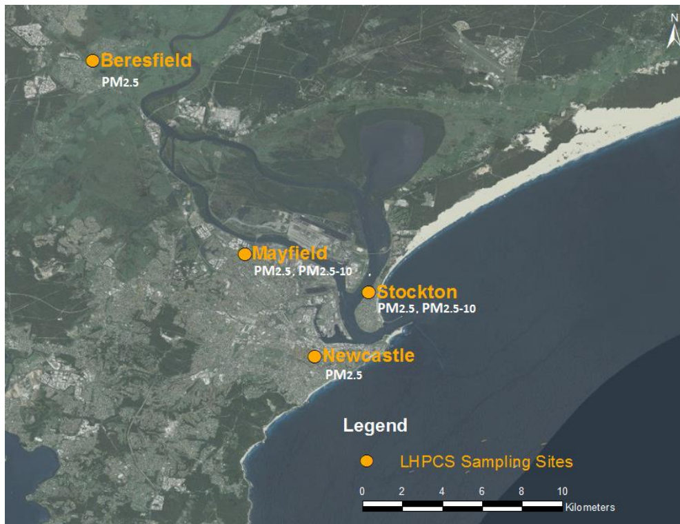
Figure 6: Sampling sites for the Lower Hunter Particle Characterisation Study
