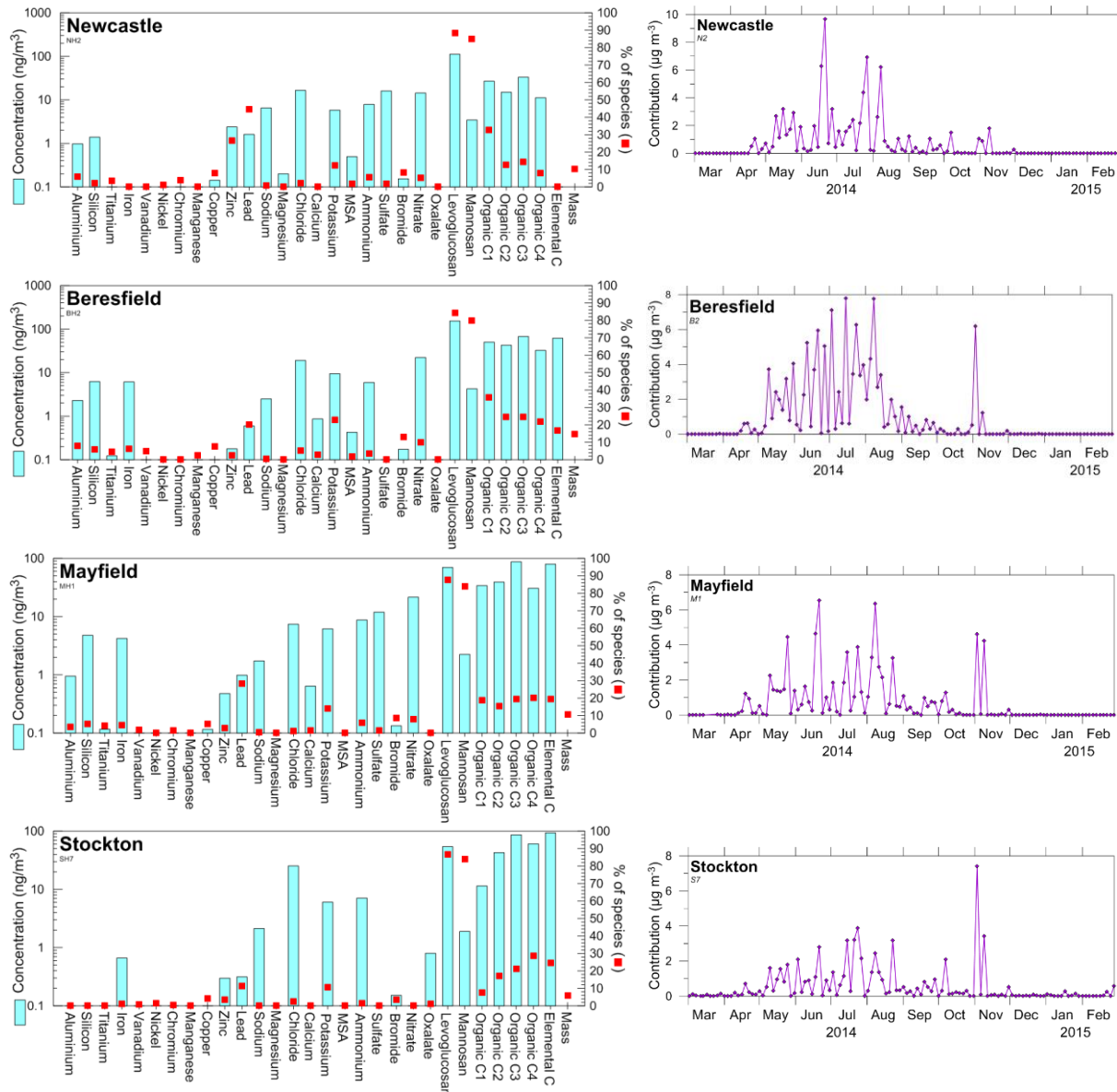
Figure 61: Fingerprints and time series plots of PM 2.5 Factor 4 (wood smoke) at the four study sites
