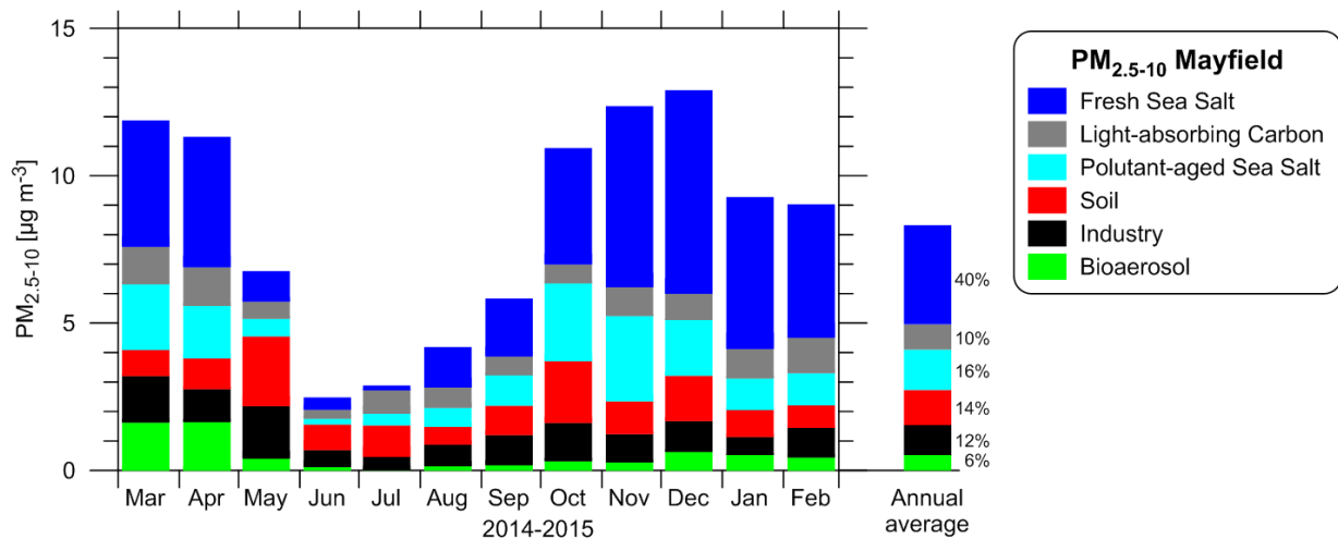
Figure 93: Monthly and annual factor contributions to PM 2.5-10 at Mayfield
