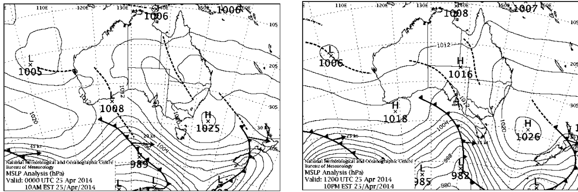
Figure 97: Surface analyses at (a) 1000 EST and (b) 2200 EST on 25 April 2014
