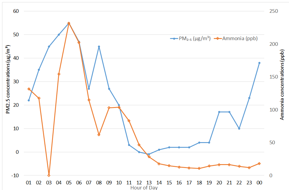
Figure 102: PM 2.5 and ammonia levels recorded at Stockton Air Quality Monitoring Station on 27 July 2014 (based on data from Orica Australia's Fuller Street Stockton station)
