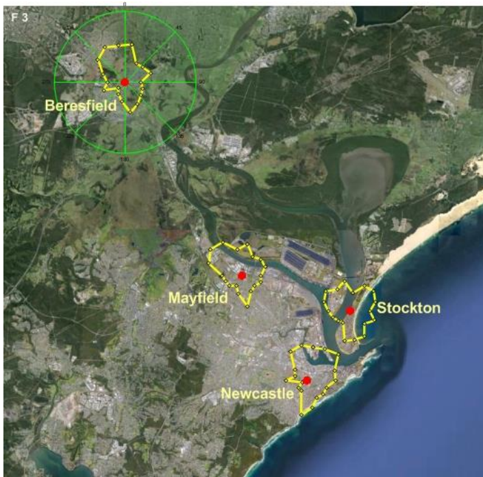
Figure 59: CPF of PM 2.5 Factor 3 (secondary ammonium sulfate) at the four study sites
