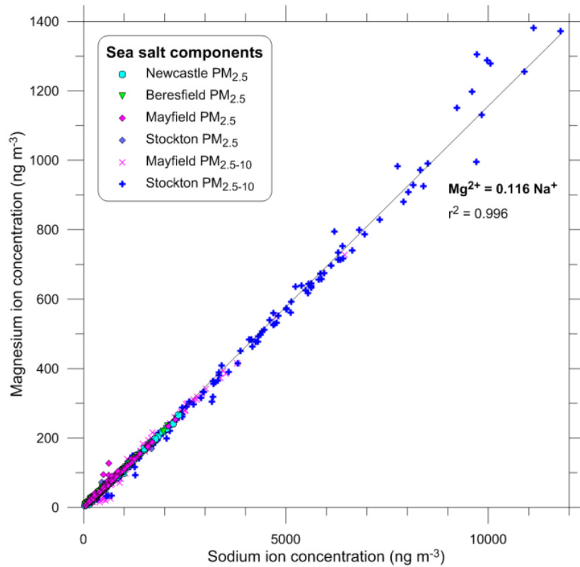
Figure 45: Scatter plot showing the strong linear relationship between magnesium and sodium concentrations in the LHPCS dataset
