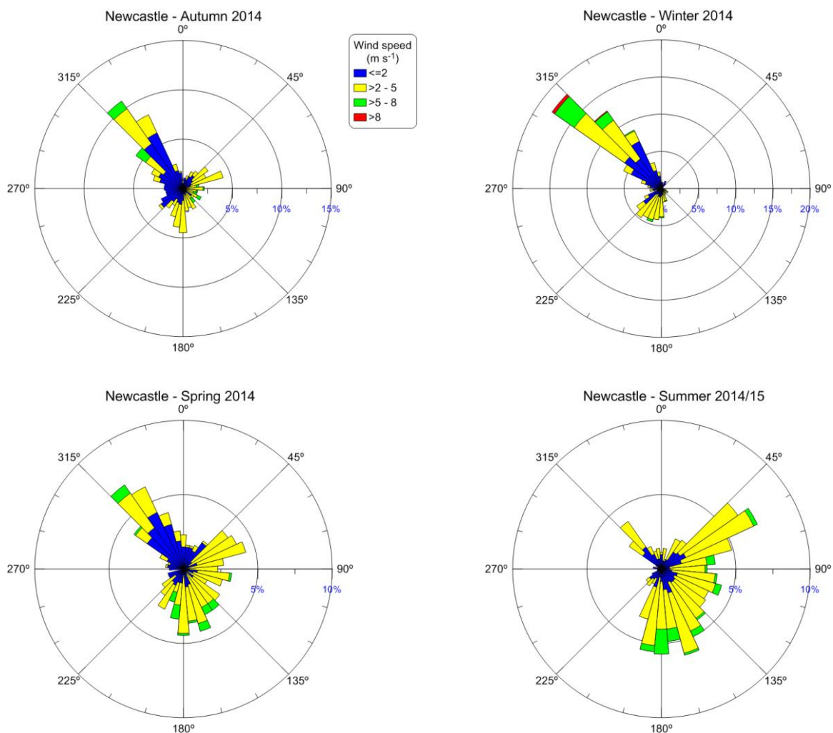
Figure 27: Seasonal wind roses from the Newcastle site (including wind data from the study sample days only)
