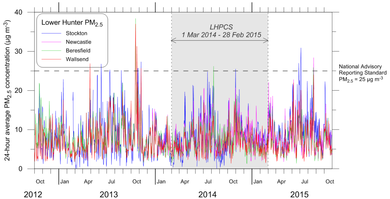
Figure 21: Long-term (Oct 2012 – Oct 2015) time series of 24-hour average PM 2.5 (BAM) concentrations recorded at the OEHL lower Hunter monitoring stations
