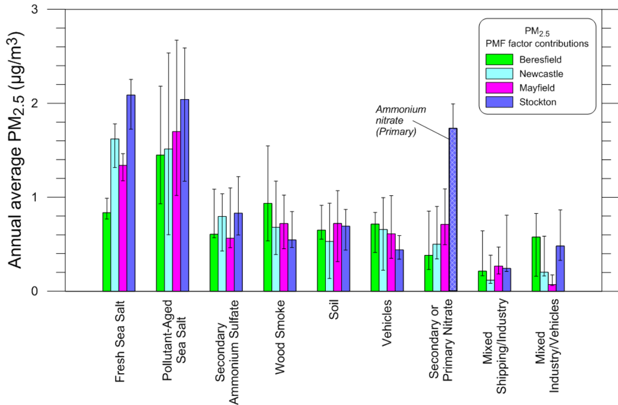
Figure 79: Comparison of the factor contributions at each site to annual average PM 2.5 mass
