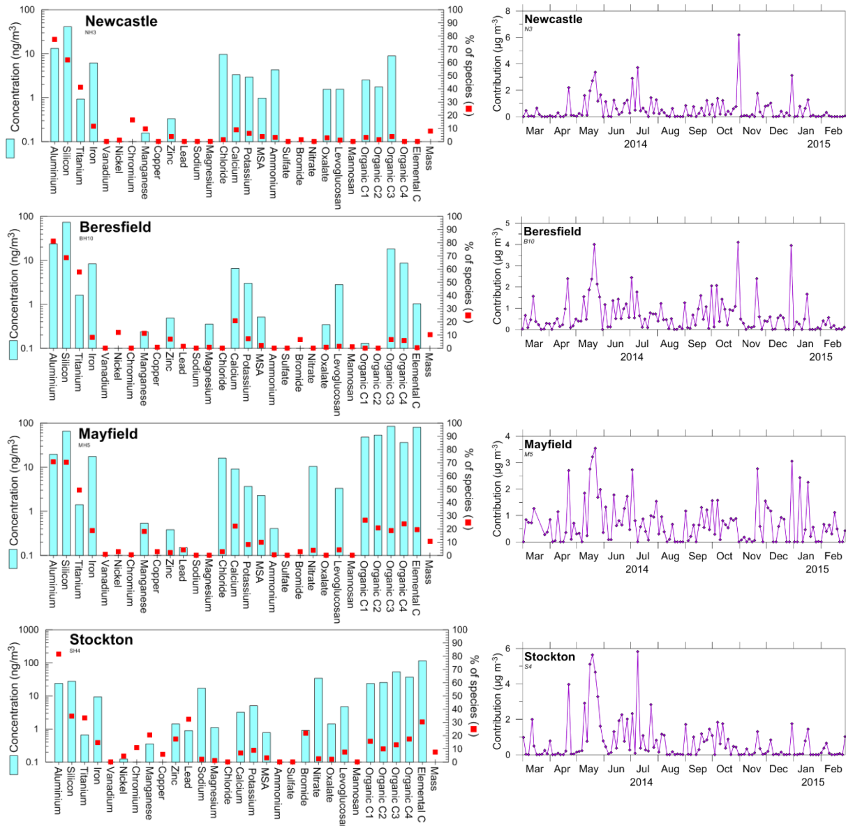
Figure 64: Fingerprints and time series plots of PM 2.5 Factor 5 (soil) at the four study sites
