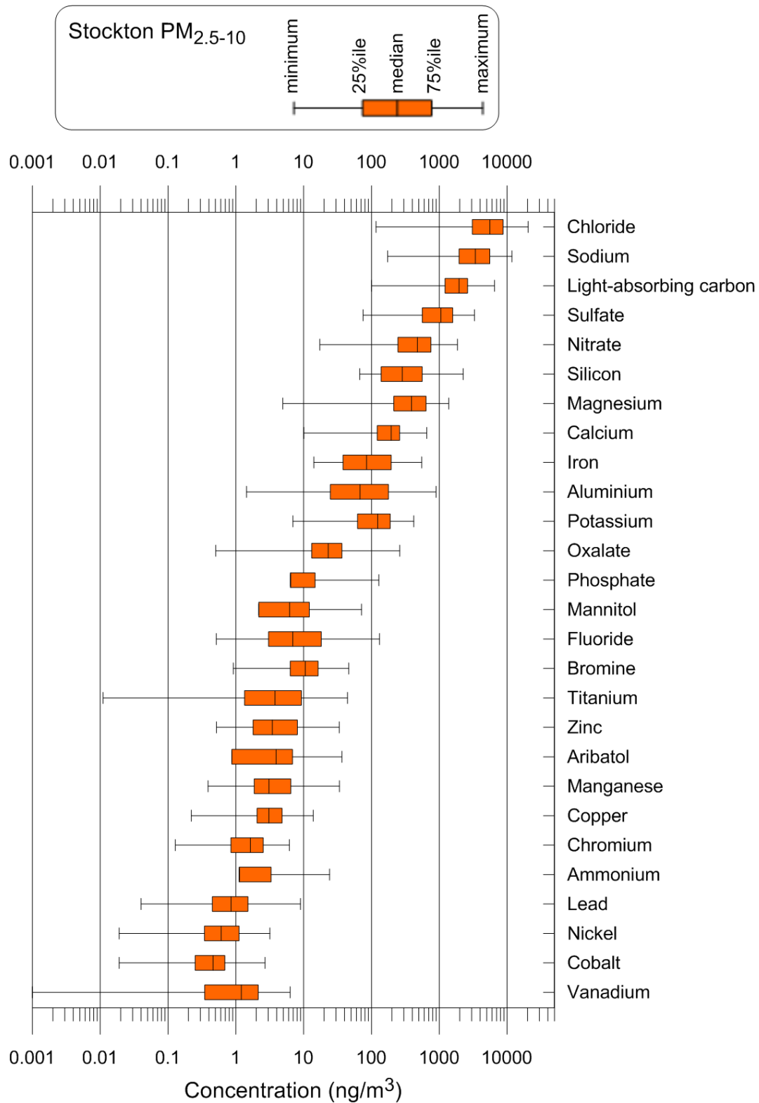
Figure 40: Box and whisker plot of the PM 2.5-10 species concentrations measured in the year of filter samples from Stockton
