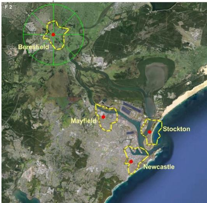
Figure 57: CPF of PM 2.5 Factor 2 (pollutant-aged sea salt) at the four study sites
