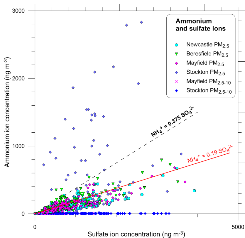
Figure 60: Scatter plot of ammonium versus total sulfate in all PM 2.5 and PM 2.5-10 samples
