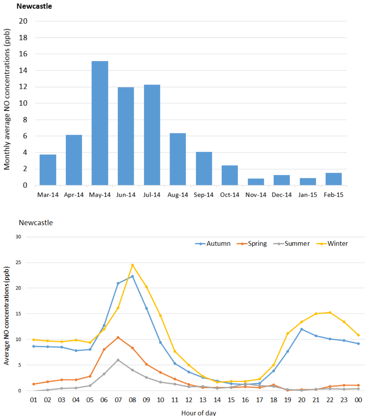
Figure 67: Monthly average nitric oxide (NO) concentrations (top) and seasonal average diurnal trends in NO concentrations (bottom) as measured at Newcastle Air Quality Monitoring Station during the study period
