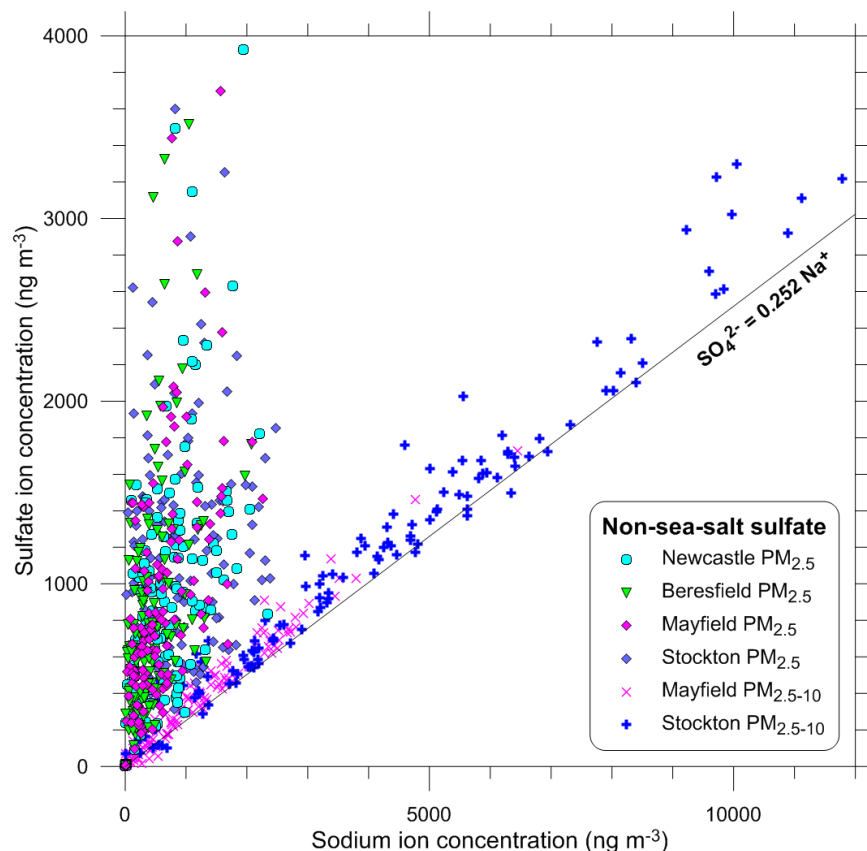
Figure 48: Scatter plot of sulfate versus sodium in fine and coarse fractions
