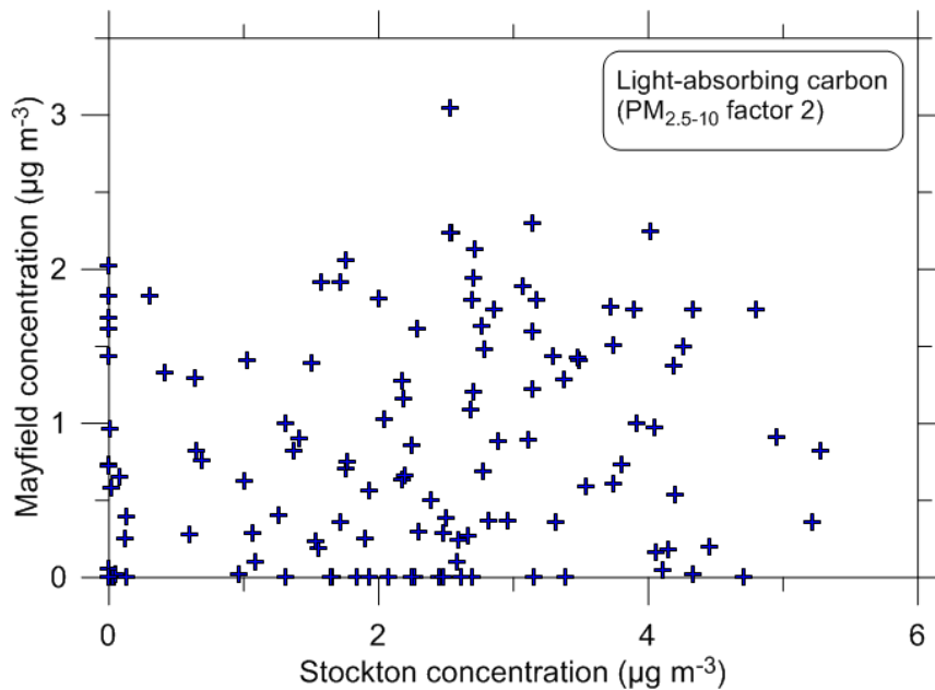
Figure 113: Scatter plot of PM 2.5-10 Factor 2 (light-absorbing carbon) measured at Stockton and Mayfield
