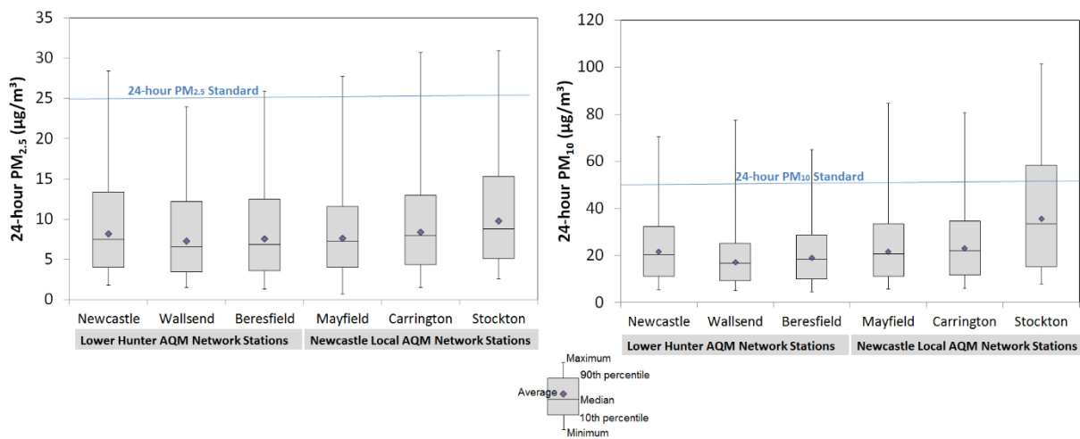
Figure 2: 24-hour average \text{PM}_{2.5} and \text{PM}_{10} concentrations measured at Lower Hunter and Newcastle Local AQMN stations (maximum, minimum, median, 90th and 10th percentile)
