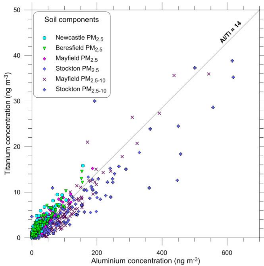
Figure 50: Scatter plot of titanium versus aluminium in PM 2.5 and PM 2.5-10
