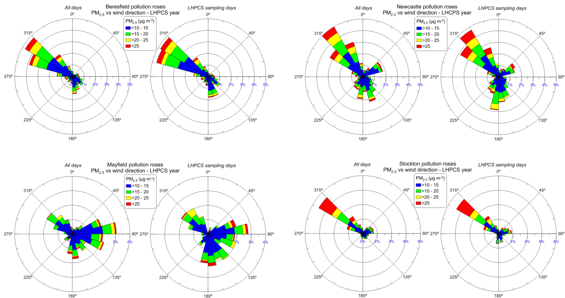
Figure 32: PM 2.5 pollution roses for PM 2.5 > 10 \mu\text{g m}^{-3} for the study period at Newcastle, Beresfield and Stockton showing close agreement between all days (left-hand side) and the 1-day-in-3 sampling days (right-hand side)
