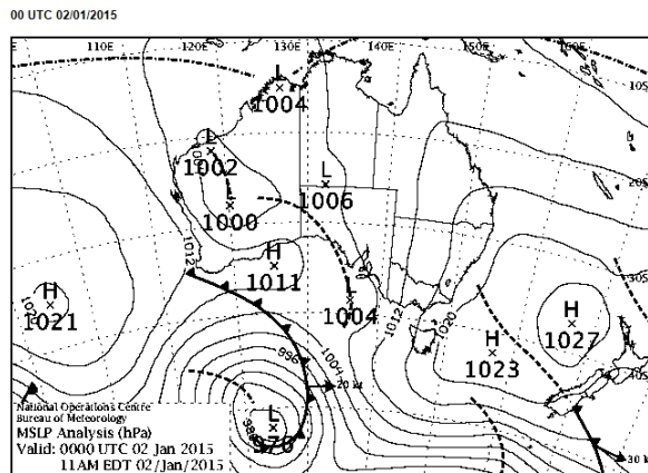
Figure 109: Surface analyses at (a) 1100 EDT and (b) 2300 EDT on 2 January 2015
