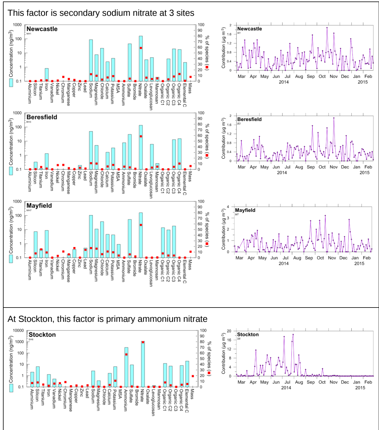
Figure 69: Fingerprints and time series plots of PM 2.5 Factor 7 (secondary sodium nitrate at three sites, primary ammonium nitrate at Stockton)
