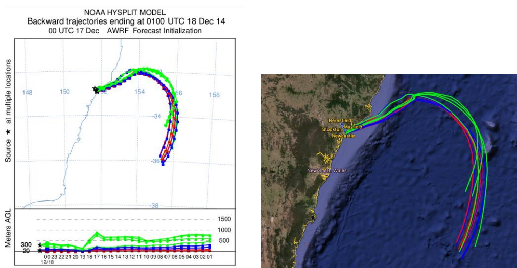
Figure 98: HYSPLIT computed backward trajectories for the 24-hour period ending at 1200 EST (0100 UTC) on 18 December 2014 from Mayfield, Newcastle, Beresfield and Stockton; HYSPLIT initialized with WRF 9km simulations
