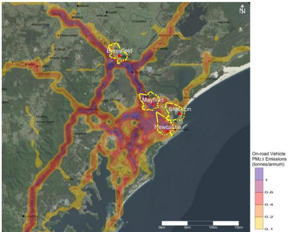
Figure 68: CPF of PM 2.5 Factor 6 (vehicle) at the four study sites overlaid on contour of PM 2.5 vehicle emissions from the Greater Metropolitan Region air emissions inventory (EPA 2012)
