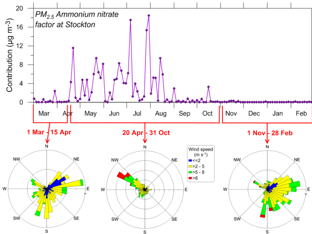
Figure 115: Wind roses at Stockton for three distinct periods identified in the ammonium nitrate factor time series trace at the top of the figure
