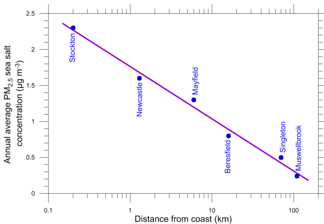
Figure 55: Variation in annual average \text{PM}_{2.5} fresh sea salt concentration with distance from coast
