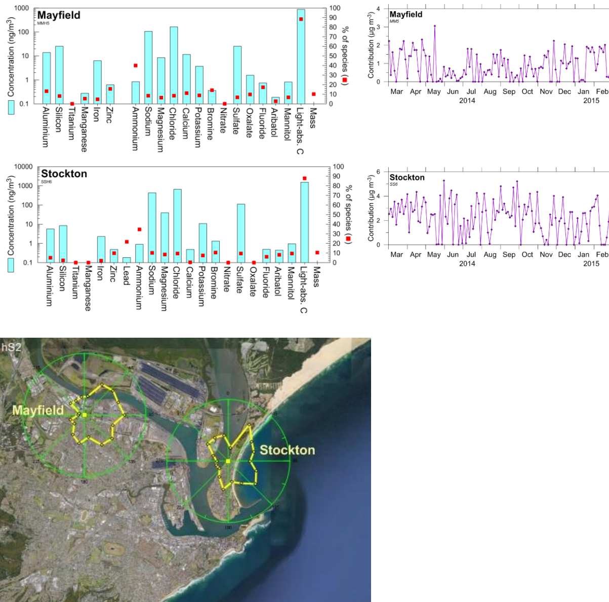
Figure 86: Fingerprints, CPF and time series plots of PM 2.5-10 Factor 2 (light-absorbing carbon)
