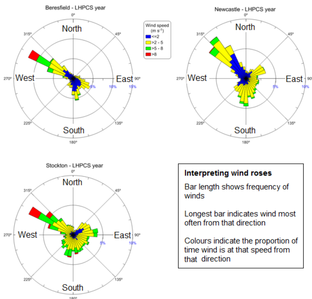
Figure 25: Annual wind roses from the study sites including data from the sample days only Mayfield not shown because wind data was only collected there for the second half of the year.
