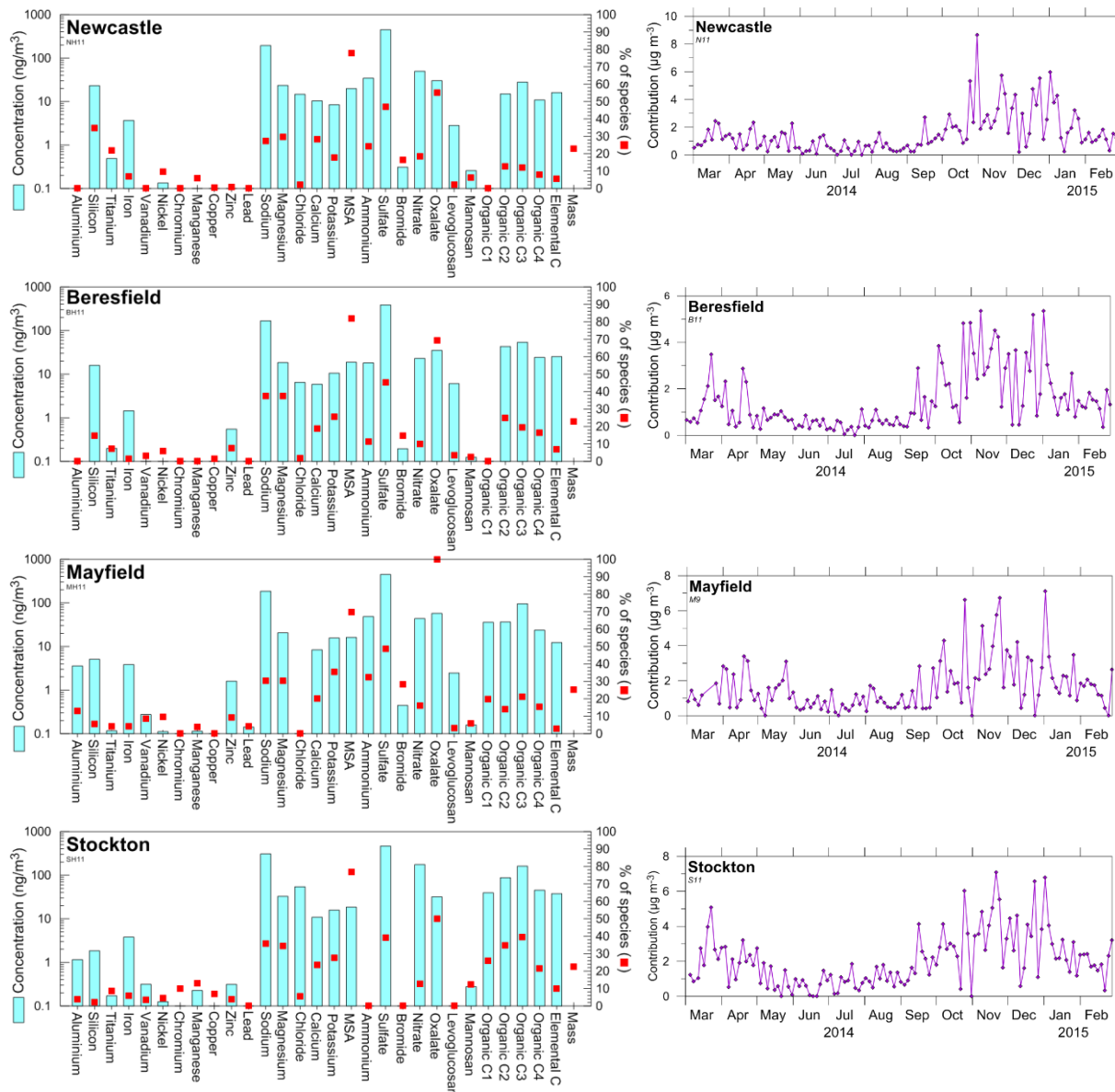
Figure 56: Fingerprints and time series plots of PM 2.5 Factor 2 (pollutant-aged sea salt) for each of the four study sites
