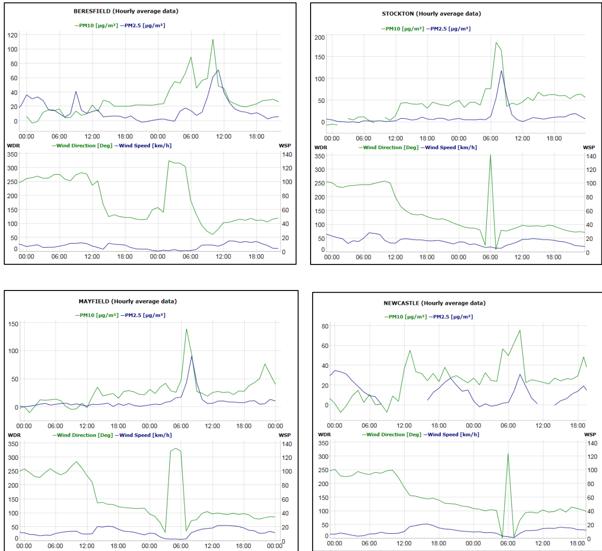
Figure 105: Hourly average wind and PM 2.5 measured 2 to 3 November 2014 showing the distinct peak in PM 2.5 (and PM 10 ) levels coinciding with north-easterly winds
