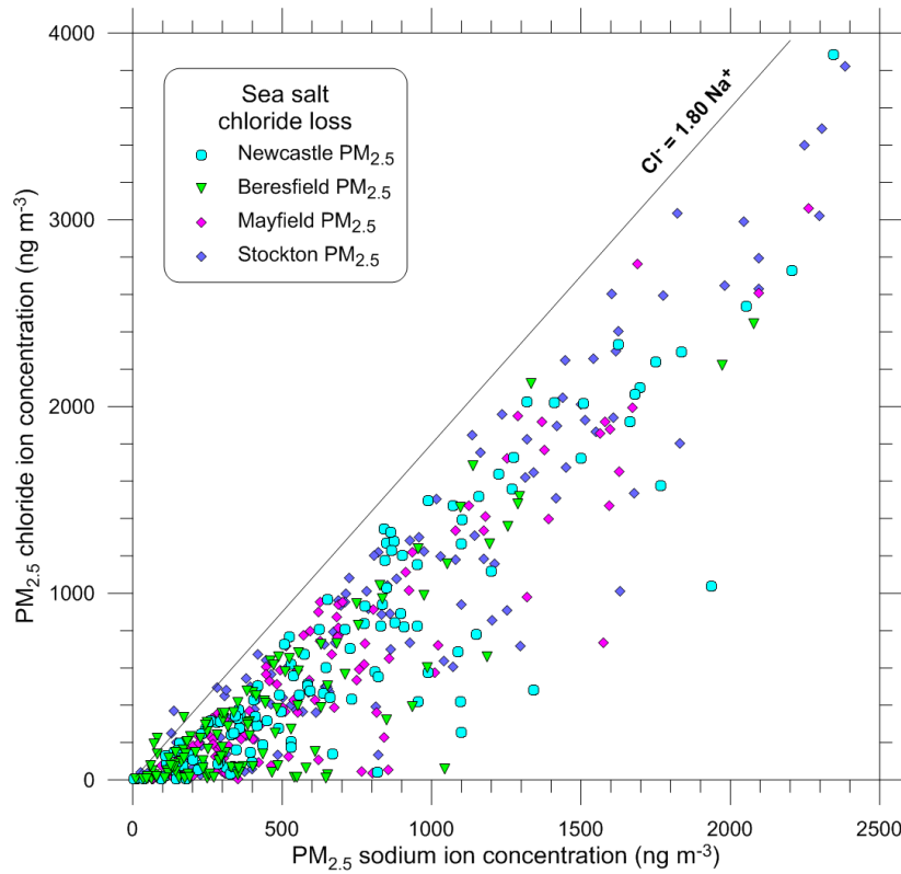
Figure 46: Scatter plot for PM 2.5 showing that for a given sodium concentration, the observed chloride concentrations are always lower than for fresh sea salt ( \text{Cl}^-/\text{Na}^+ = 1.80 ) due to the presence of ‘aged’ sea salt in the atmosphere for these 24-hour averages
