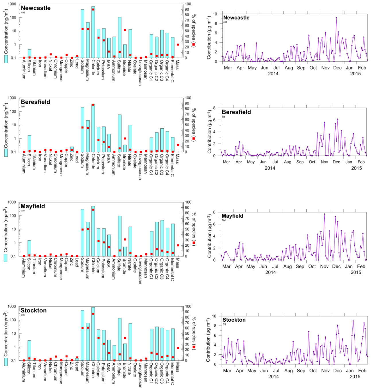
Figure 53: Fingerprints and time series plots of PM 2.5 Factor 1 (fresh sea salt) at the four study sites
