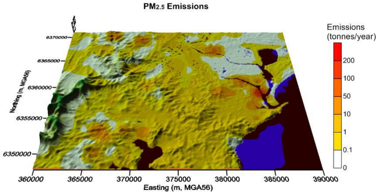
Figure 4: Spatial distribution of primary PM 2.5 emissions for the 2008 calendar year
