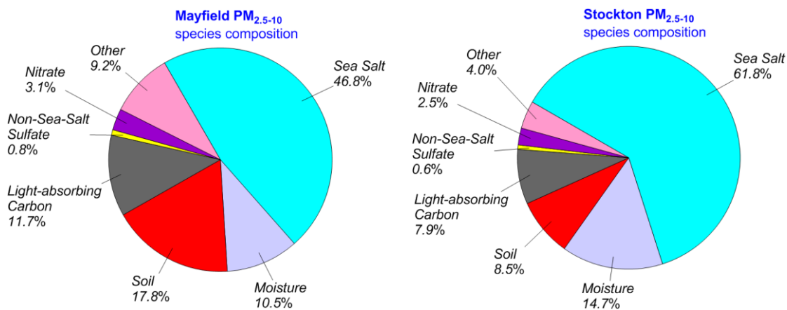
Figure 42: Main components of PM_{2.5-10} based on the chemical speciation (annual averages)
