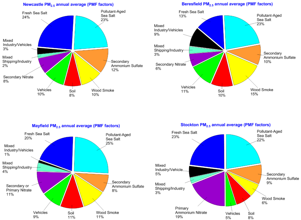
Figure S2: Percentage annual average contributions to total PM 2.5 mass at the four study sites during the study
