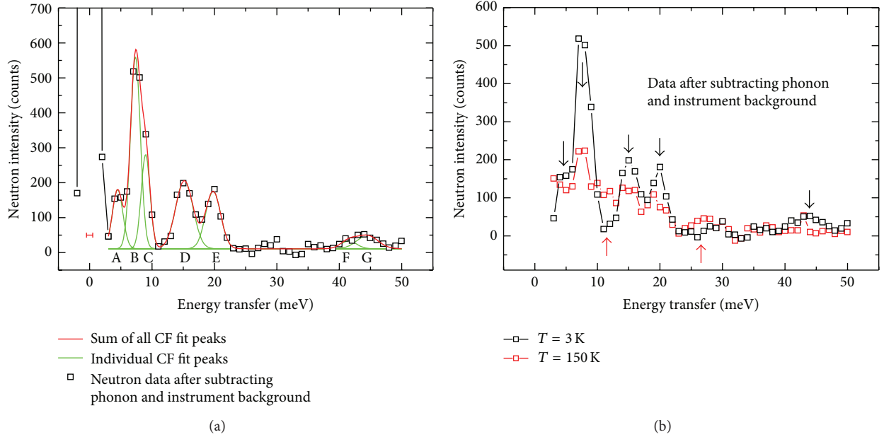
FIGURE 2: (a) Energy spectra of CF excitations in \text{NdFeAsO}_{0.85}\text{F}_{0.15} at T = 3\text{ K} after subtracting the phonon and instrument background. The spectra were well fitted by seven Gaussian peaks. The instrumental energy resolution is 0.98\text{ meV} at elastic position (horizontal bar). (b) Comparison of the energy spectra of CF excitations between T = 3\text{ K} and T = 150\text{ K} after subtracting the phonon and instrument background. The black lines are guides to the eye.
