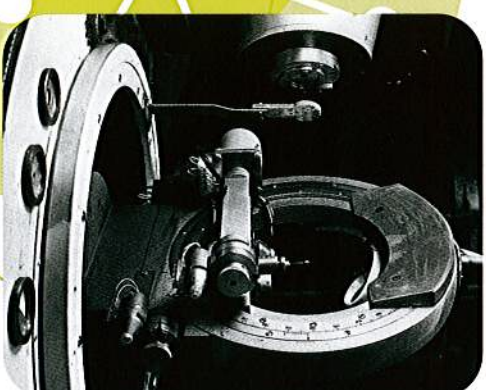
The first computer controlled 4-circle Neutron Diffractometer at HIFAR July/Aug 1972
