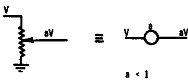
(a) A potentiometer
