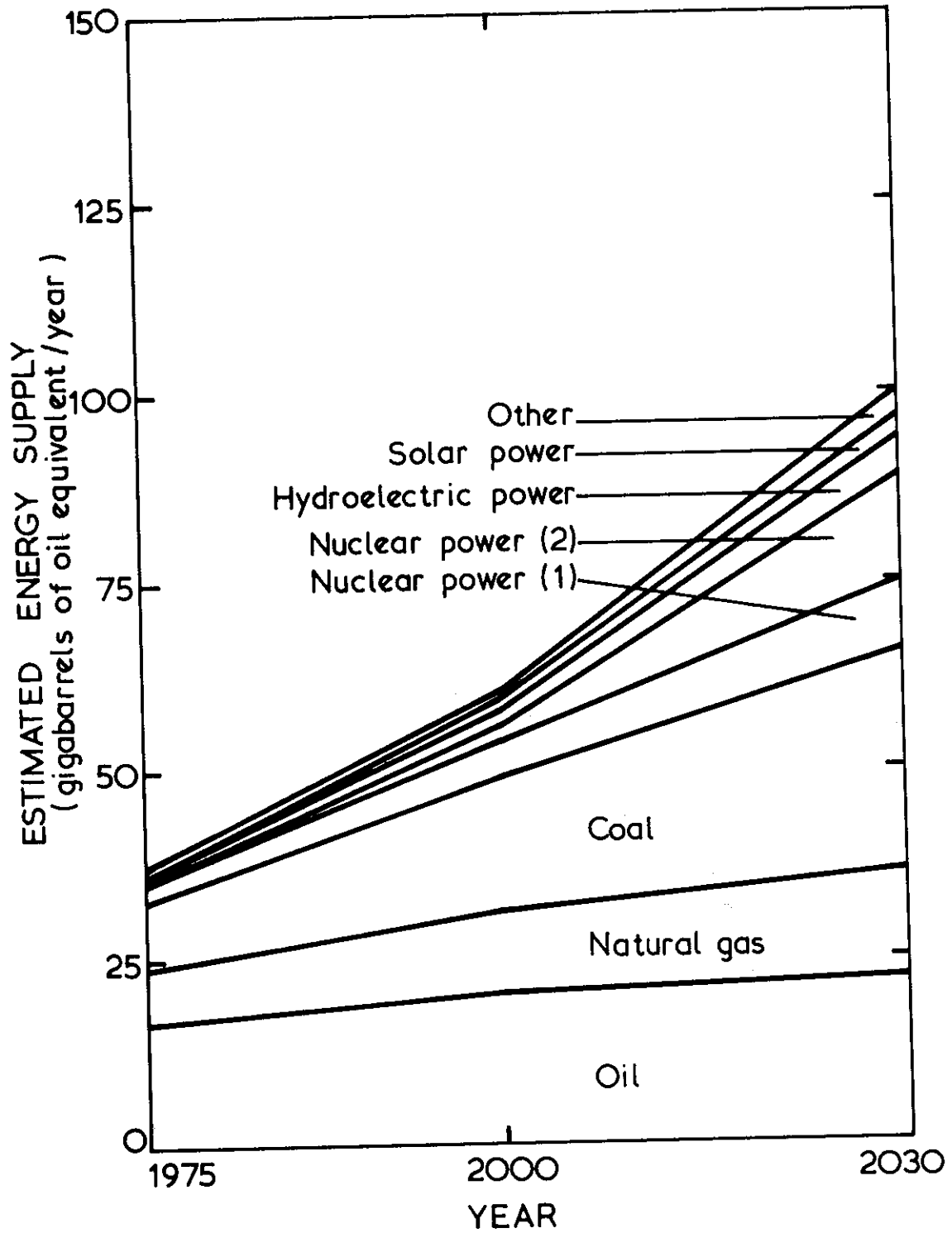
Figure 9.3 Global consumption rate of a variety of primary energy forms according to the low-growth IIASA scenario. [From Sassin 1980].
