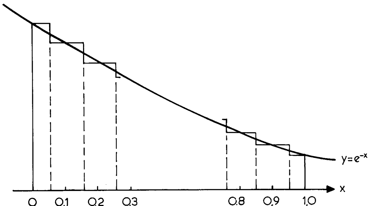
Figure 6.7 A numerical approximation to \int_0^1 e^{-x} dx
