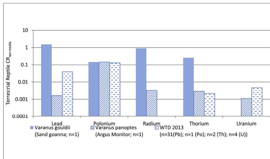
Fig. 3. Comparison of arithmetic mean terrestrial reptile CR_{wo-media} values for two species of goanna Varanus panoptes and Varanus gouldii and the generic reptile value from WTD 2013 (note: the WTD 2013 do not include any Australian reptile data).
