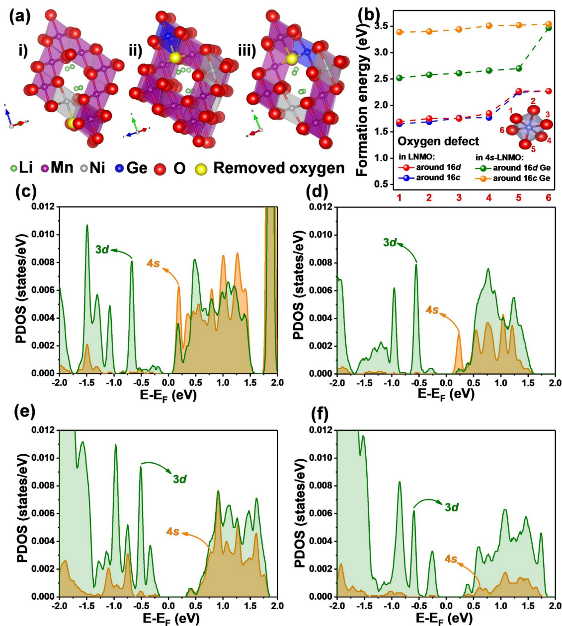
Figure 6. a) Schematic of crystal structures used in E_{\text{f(vac)}} calculations for i) LNMO and modified LNMO with Ge at ii) 16c sites and iii) 16d sites; b) corresponding calculated formation energies of oxygen defects at different parts of the crystal structure, the inset schematically shows the six oxygen sites in an octahedron (dashed lines are guides to the eye); PDOS calculated for structures containing an oxygen vacancy c) next to Ge at a 16c site, d) 10 Å away from Ge at a 16c site, e) next to Ge at a 16d site f) 10 Å away from Ge at a 16d site.
