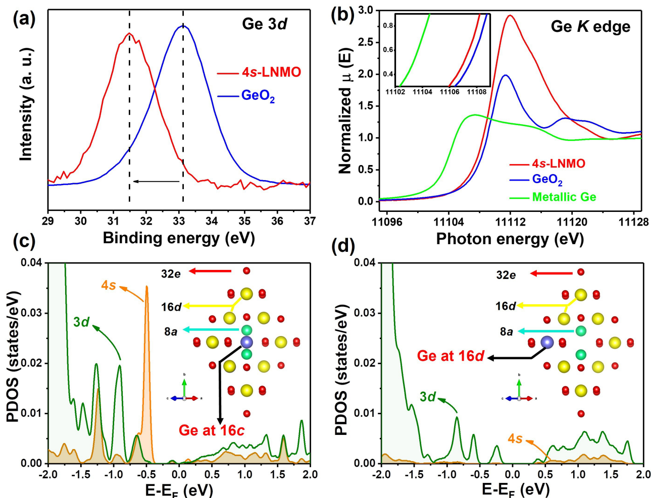
Figure 2. a) Ge 3d XPS data of 4s-LNMO and \text{GeO}_2 ; b) Ge K edge XAS data of 4s-LNMO and reference materials of \text{GeO}_2 and Ge. The inset corresponds to the enlargement of the normalized absorbance from 0.3 to 0.9; projected density of states (PDOS) for the spinel materials with Ge locating at c) 16c and d) 16d site, respectively. The inset in (c) and (d) is a schematic of Wyckoff sites in the spinel-type structure with Fd\bar{3}m space group symmetry shown along the [101] direction.
