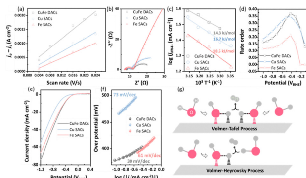
Fig. 4 (a) Capacitive current density as a function of scan rates. (b) EIS spectra. (c) T-dependant j_{\text{NH}_4^+} . (d) Potential-dependent reaction rate order. (e) LSV curve in 0.1 M KOH and (f) corresponding Tafel slope for HER on catalysts. (g) Schematic diagram of the Volmer–Tafel (top) and Volmer–Heyrovsky (bottom) processes on a catalyst surface.
