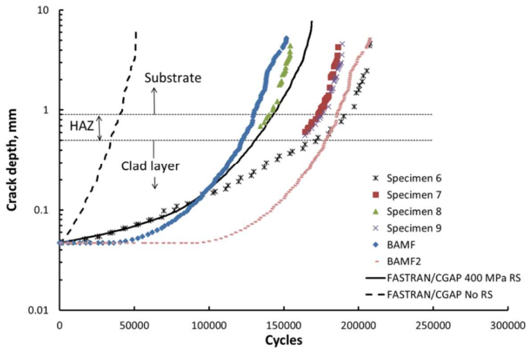
Figure 1. Modelling results for crack propagation through compressive residual stress field in case of laser cladding repair of AerMet®100 steel
