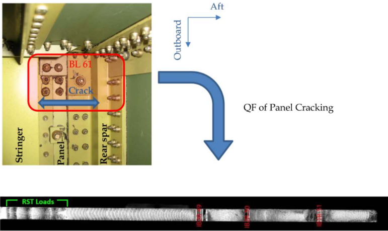
Figure 2. Example teardown location and fracture surface picture ready for QF in the BL 61 region (centre wing to fuselage attachment point at the rear spar cap)
