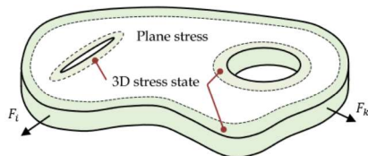
Figure 1. Representation of the exact solution to plane problems of elasticity as a sum of an interior plane stress solution and 3D stress state near boundaries [1].
