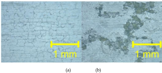
Figure. 2. Micrograph of the graphene coating (a) prior and (b) post corrosion testing
