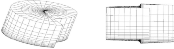
Figure 3. Generation of the coupled fracture mode due to Poisson's effect for a through-the-thickness crack loaded in Mode II [1, 10].
