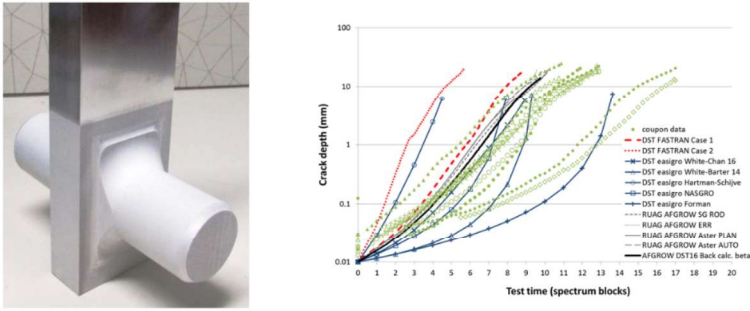
Figure 1. Fatigue test specimen and combined results [2] from first challenge – combat aircraft wing root shear tie (full details can be found on www.govteams.gov.au )
