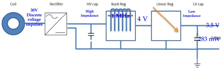
Figure 2. Energy harvester functional block diagram
