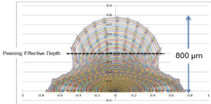
Figure 3. BAMF model after growth through the shot peen RS field
