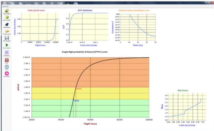
Figure. 3 FracRisk graphical user interface
