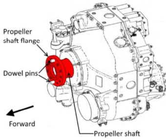
Figure 3. Gear box schematic
