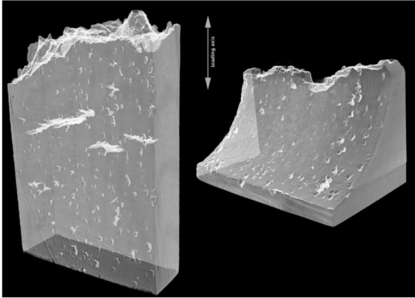
Figure 1. X-Ray synchrotron CT reconstructions of corroded low- k_1 (left) and high- k_1 (right) fatigue specimens of aluminium alloy 7050-T7451. Each specimen is approximately 5 mm wide.
