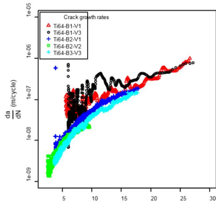
Figure 1. Crack growth rates for the vertically and horizontally built CT specimens of AM Ti-6Al-4V containing numerous lack-of-fusion defects.
