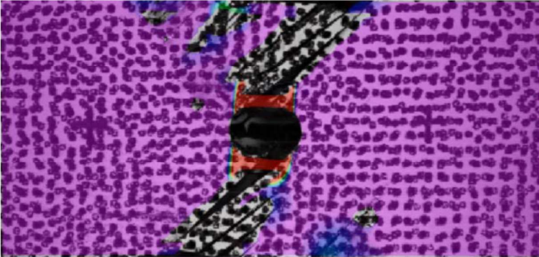
Figure 1. The failure mode of a typical aircraft composite material captured by an ultra-high speed camera at 1million FPS overlaid with surface strain data represented by different colours.
