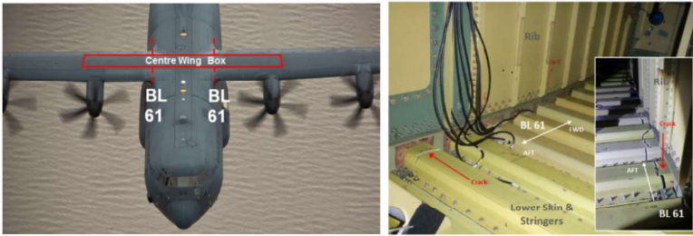
Figure 1. Life Limiting BL 61 region of the C-130J Hercules
