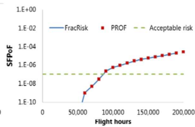
Figure 2. Comparison of FracRisk and PROF results using Gumbel peak stress distribution for C-130J CW-3A location
