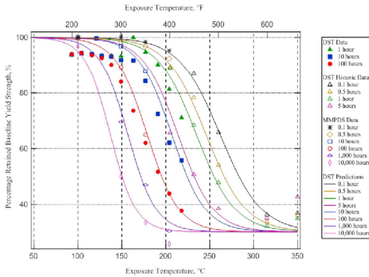
Figure 1. DST Group retained strength model predictions for AA7050 tested against independent data
