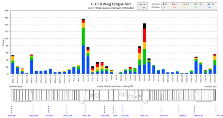
Figure 1. C-130J Wing Fatigue Test teardown centre wing span-wise damage distribution map
