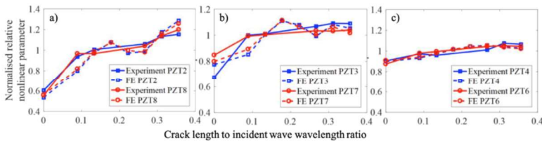
Figure 2. Normalised relative second-order nonlinear parameter as a ratio of the fatigue crack length to the incident wave wavelength of PZTs installed at different locations [3]
