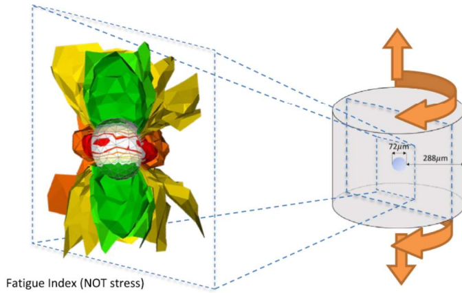
Figure 1. Assessment of fatigue sensitivity around a spherical defect subjected to non-proportional multiaxial loading. Red colours indicate regions of shorter life prediction
