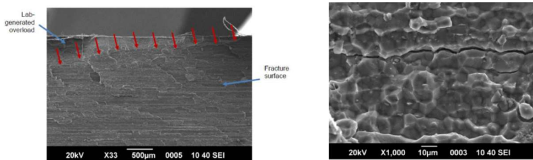
Figure 3. The intergranular nature of the fracture surface
