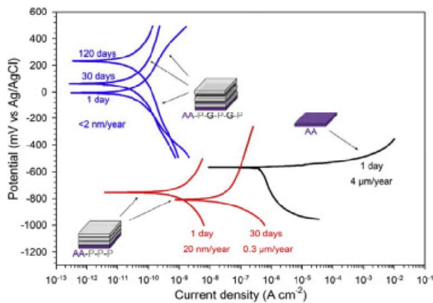
Figure 1. Potentiodynamic scans for various exposure times in NaCl solution
