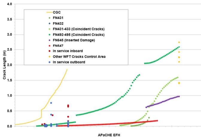
Figure 1. Crack growth modelling versus test cracking and fleet observations
