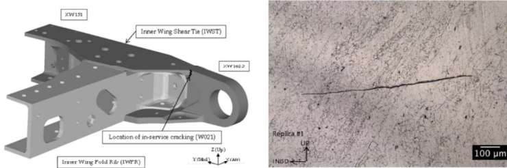
Figure 1. The inner wing aft spar upper flange shear tie radius location (left), and a replica inspection of the 're-cracked' condition of the location prior to shape optimised blend repair (right).
