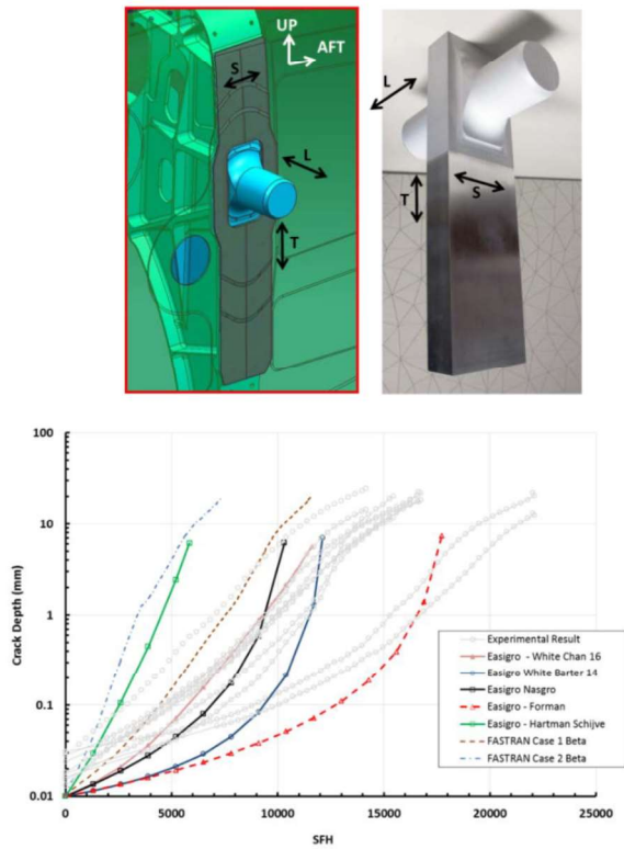
Figure 1. The shear tie post (top), an integral part of a centre fuselage former on a combat aircraft, represented by a symmetric coupon (top right) Note: transverse, long and short relate to plate rolling direction. Blind crack growth predictions compared to coupon quantitative fractography is shown (at bottom).
