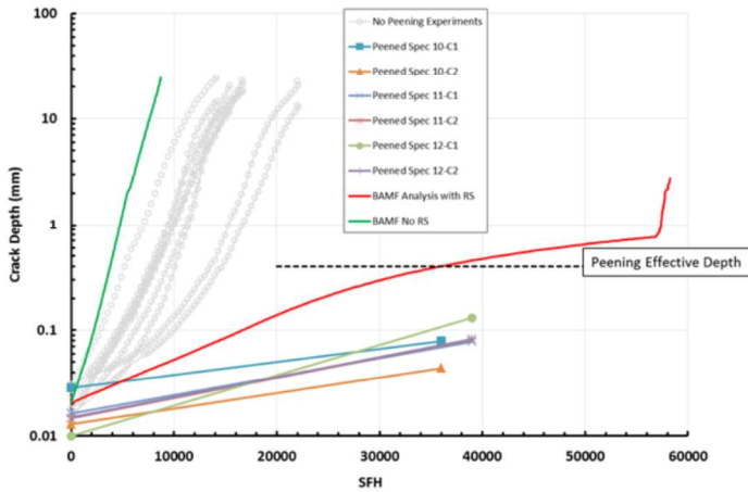
Figure 4. Crack growth predictions vs experiment for with and without shot peening
