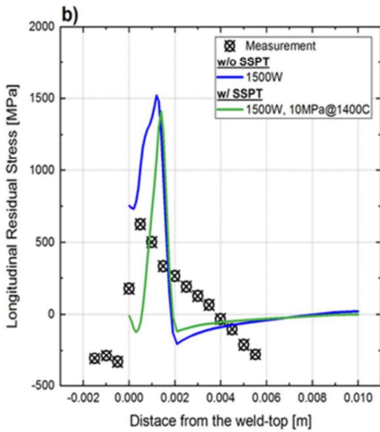
Figure 2. Residual stress profile comparisons, with and without SSPT
