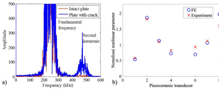
Figure 1a) Experimentally measured signal for incident S_0 guided wave, b) comparison of 3D FE simulations and experimental results [2].
