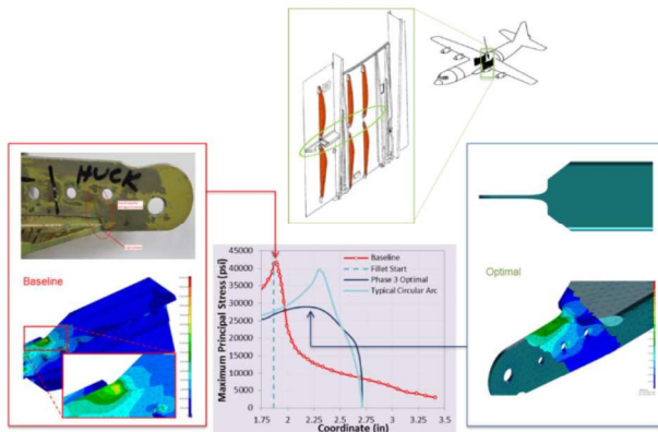
Figure 2. Application of the hypotrochoid-based approach for the design of optimal rework shape of C-130J bow beam runout.
