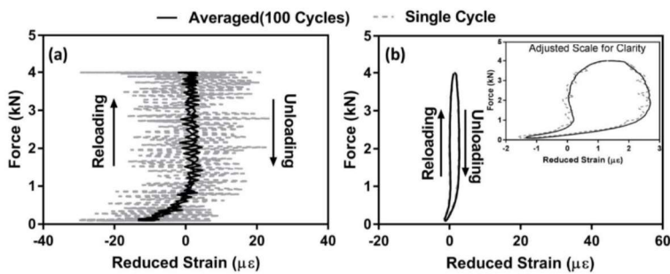
Figure 1. Reduced strain measurements at block 282 where the dashed line is a single cycle and the solid line is averaged over 100 cycles for a) resistive strain gauge and b) piezoelectric strain gauge
