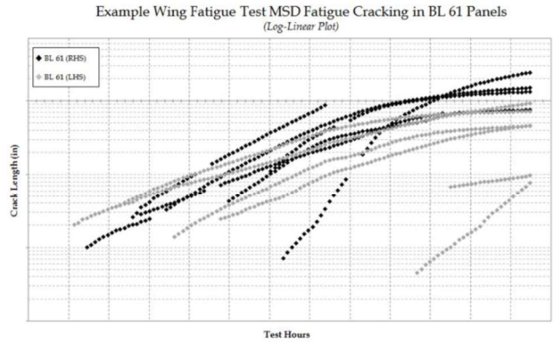
Figure 3. Indicative log-linear crack growth curves determined from QF that underpin Test Interpretation activities
