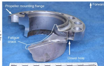
Figure 4. Section of propeller shaft
