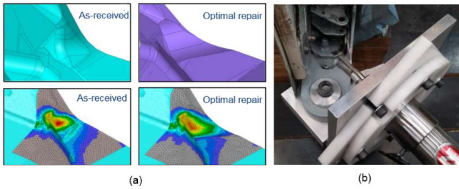
Figure 1. Application of the hypotrochoid-based optimal rework shape design for the recovery of an F/A-18 A/B inner wing shear tie. (a) comparison of geometry and stress at the aft spar shear tie location before and after optimal rework; and (b) In-situ machining, implementing the optimal rework design.
