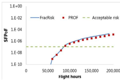
Figure 1. Comparison of FracRisk and PROF results using tabulated stress exceedance data for C-130J CW-3A location
