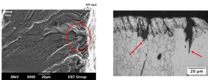
Figure 3. Crack origin below IVD and other etch pits below the IVD layer that could potentially act as crack initiation sites
