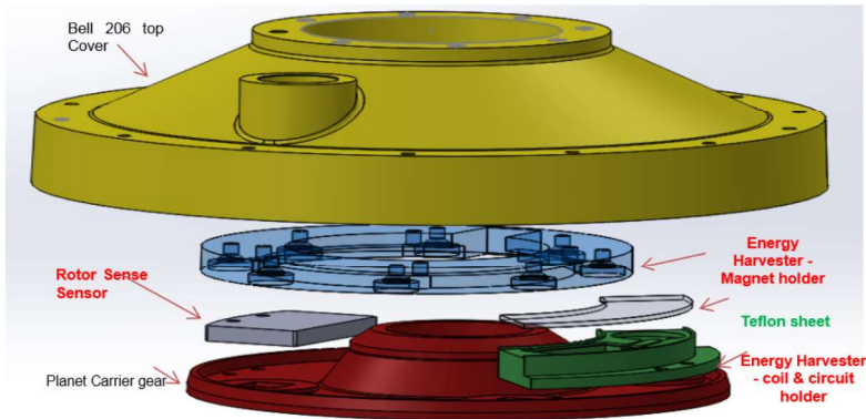
Figure 1. Exploded view in Solid Works for the components of energy harvester to be 3D printed
