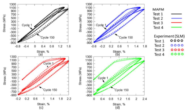
Figure 1. Experimental and computed SLM Ti-6Al-4V first and 150th cycle hysteresis loops for asymmetric strain controlled loading on vertically built specimens (a) {1.6%, -0.8%} (b) {1.8%, -0.6%} (c) {2.2%, -0.2%} and (d) {2.4%, 0.0%}
