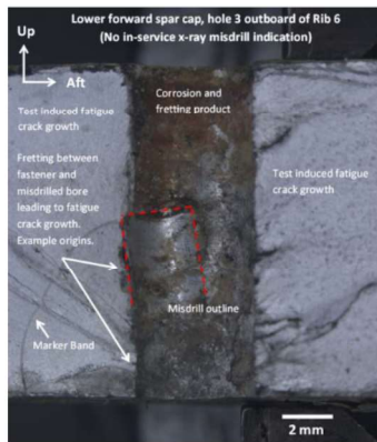
Figure 2. Fractography of the main spar cap primary failure location which contained a mis-drill not identified in-service.
