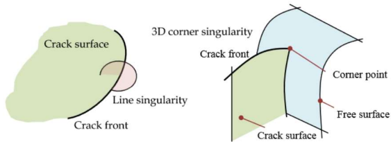
Figure 2. Stress singularities associated with the front of 3D crack [1].
