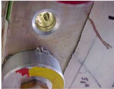
Figure 1. Miss-Drill Damage at Spar Cap Hole
