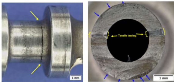
Figure 2. Crack location and fracture surface. Numerous crack origins, with multiple small fatigue cracks having merged to form single crack fronts
