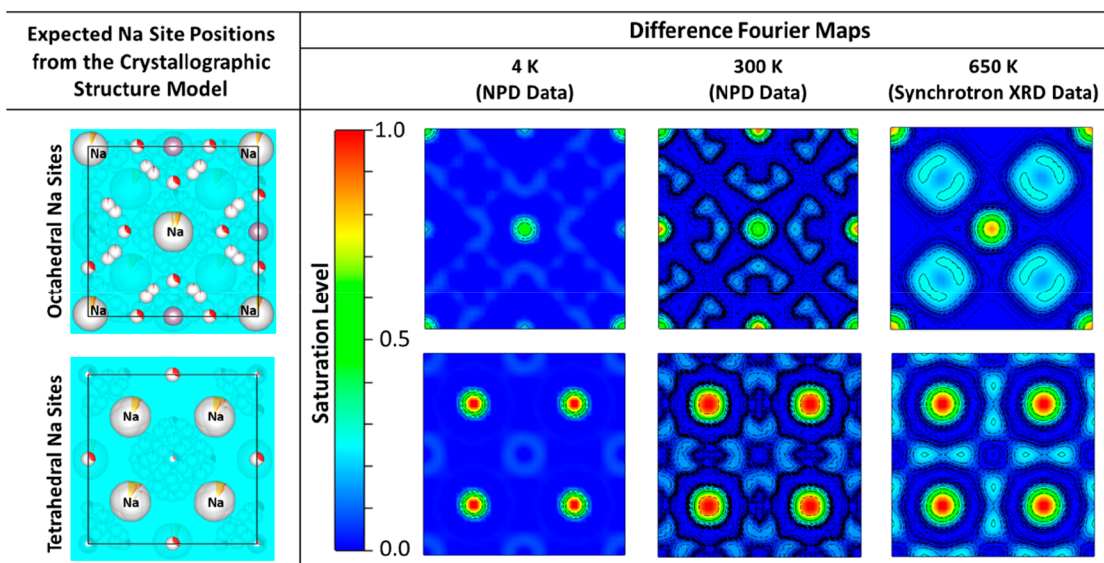
Figure 4. Difference Fourier maps of \gamma\text{-Na}_{2.744}\text{Mg}_{0.128}\text{PO}_4 showing slices through the Na site model positions at 4, 300, and 650 K. The maps were generated from fits of the structural model to the powder diffraction data where all Na occupancies were set to zero. The color scale for the difference Fourier maps shows regions with the greatest difference between the model and data in red and the least difference in blue (NPD data maximum saturation = 0.63; synchrotron data maximum saturation = 3.98).
