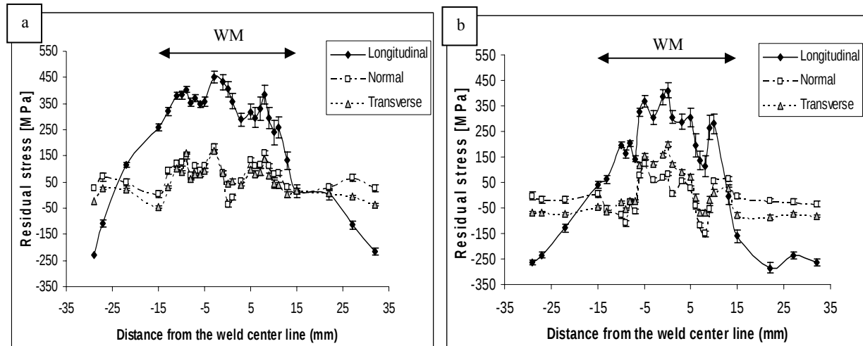
Fig. 2. The longitudinal, transverse and normal components of RS for (a) Sample I and (b) Sample II, measured by ND against distance from the weld center line.
