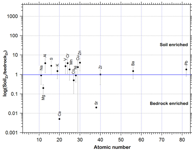
Fig. 2. Soil EF relative to the bedrock material as a function of atomic number, the error bars are one s.d. Values > 1 denote the enrichment of the element in the soil relative to the bedrock and values < 1 indicate depletion in the soil profile relative to the bedrock. For soil and bedrock chemical data see Table A.1 in Supplementary.
