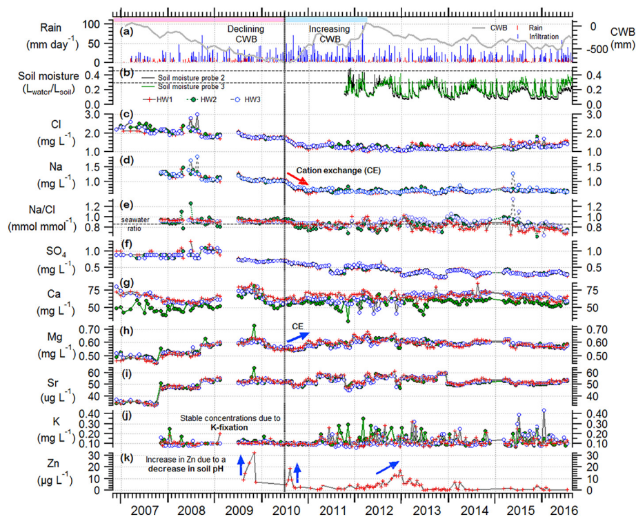
Fig. 3. Time series of (a) daily rainfall, inferred infiltration (Section 3.1) and cumulative water balance (CWB) and (b) soil moisture; the recharge threshold range between 0.30 and 0.45 ( L_{\text{water}}/L_{\text{soil}} ) is indicated by the horizontal dotted lines. Drip water (c) Cl, (d) Na, (e) Na/Cl, (f) \text{SO}_4 (g) Ca, (h) Mg, (i) Sr and (j) K concentration at drip sites HW1 – HW3 and (k) Zn concentration at drip site HW1. The pink and blue coloured bars at the top correspond to a decline and increase in the CWB, respectively and the black vertical line at July 2010 signifies the onset of the wet 2010–12 La Niña event.
