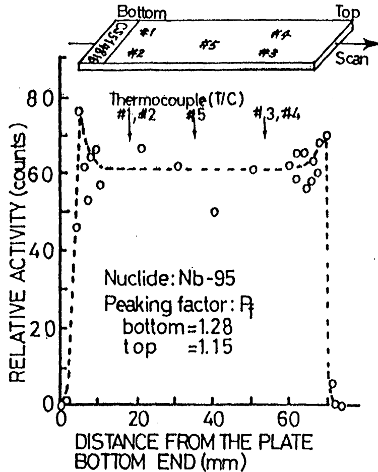
Fig. 2.6 Results of gamma scanning of the silicide plate-type fuel
