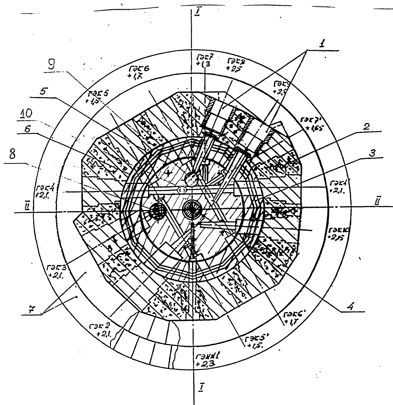
Fig. 4. Layout of arrangement of the experimental beams in the reflector of the PIK reactor.
