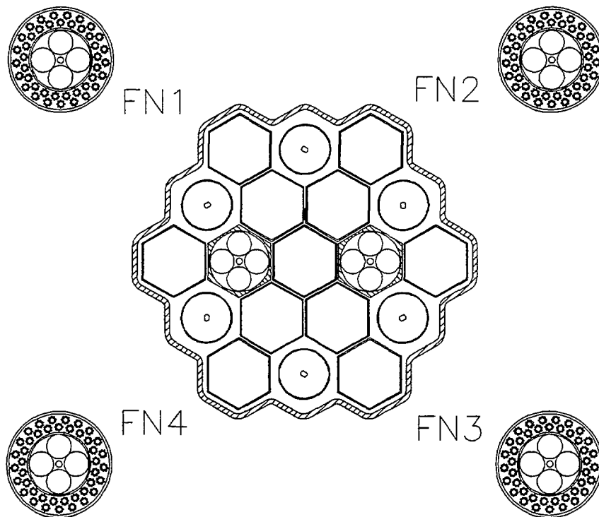
Figure 2: Schematic Representation Of FN-rods Around The MAPLE-MTR Core
