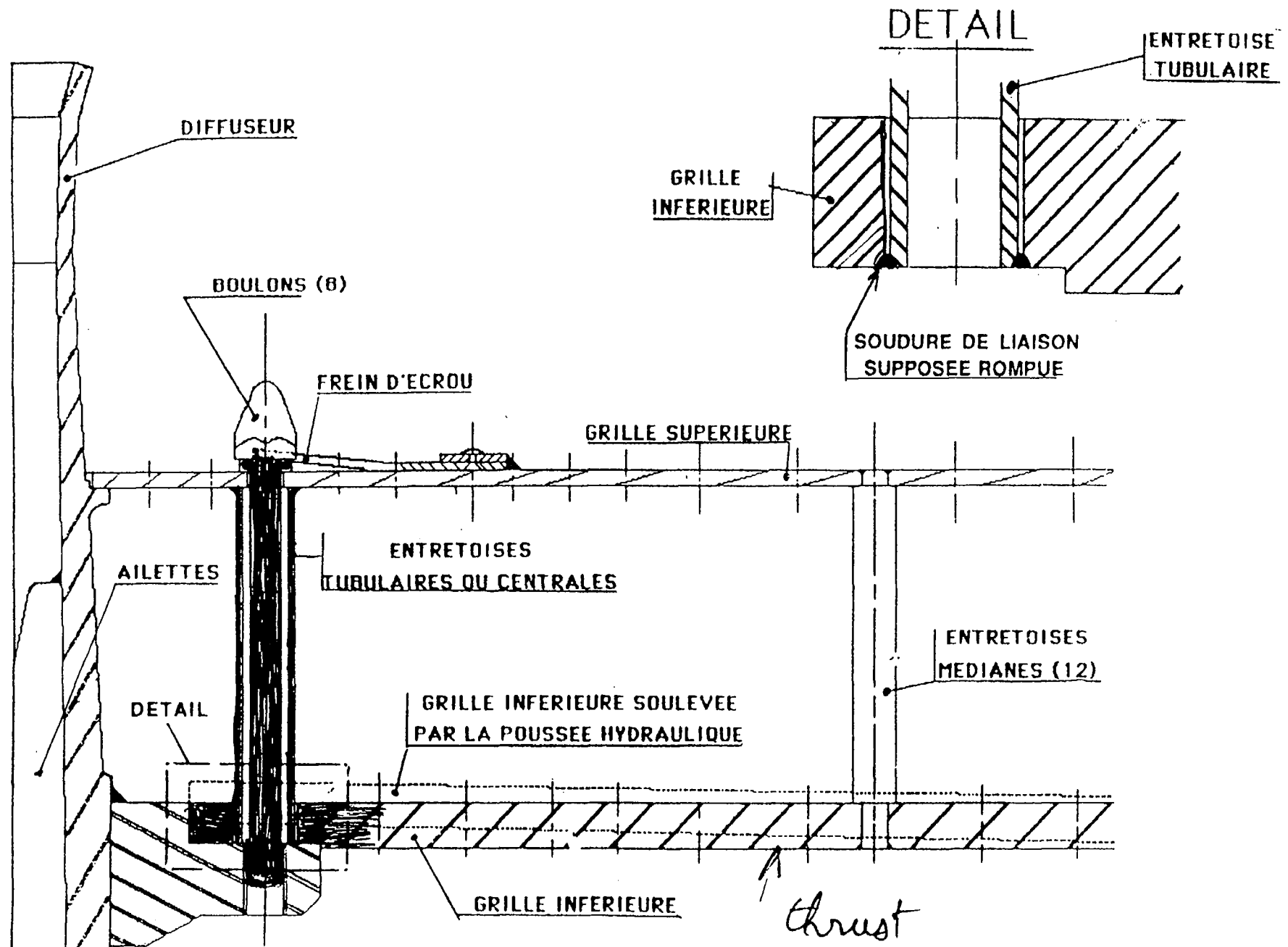
FIG.3 DETAIL DES GRILLES -DETAILS OF THE GRIDS
