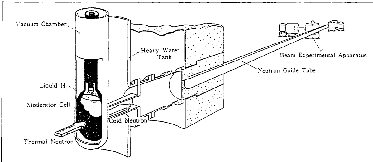
Fig. 2 General Description of Moderator Cell of JRR-3M CNS Facility
