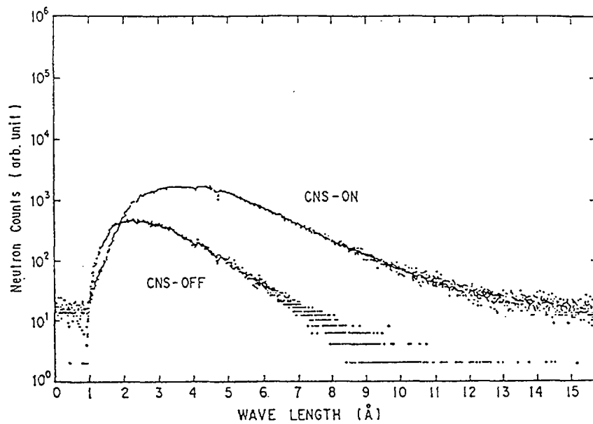
Fig. 4 Comparison of Neutron Spectra at the End of the Cold Neutron Guide tube C2 when the CNS was Operated (CNS-ON) and the CNS was not Operated (CNS-OFF)
