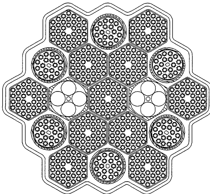
Figure 1: Schematic Representation Of The MAPLE-MTR Core
