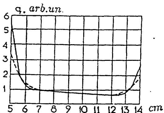
Fig. 12. Distribution of energy output in medial plane along PIK-04 core.
