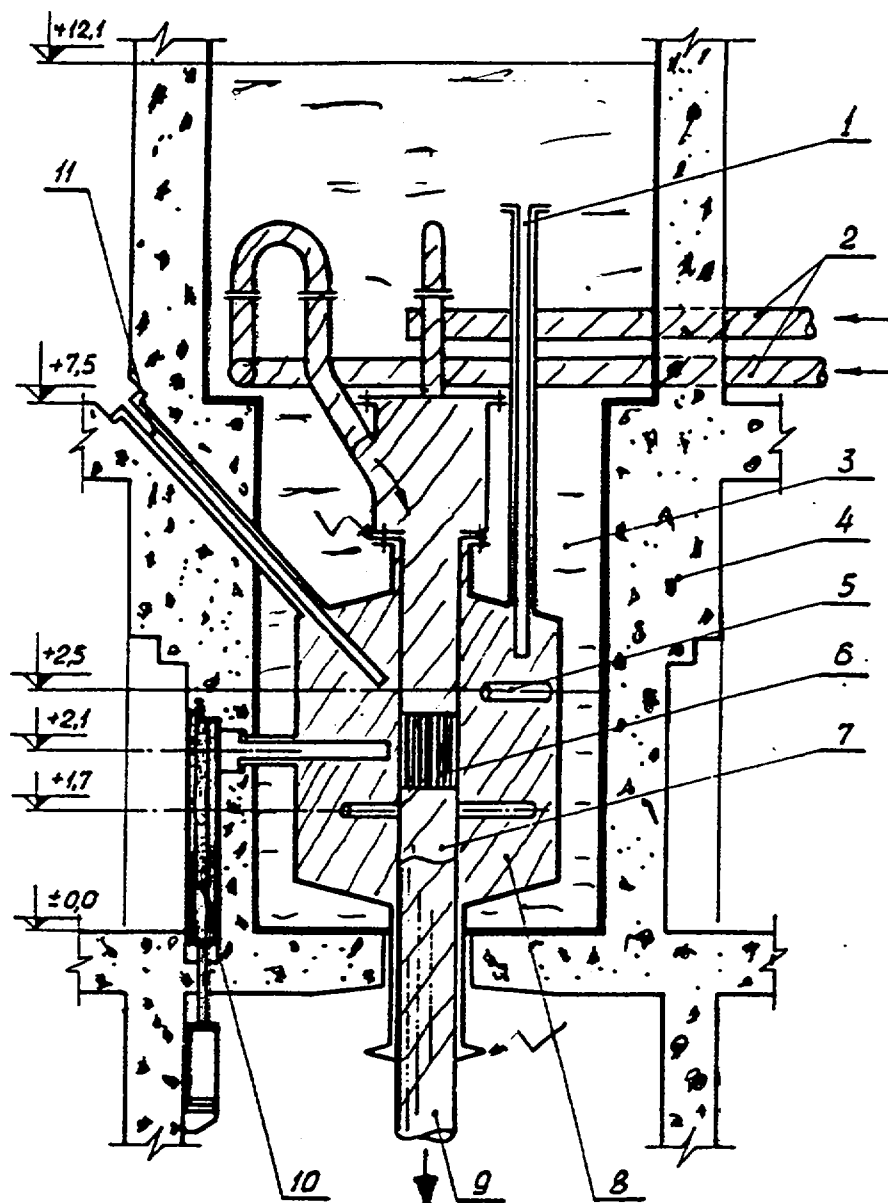
Fig. 3: Schematic vertical section of the PIK reactor.
