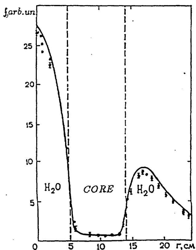
Fig. 13. Fission rate as a function of the radius critical assembly. Continuous line - calculated values. Points - experiment.
