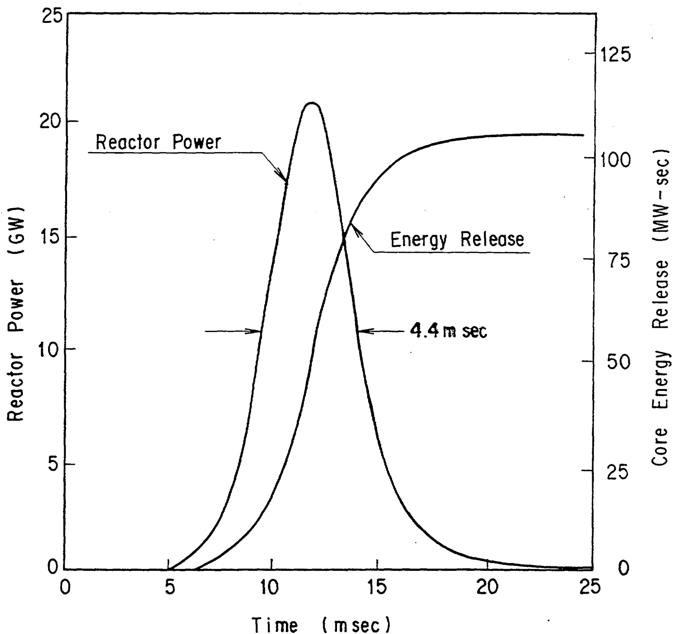
Reactor Power and Core Energy Release Histories Obtained by 4.67S Pulse Operation in the NSRR
