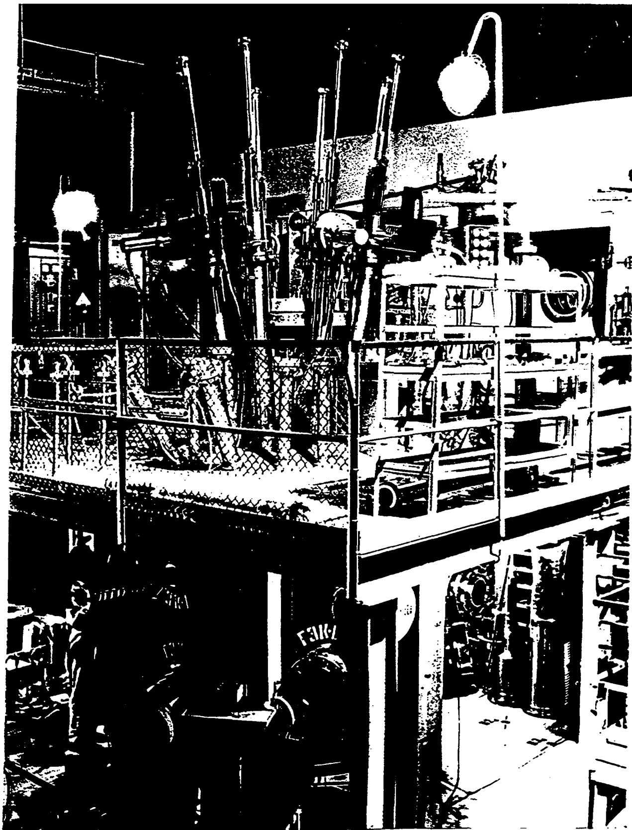
Fig. 9. Mock - up of PIK reactor ( 100 W).
