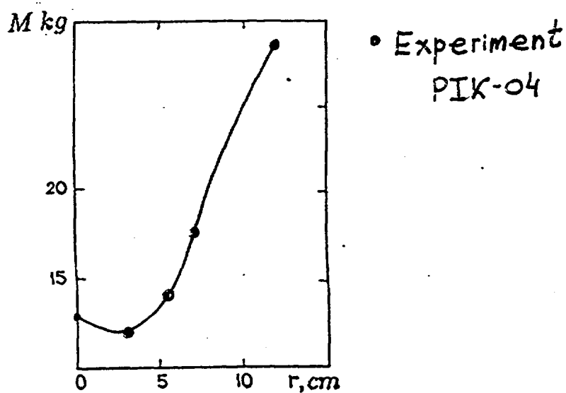
Fig. 11. Critical mass M as a function of r - radius of the inner light-water trap. Continuous line - calculated values. Points - experiment (error is less than the points dimensions).
