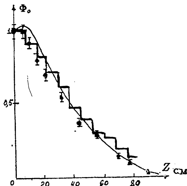
Fig. 14. Distribution thermal flux density \Phi_0 (in respect to I ) along Z direction of beam tube \Gamma\Theta K - 1 .
