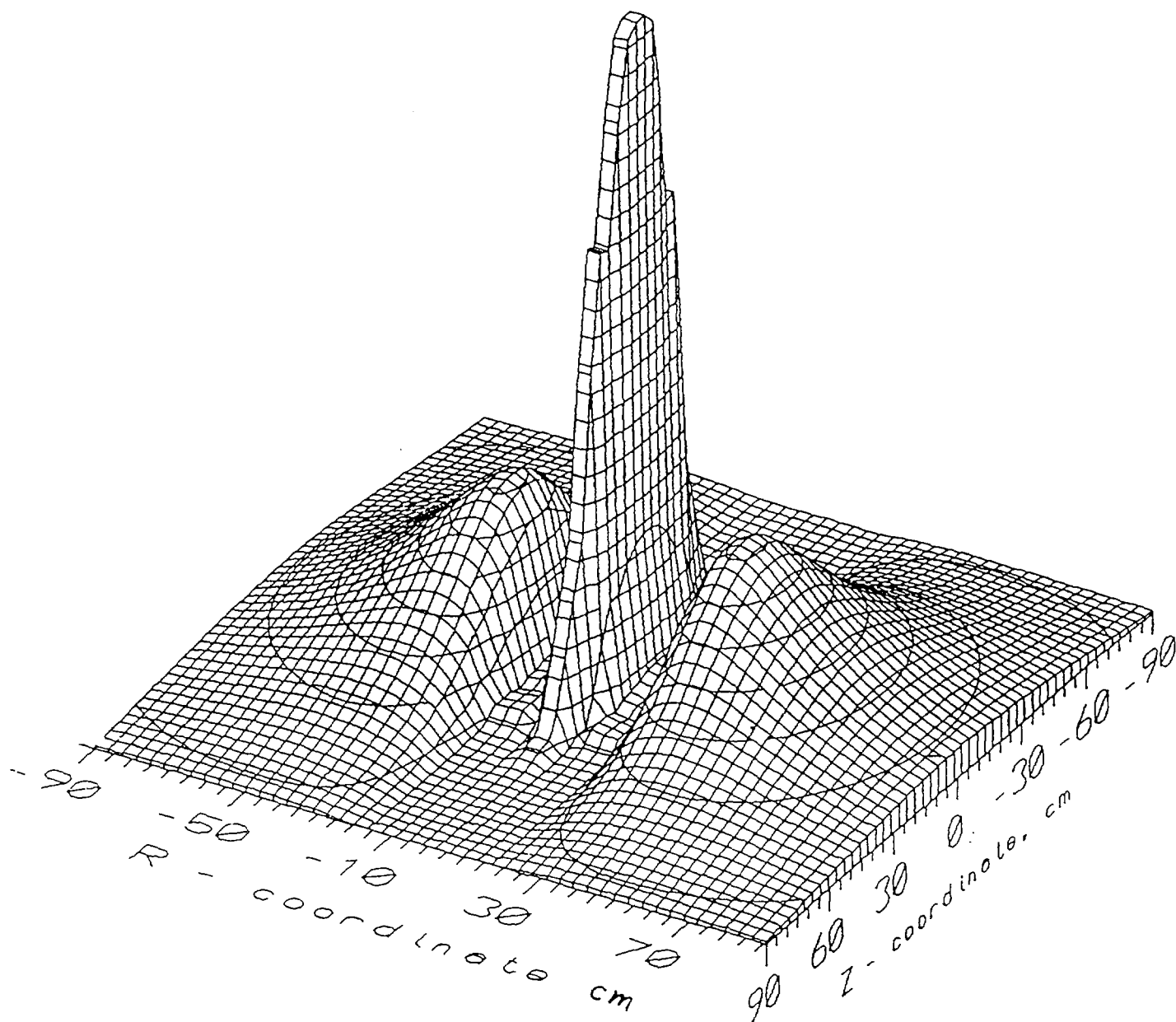
Fig.11: Distribution of unperturbed flux of thermal neutrons in the middle plane of the core
