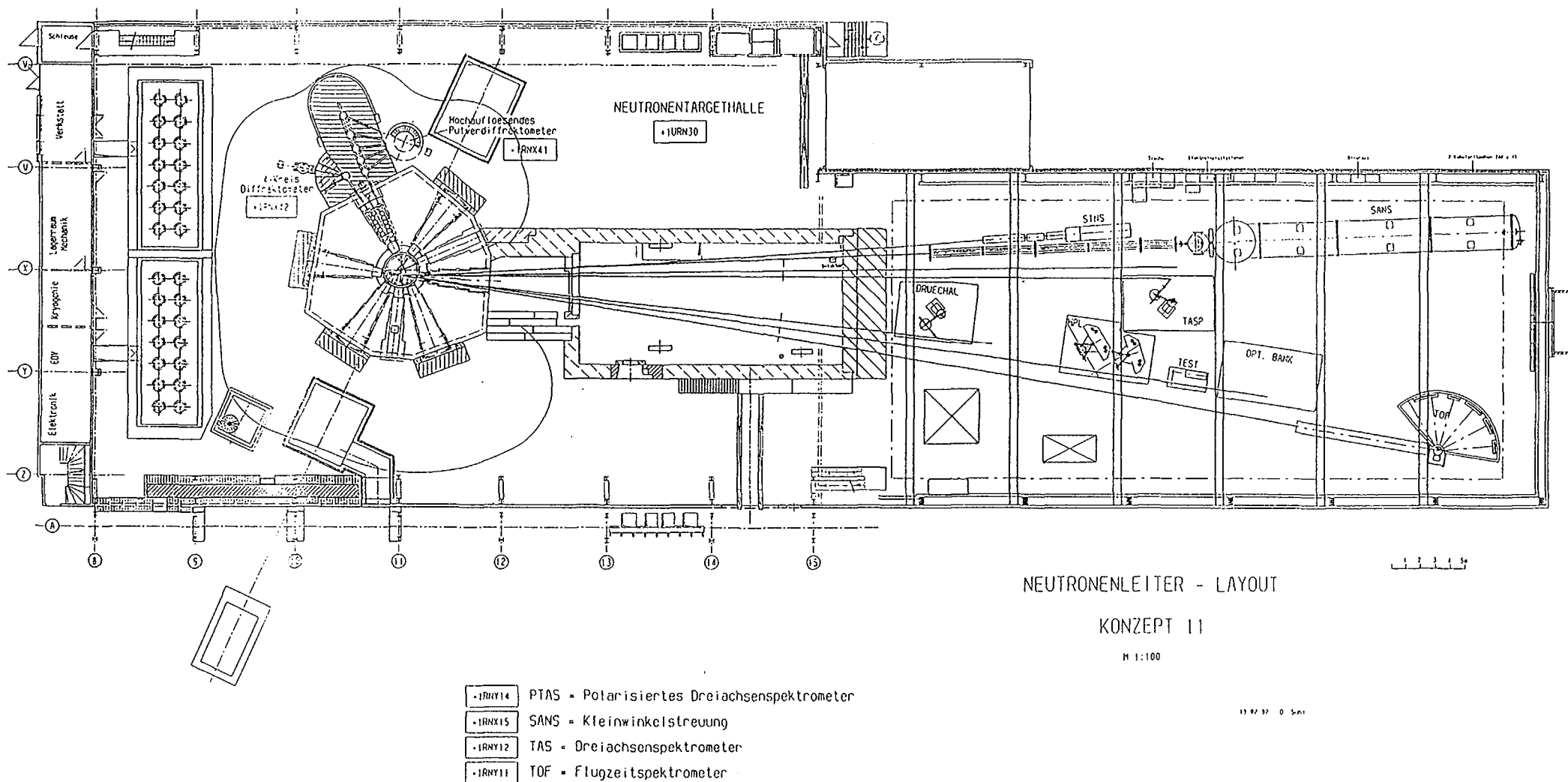
Fig. 4 Floor plan of the SINQ target and neutron guide halls showing the presently projected suite of instruments.
