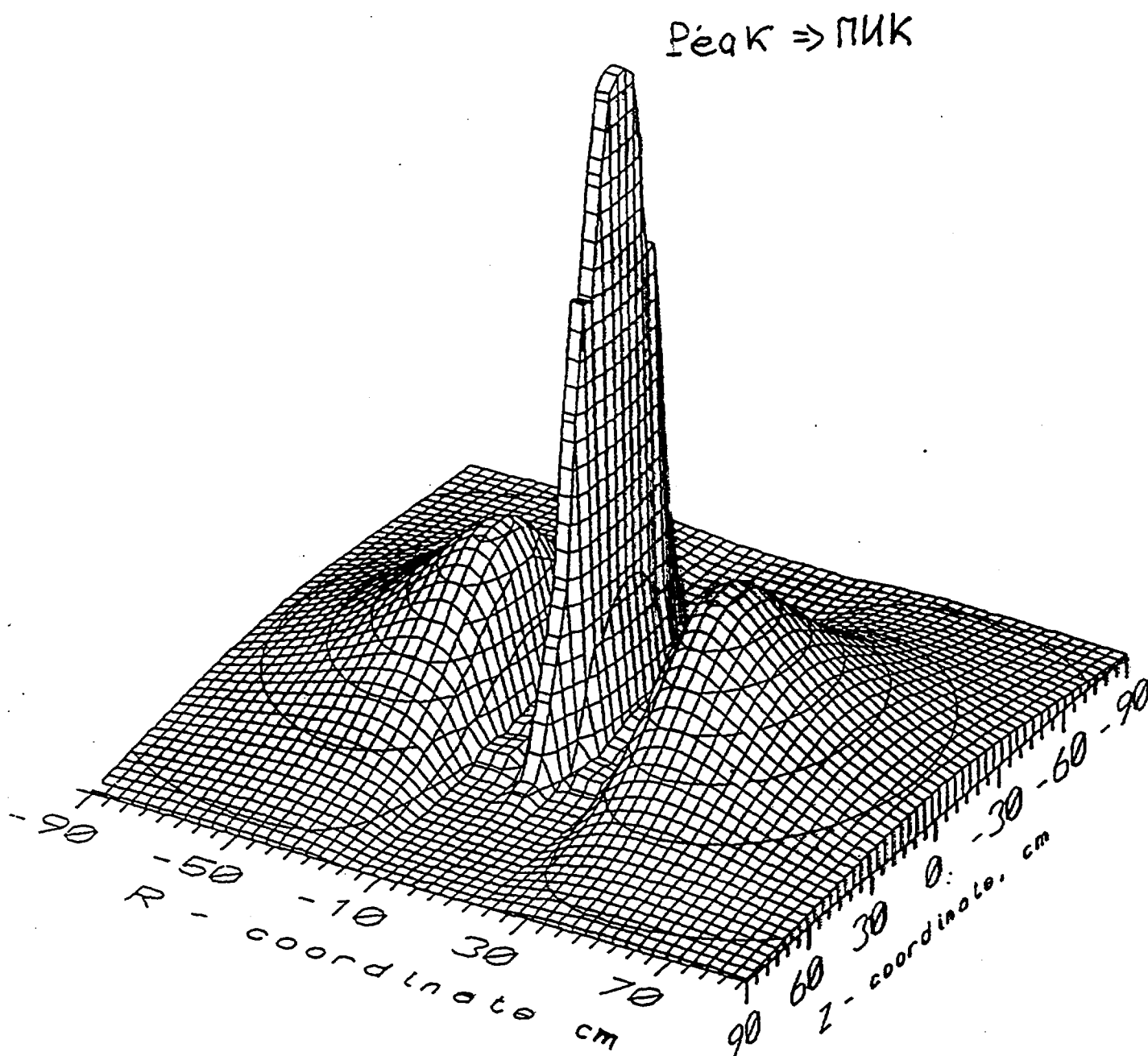
Fig. 16. Distribution of unperturbed flux of thermal neutrons along PIK reactor.
