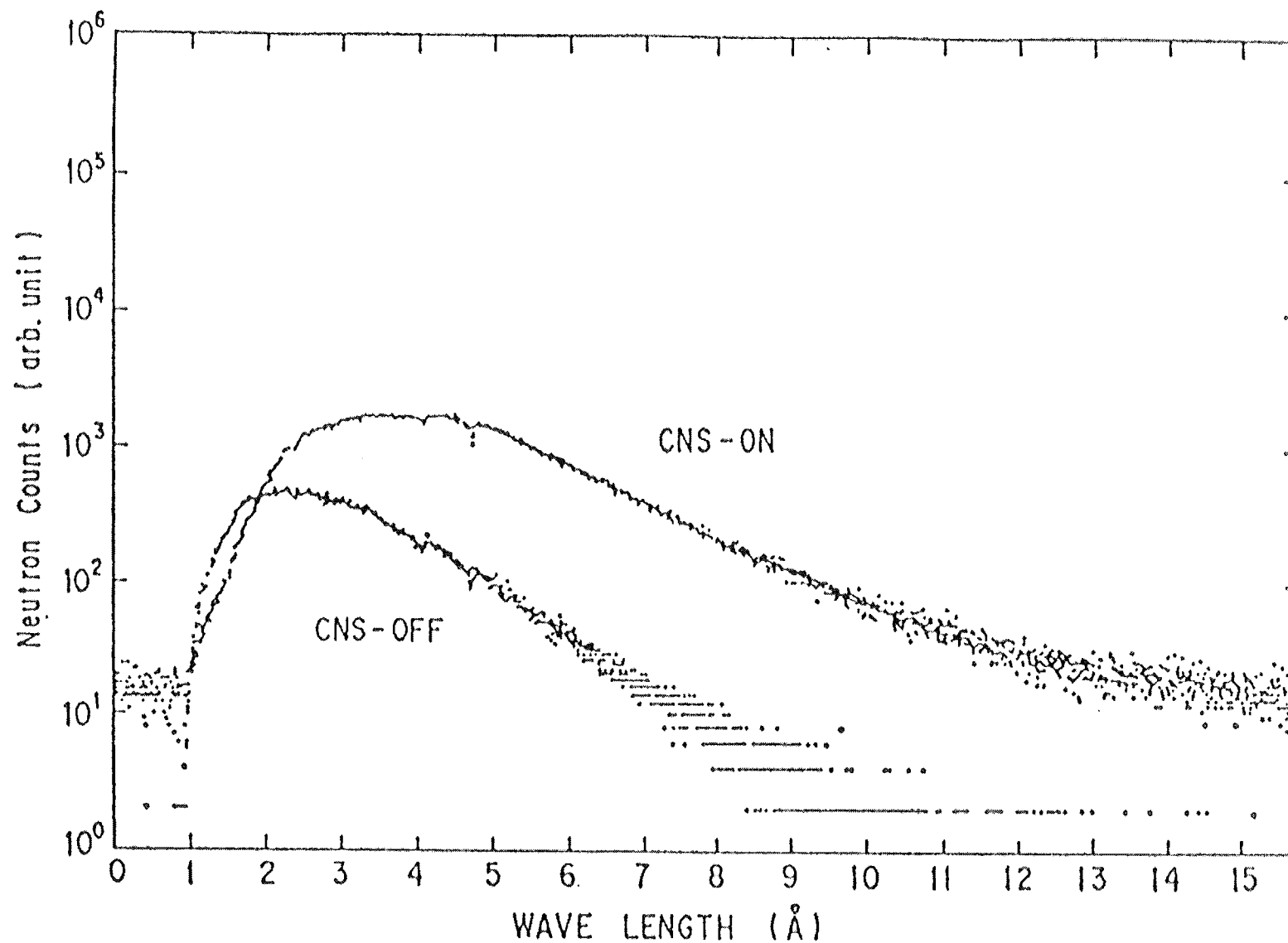
Fig. 4 Comparison of Neutron Spectra at the End of the Cold Neutron Guide tube C2 when the CNS was Operated (CNS-ON) and the CNS was not Operated (CNS-OFF)
