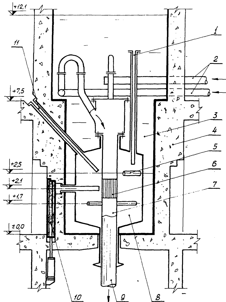
Fig.3: Schematic vertical section of the PIK reactor.
