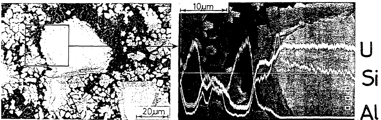
Photo.1 XMA Linear Analysis against the Agglomerations of Si, U, and Al
