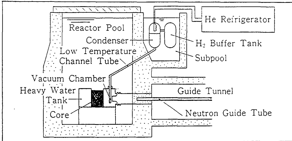
Fig. 1 The Schematic Diagram of JRR-3M CNS Facility
