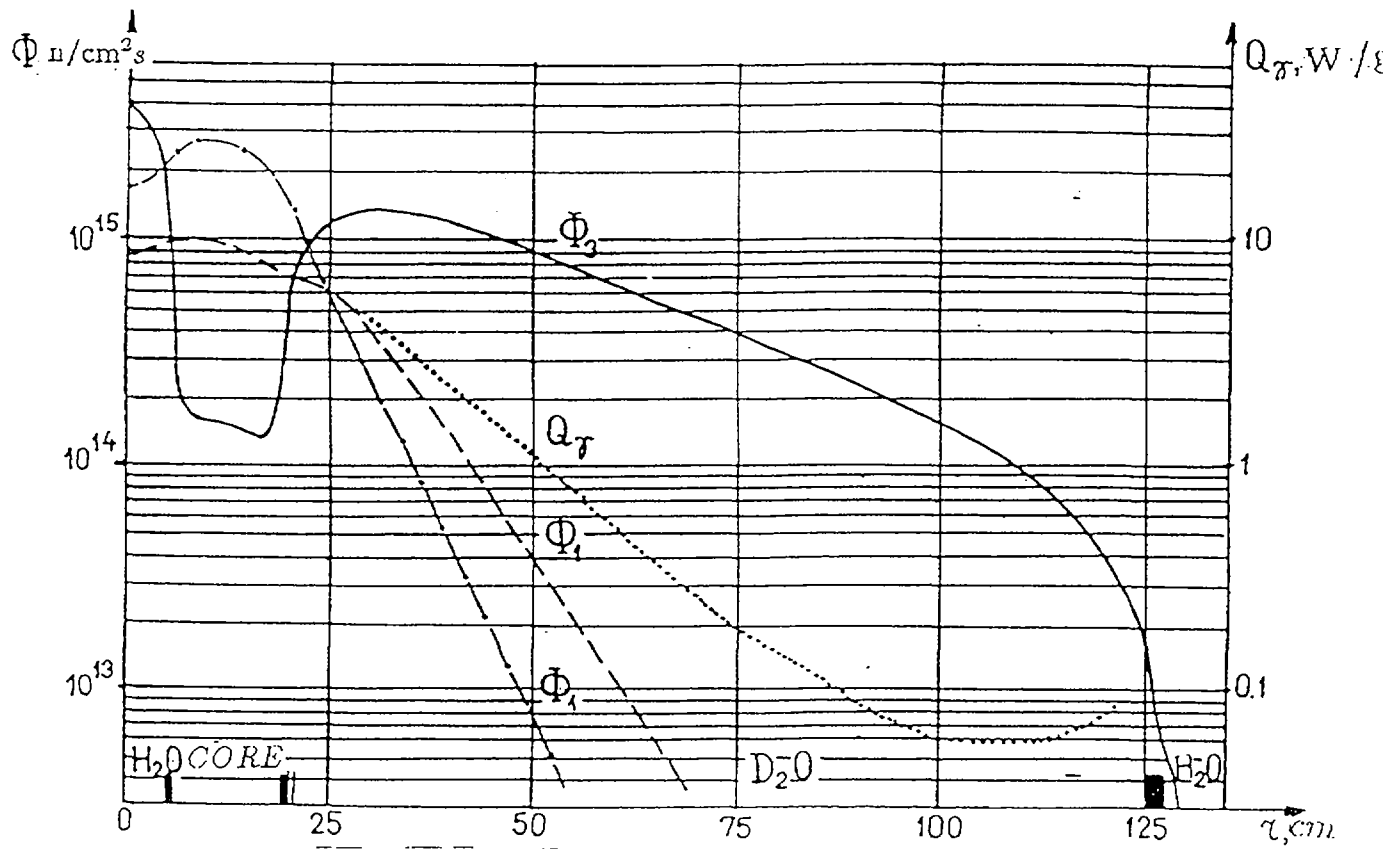
Fig.6: Distribution of unperturbed neutron flux \Phi and energy output Q_\gamma for 100 MW reactor power. \Phi_1 - fast neutron flux E > 5 \text{ keV} ; \Phi_2 - epithermal neutron flux 5 \text{ keV} > E > 0.6 \text{ eV} ; \Phi_3 - thermal neutron flux E < 0.6 \text{ eV}
