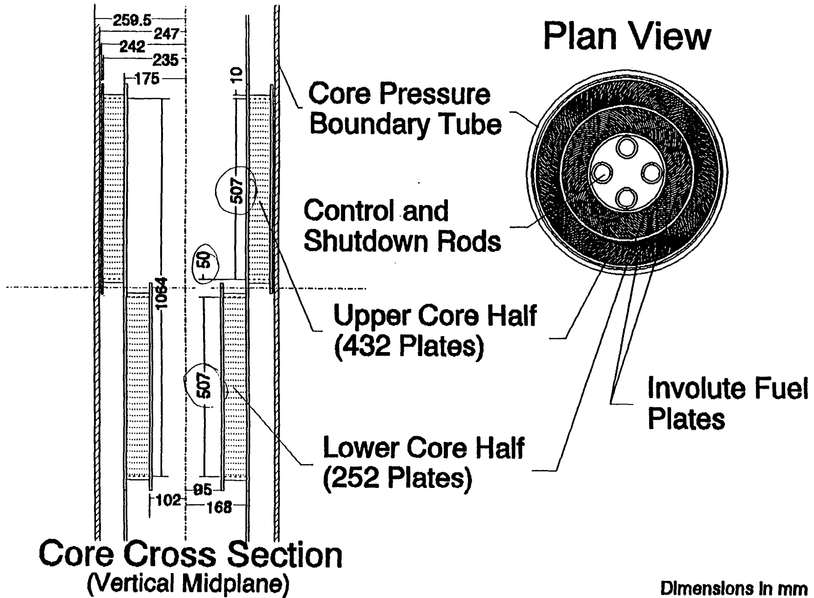
Dimensioned Core Drawing
