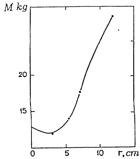
Fig.9: Critical mass M as a function of radius r of the inner light water trap. Full line: calculated values; dotted: experiment (error smaller than point size).
