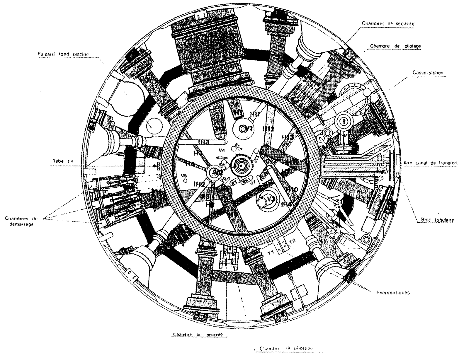
FIG.5 HORIZONTAL VIEW OF THE POOL
