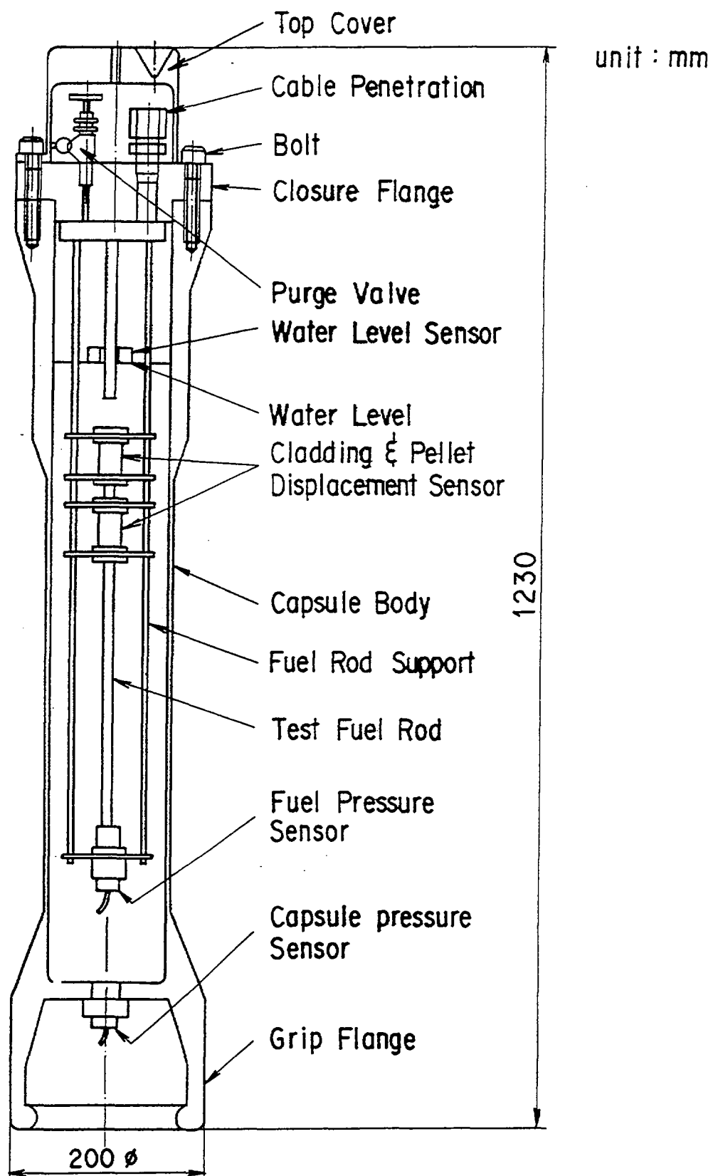
Standard Water Capsule
