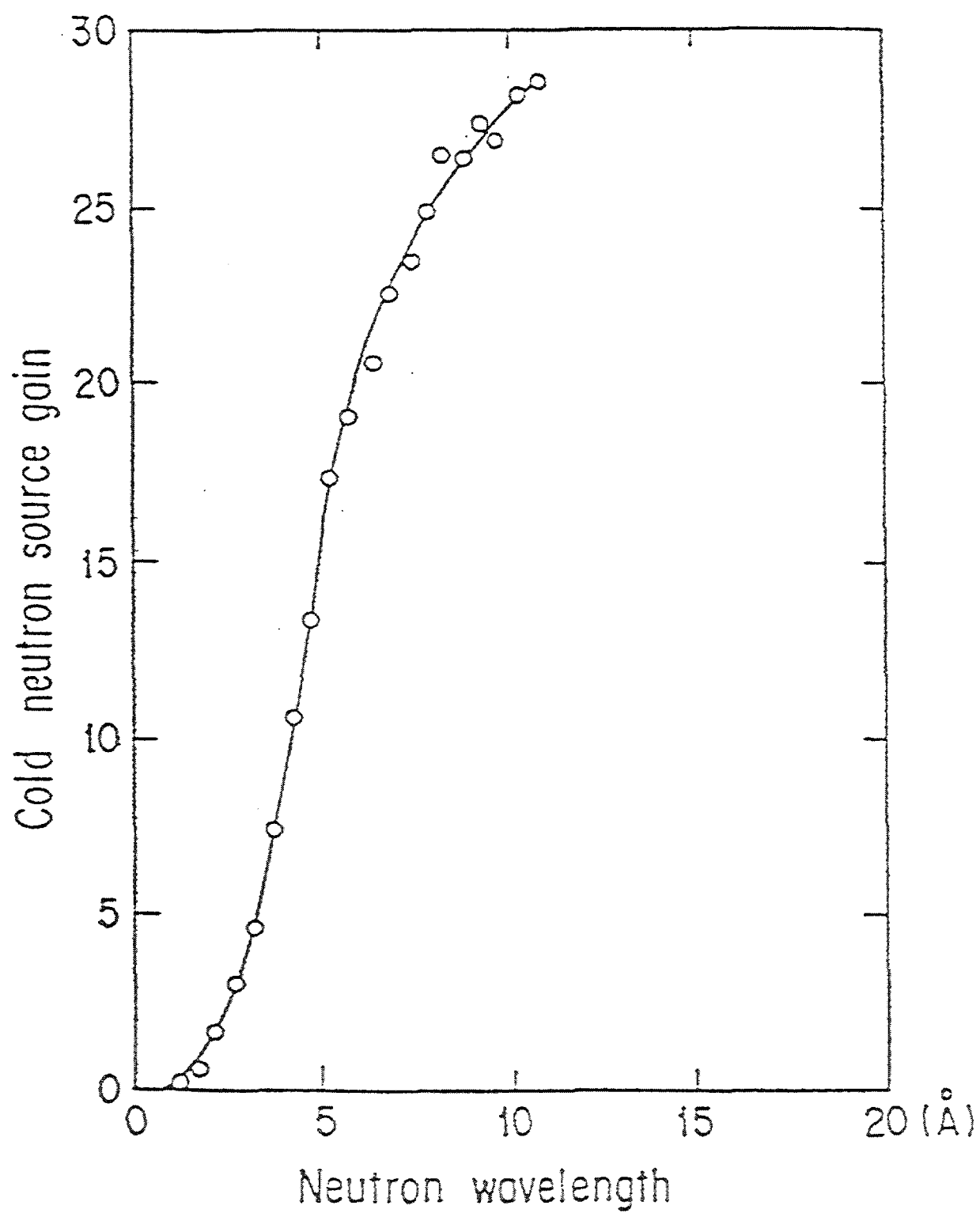
Fig. 5 The Cold Neutron Source Gain
