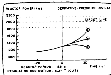
Figure 5. Limited-Derivative, Current, and Predictive Information (Scheme V)
