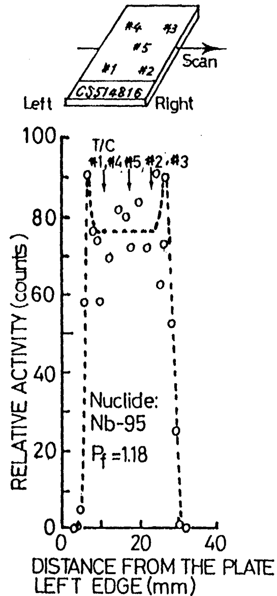
Fig. 2.6 Results of gamma scanning of the silicide plate-type fuel
