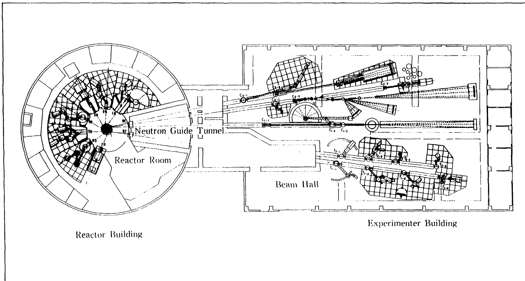
Beam Experimental Facilities
