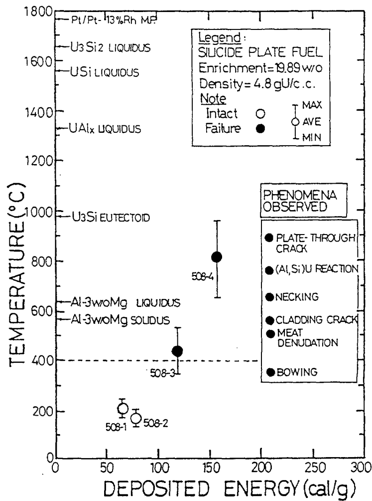
Fig. 3 Temperature of the Silicide Fuel Mini-plate as a Function of Deposited Energy by Pulse Irradiation
