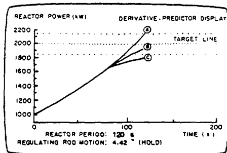
Figure 4. Derivative, Current, and Predictive Information (Scheme IV)
