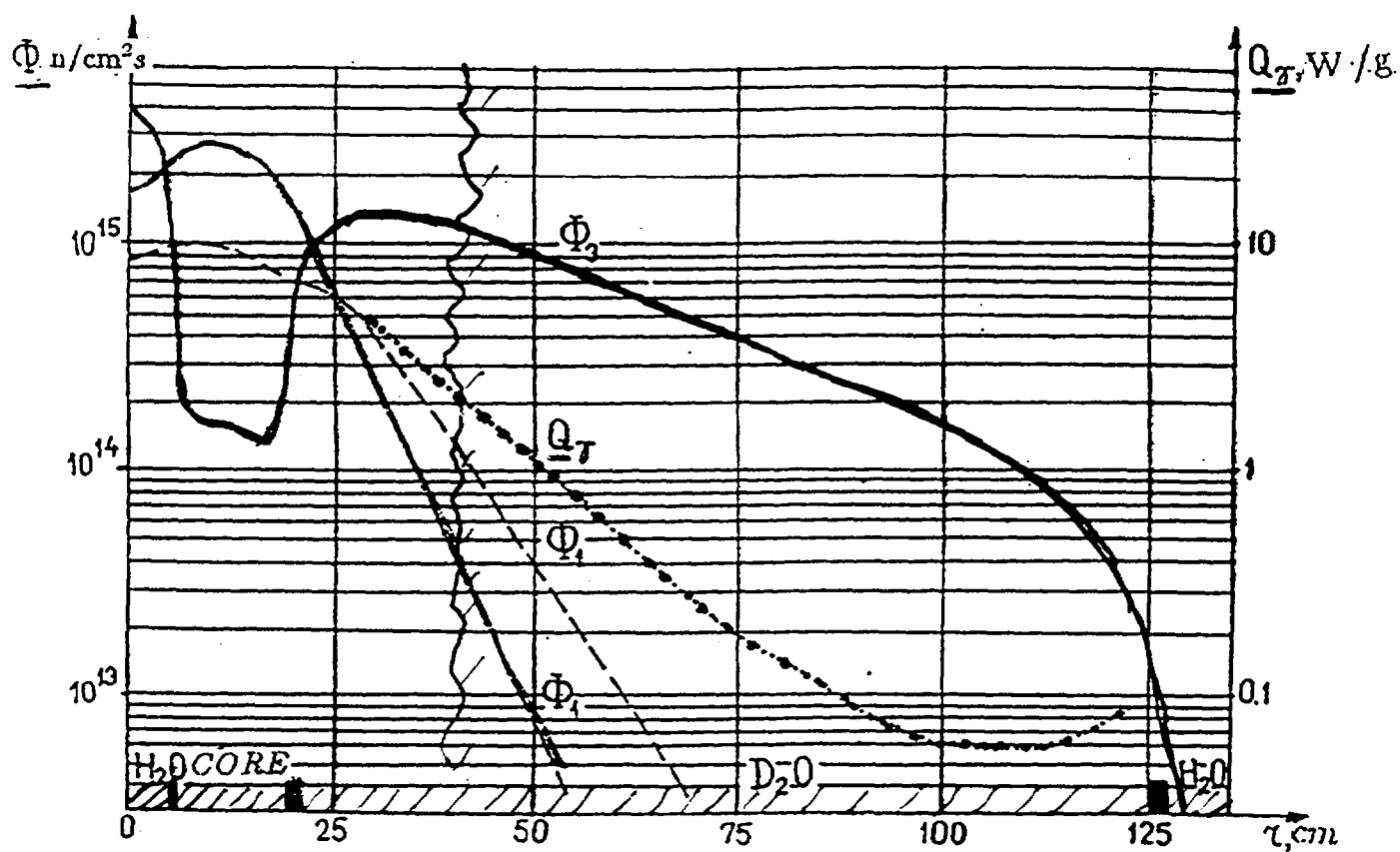
Fig. 6. Distribution of unperturbed neutron flux \Phi and energy output Q_T for 100 MW reactor power.
