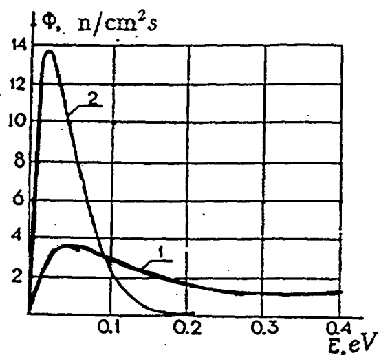
Fig. 10. Spectrum of thermal neutrons \Phi(E) . 1 - in PIK-04 core; 2 - in the water at 293K. \Rightarrow 2 overlapping thermal groups
