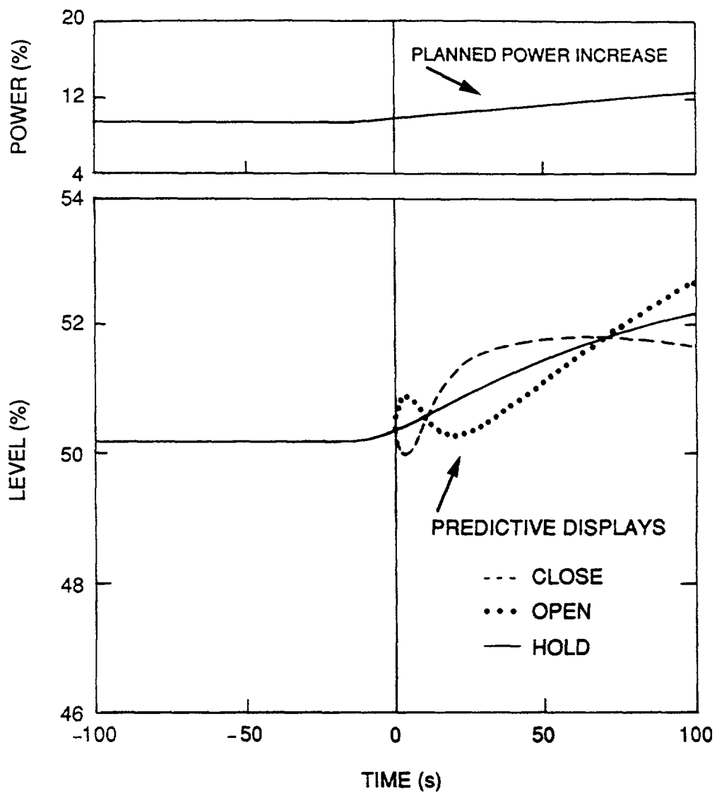
Figure 8. Steam Generator Level Display After Start of Power Ramp with Ramp Rate of 2.5% of Full Power Per Minute with Reactor Initially at 10% of Rated Power
