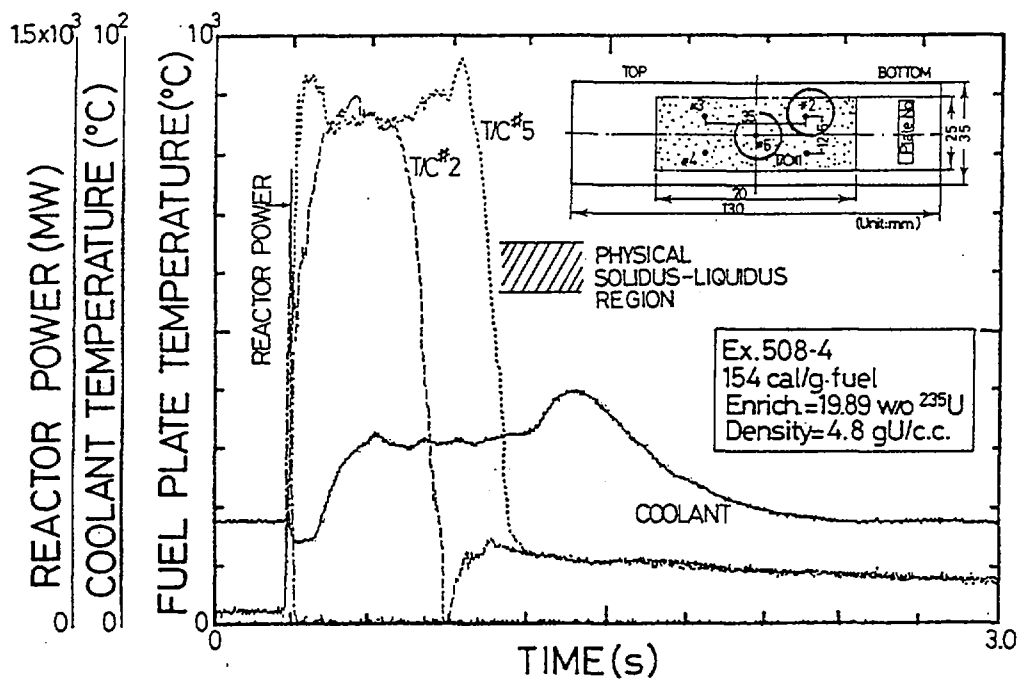
Fig. 2 Time-dependent Change of Fuel Plate Surface Temperatures, Coolant Temperature and Reactor Power in Test #508-4
