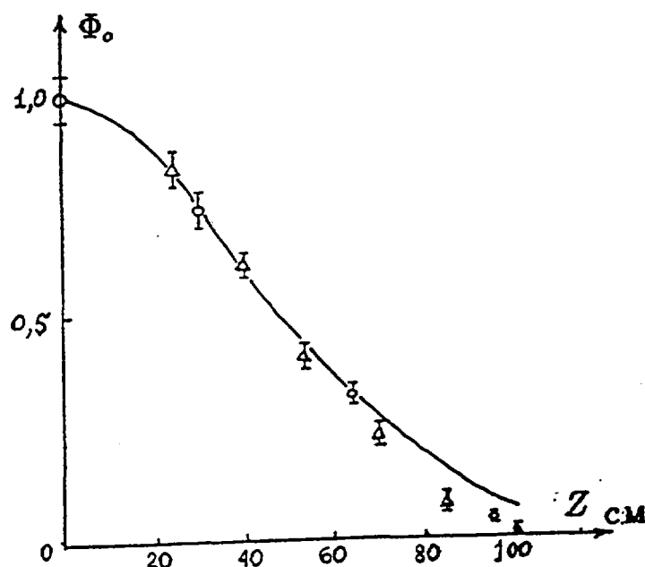
Fig. 15. Distribution thermal flux density \Phi_0 (in arbitrary units) along Z direction of beam tube \Gamma\Theta K - 4 .
