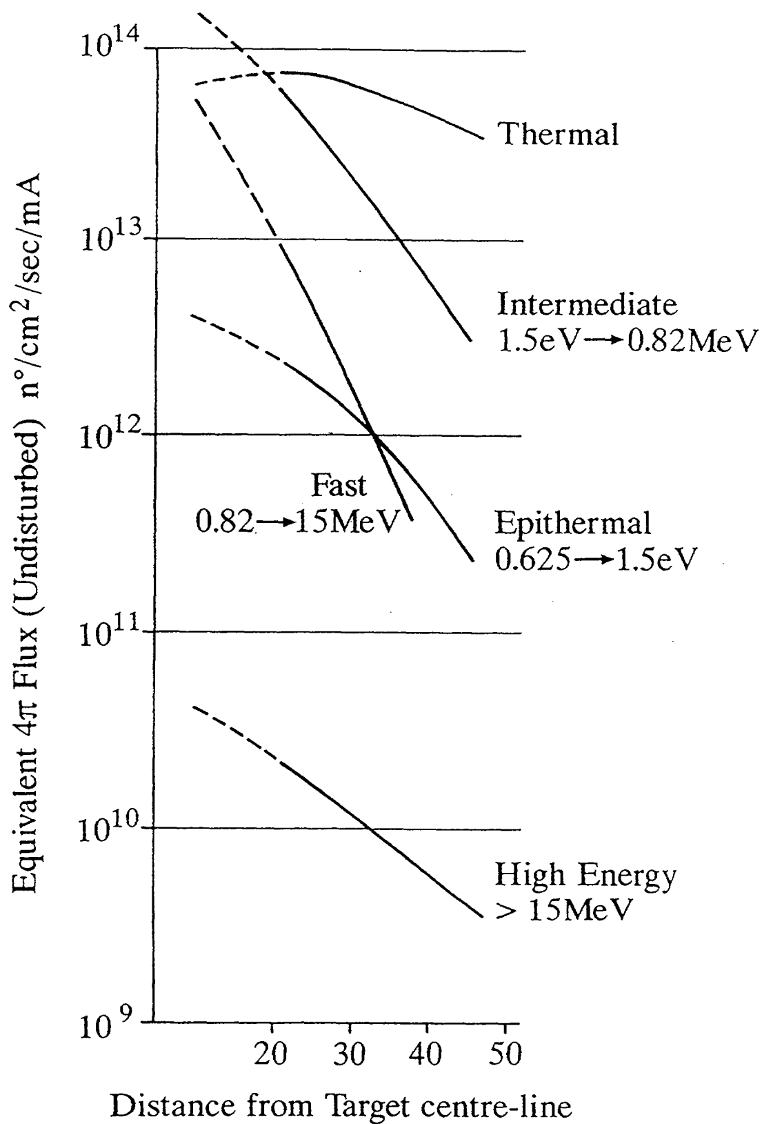
Fig. 3 Flux distribution for various energy groups in the \text{D}_2\text{O} moderator for a Pb-Bi target with steel container. The flux depression caused by absorption in the steel is clearly visible for the thermal group. (after ref. 11)
