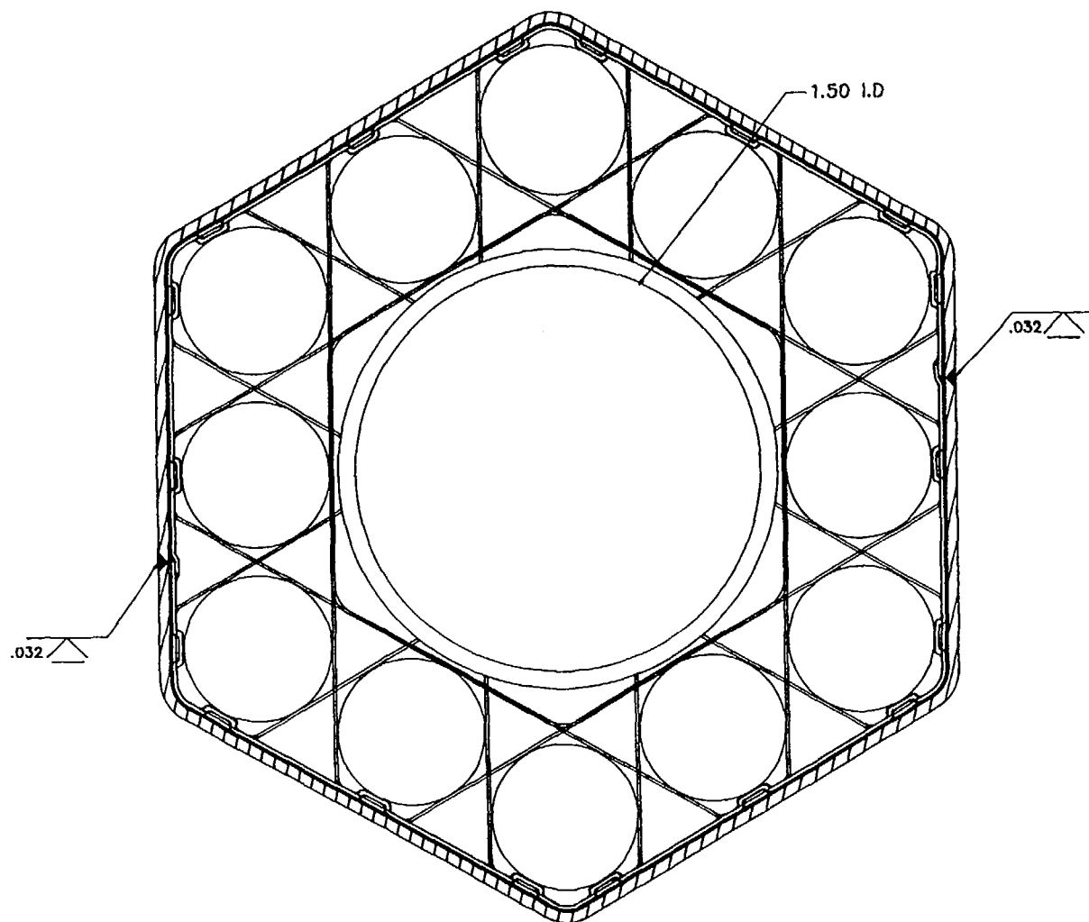
Figure 5. Hexagonal Control Rod Fuel Element
