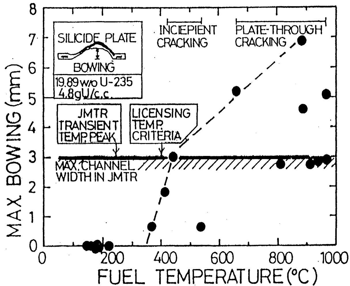
Fig. 7 Maximum Bowing of the Silicide Fuel Mini-plate as a Function of Fuel Temperature
