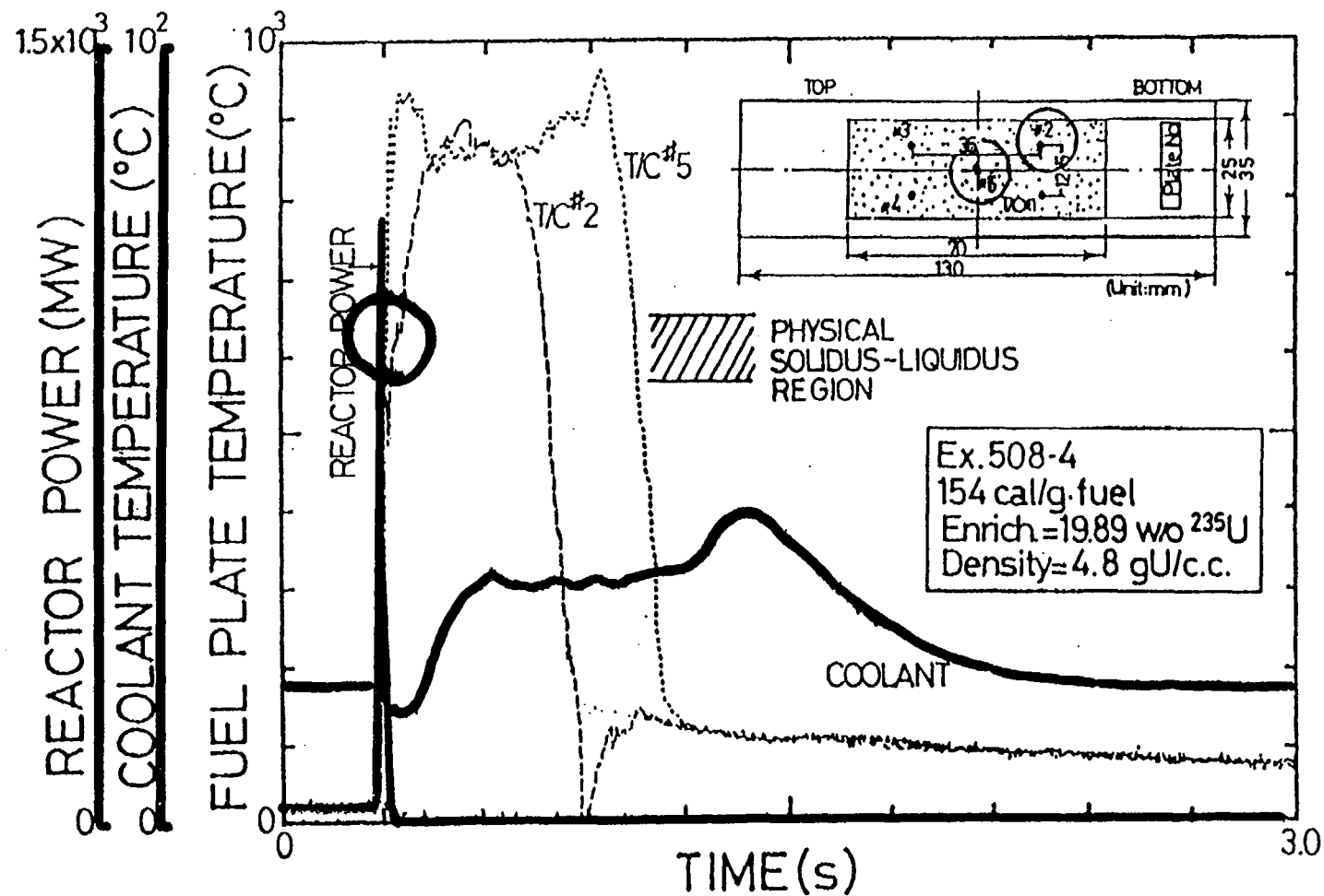
Fig. 3.4.2 Time-dependent change of the fuel plate surface temperatures measured by T/C's #2 and #5, that of coolant temperature and reactor power, where 19.89w/o enriched uranium silicide plate-type fuel having density by 4.8 \text{ gU/cm}^3 was used in experiment 508-4 (154 cal/g.fuel)
