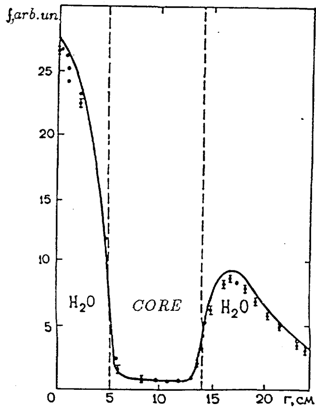
Fig.10: Fission rate as a function of the radius of the critical assembly. Full line: calculated values. Dotted: experiment
