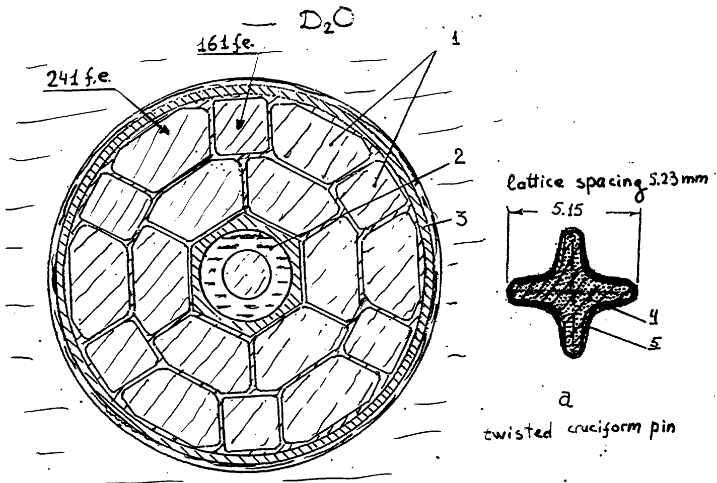
Fig. 5. Section the core of the PIK reactor.
