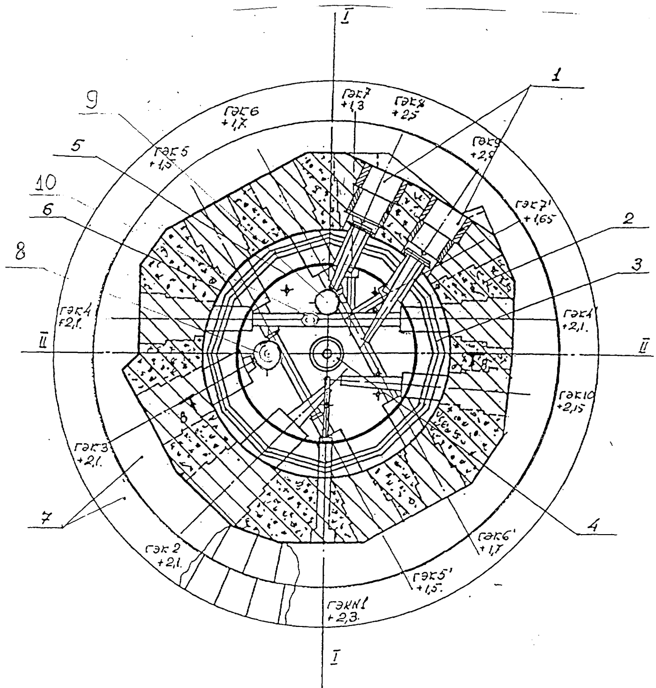
Fig.4: Layout of the experimental beams in the reflector of the PIK reactor.
