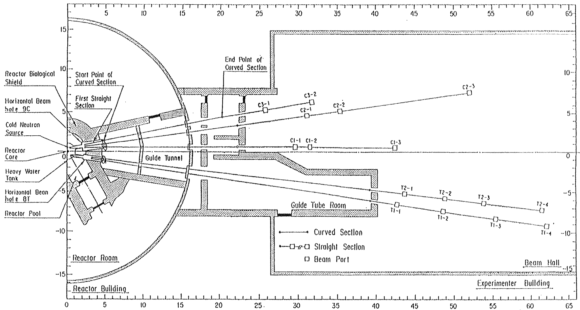
Fig. 3 Layout of the Neutron Guide Tubes in JRR-3M
