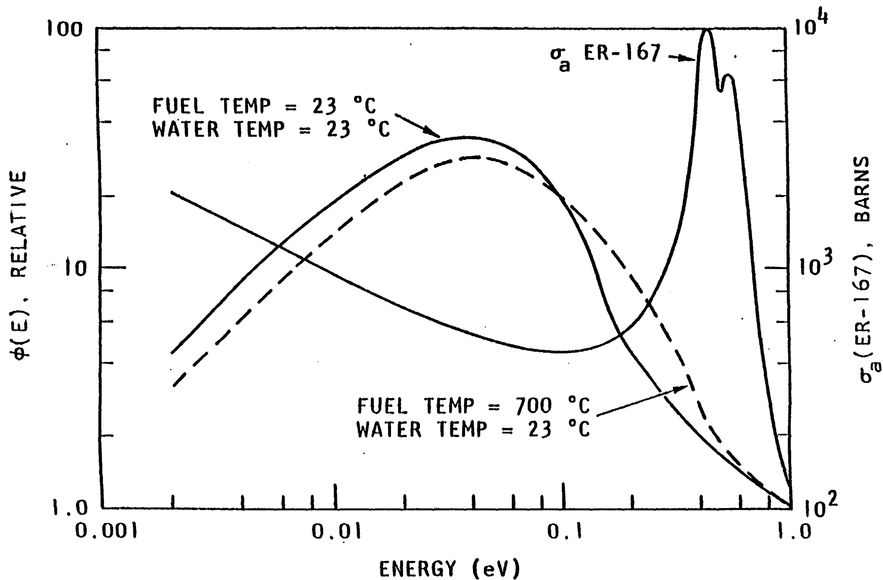
Figure 1. TRIGA Thermal Neutron Spectra vs. Fuel Temperature relative to \sigma_a vs. Energy for Er-167
