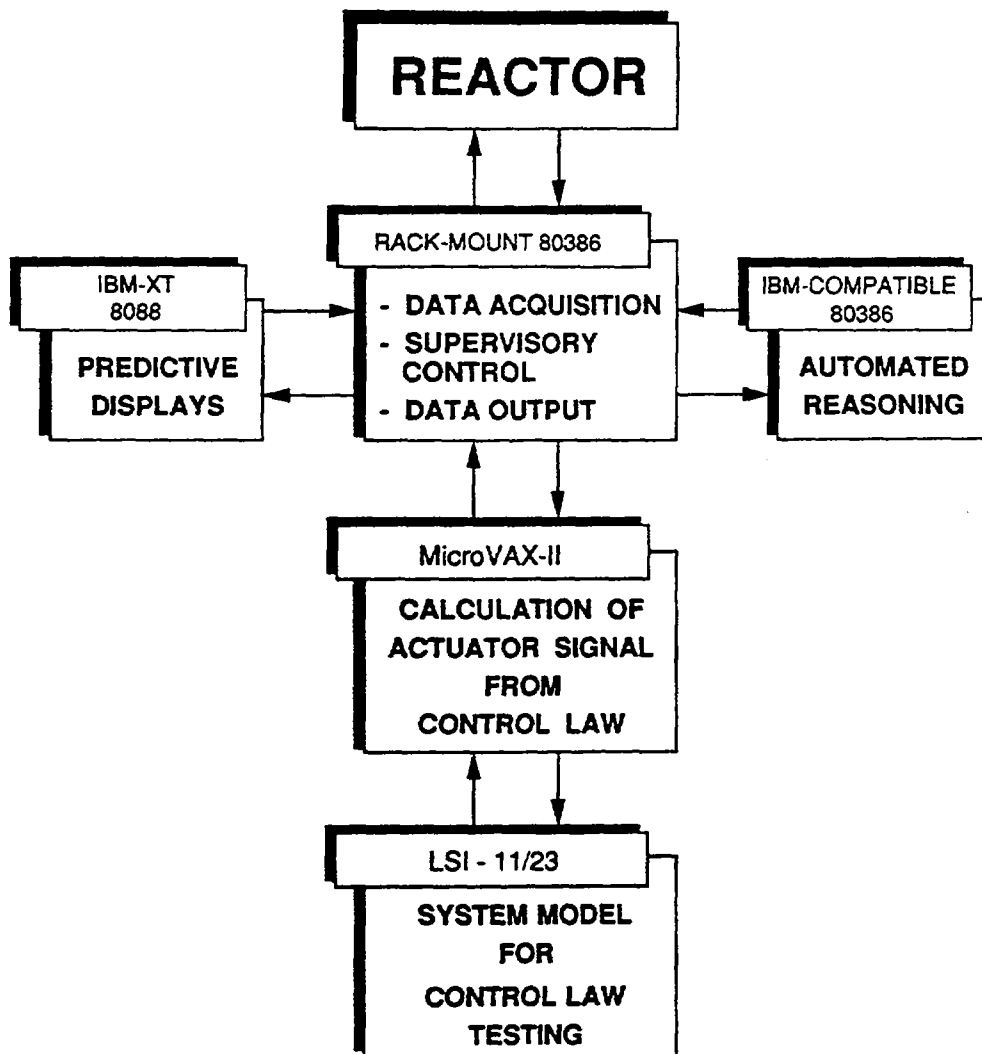
Figure 7. Configuration and Functions of MITR-II Advanced Control Computer System
