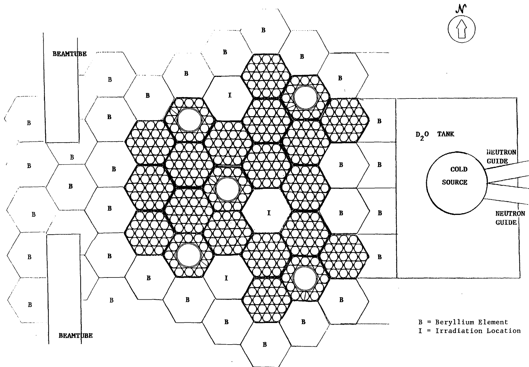
FIGURE 6. 10 MW CORE ARRANGEMENT USING HEXAGONAL FUEL ELEMENTS
