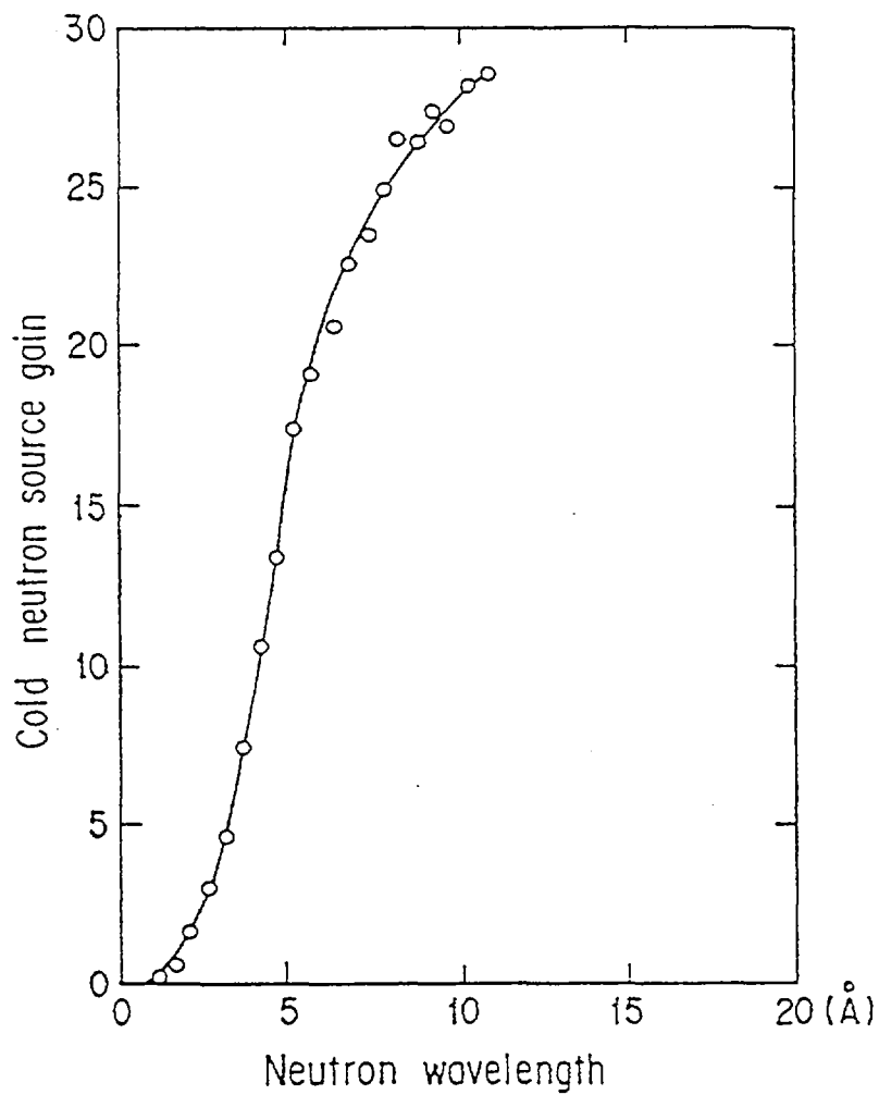
Fig. 5 The Cold Neutron Source Gain
