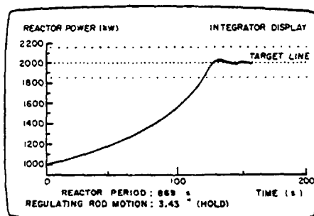
Figure 2. Current and Derivative Information (Scheme II)
