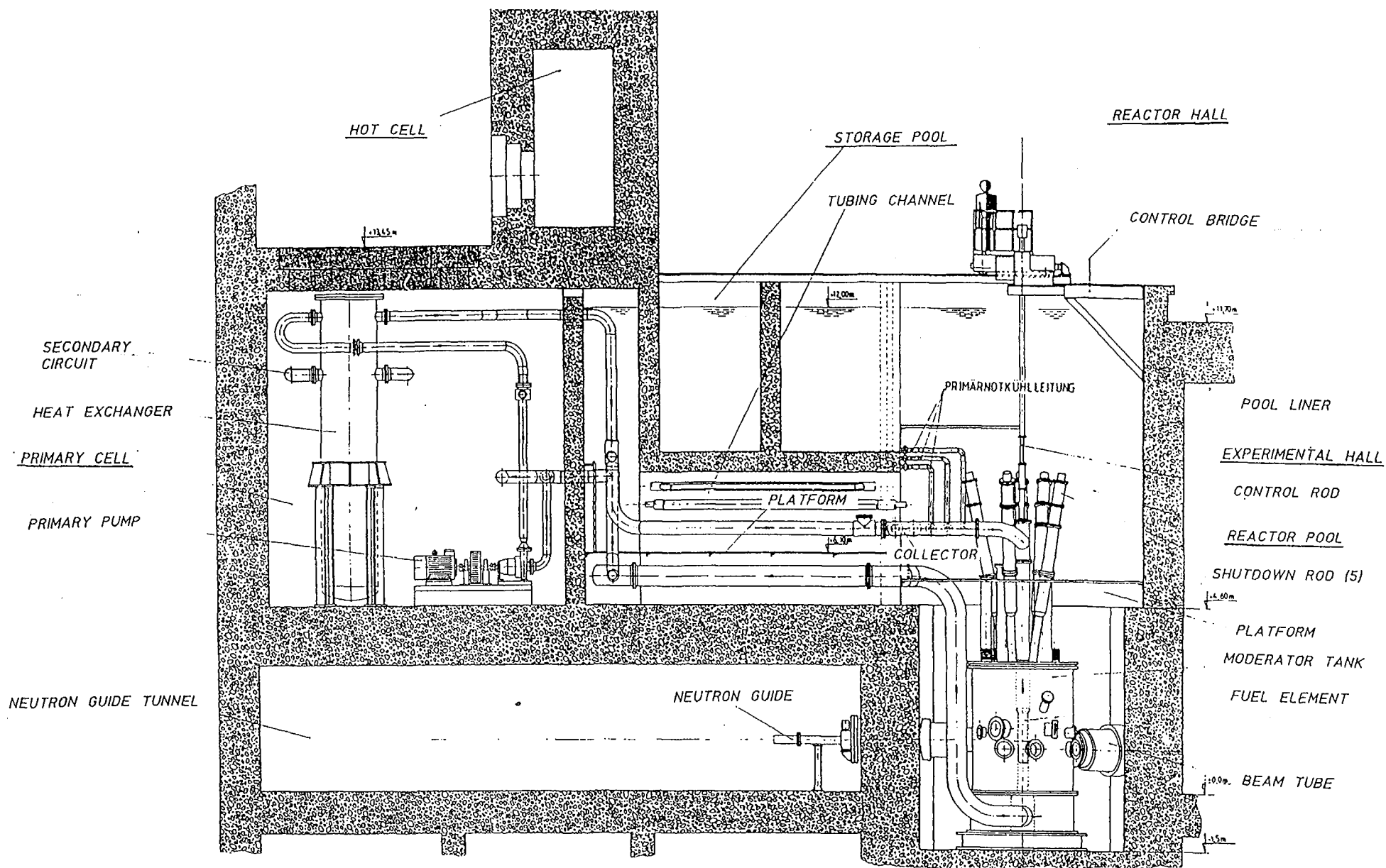
Fig. 2: Vertical cut through the reactor block showing the reactor pool, the storage pool, the tubing channel to the primary cells and the neutron guide tunnel.
