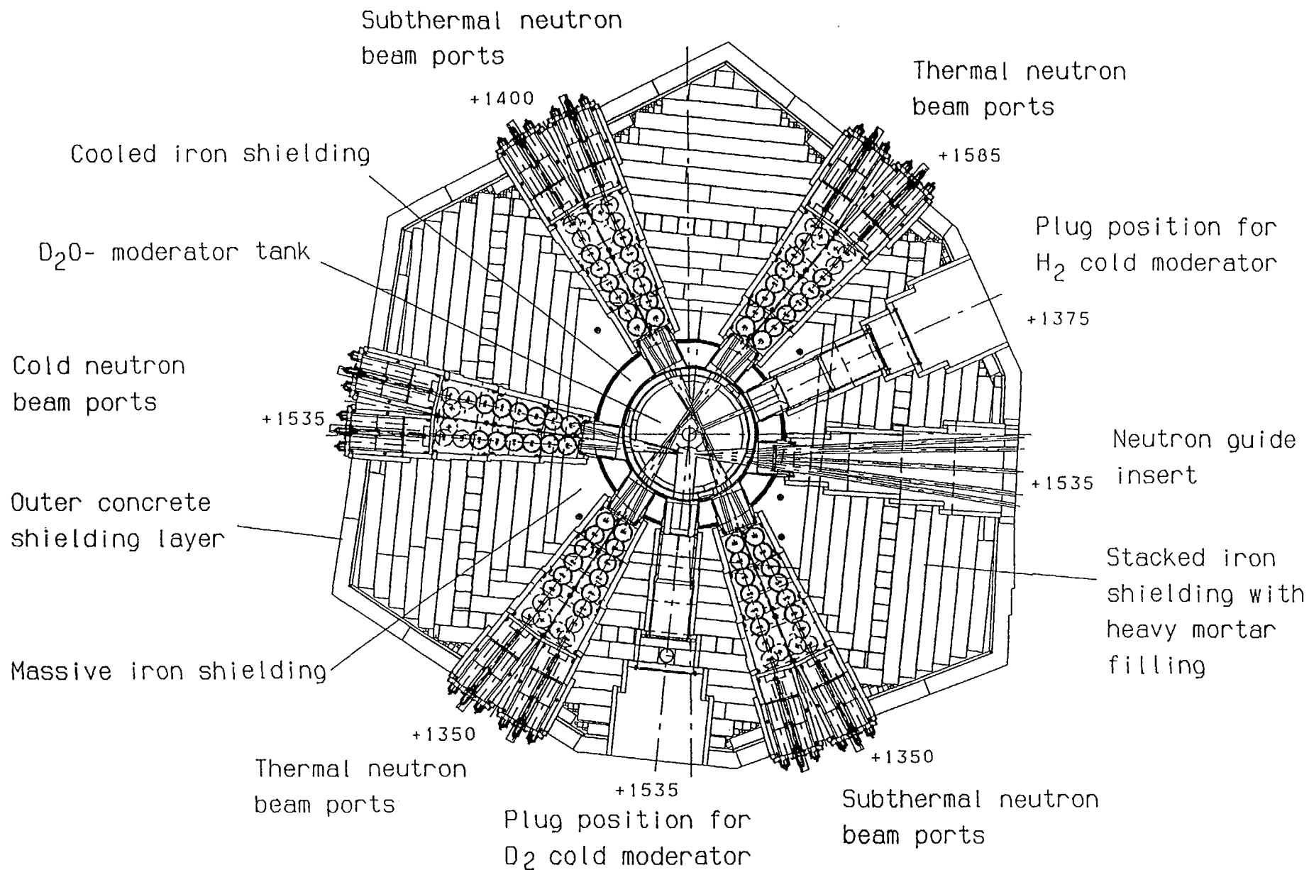
Fig.1 Horizontal section through the SINQ target block showing all horizontal penetrations, although actually on different levels. The height above the floor is indicated.
