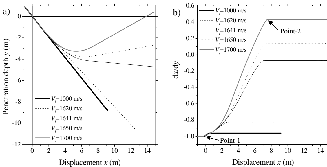
Fig.7 (a) Trajectories for projectile #2 and \phi_1=45^\circ , b) dx/dy of the trajectories from Fig.7(a)
